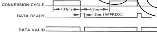
Figure 1. AD2033 Timing Diagram
