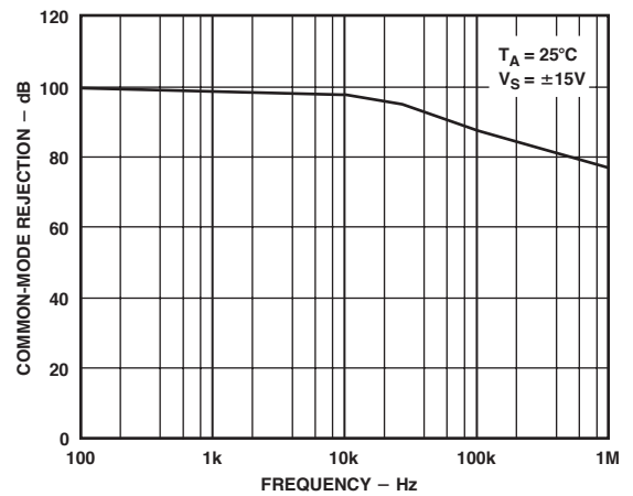
TPC 23. OP292/OP492 CMR vs. Frequency @ \pm 15\text{V}
