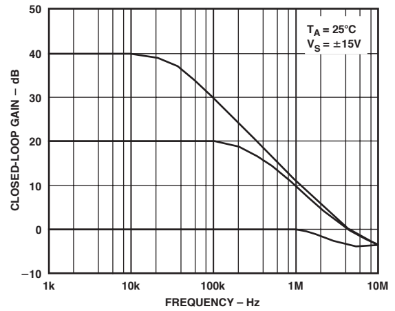
TPC 22. OP292/OP492 Closed-Loop Gain/Phase vs. Frequency @ \pm 15\text{V}
