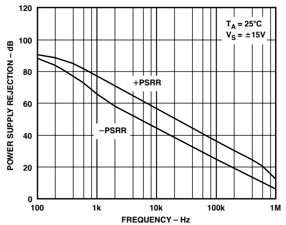
TPC 24. OP292/OP492 PSR vs. Frequency @ \pm 15\text{V}
