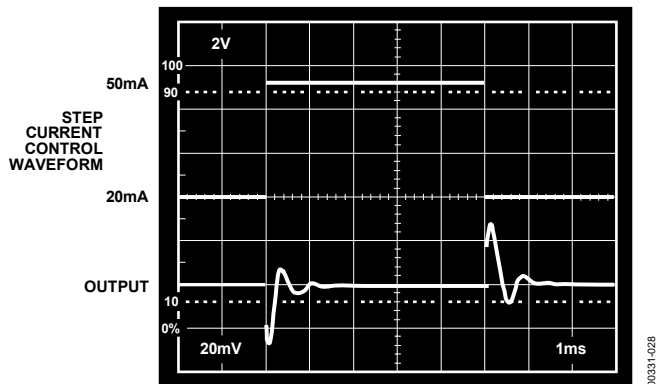
Figure 29. Output Step Load Current Recovery
