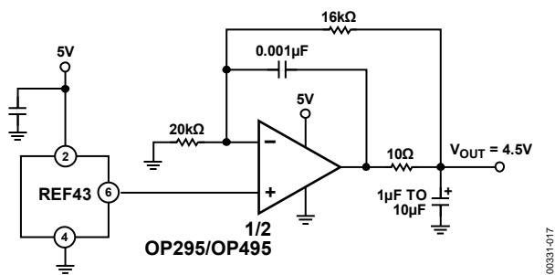
Figure 18. 4.5 V, Low Drop-Out Reference
