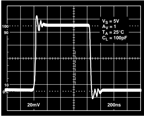
Figure 31. Small Signal Transient Response
