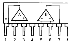
NJM072L/082L NJM072BL/082BL
