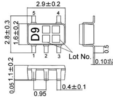
BU7481SG (SSOP5) (Unit : [mm])
