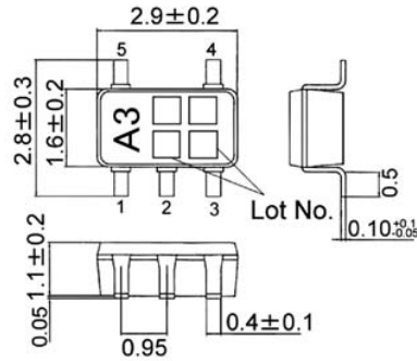
BU7481G (SSOP5) (Unit : [mm])
