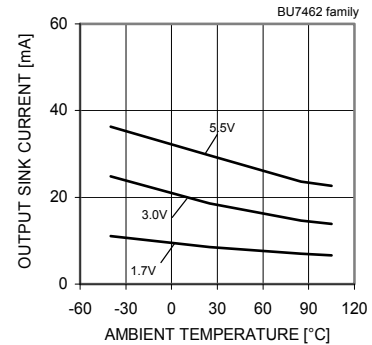
Fig.35 Output Sink Current – Ambient Temperature (VOUT=VSS+0.4[V])
