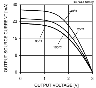
Fig.101 Output Source Current – Output Voltage ( V_{DD}=3[V] )
