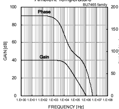
Fig.92 Gain – Frequency
