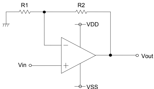
Fig.192 Non-inverting amplifier
