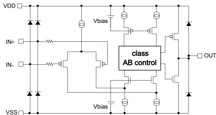
Fig.189 Schematic diagram
