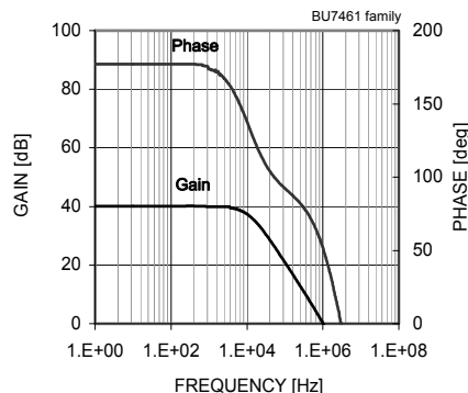
Fig.23 Gain – Frequency
