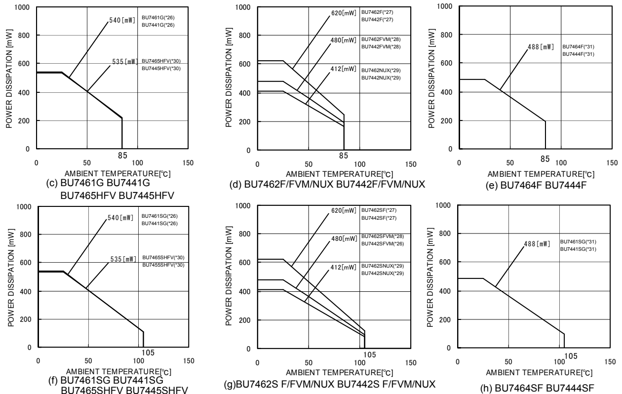
Fig.195 Thermal resistance and derating
