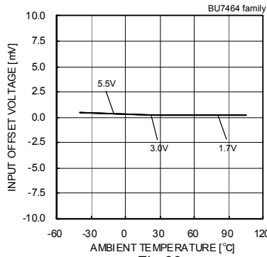
Fig. 60 Input Offset Voltage – Ambient Temperature (Vicm= VDD-1.2[V], VOUT= VDD/2)
