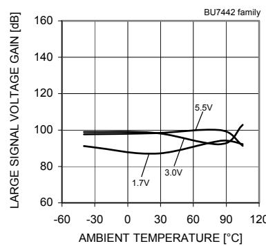
Fig. 132 Large Signal Voltage Gain – Ambient Temperature
