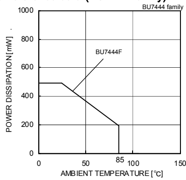
Fig. 139 Derating curve
