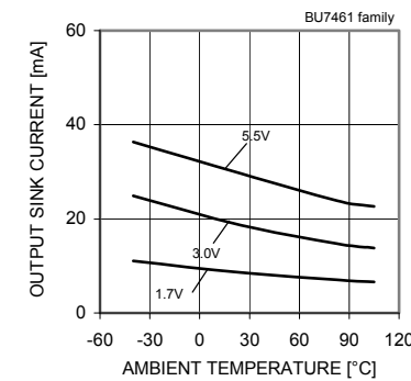
Fig.12 Output Sink Current – Ambient Temperature (VOUT=VSS+0.4[V])
