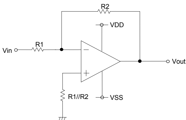
Fig.191 Inverting amplifier
