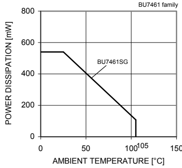
Fig.2 Derating curve
