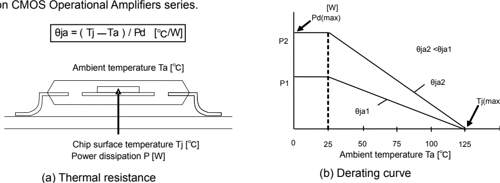
Fig.195 Thermal resistance and derating
