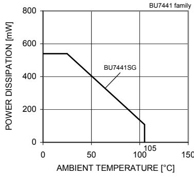
Fig.94 Derating curve
