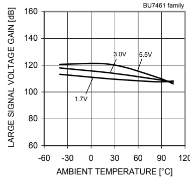
Fig.17 Power Supply Rejection Ratio – Ambient Temperature
