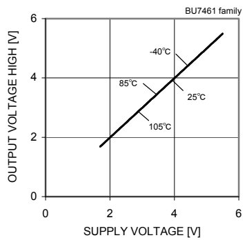
Fig.5 Output Voltage High – Supply Voltage (RL=10[kΩ])
