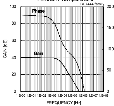
Fig.161 Gain – Frequency
