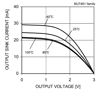
Fig.9 Output Source Current – Output Voltage (VDD=3.0[V])
