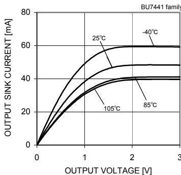
Fig.103 Output Sink Current – Output Voltage ( V_{DD}=3[V] )
