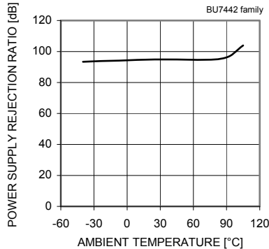
Fig. 135 Power Supply Rejection Ratio – Ambient Temperature
