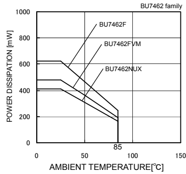
Fig.24 Derating curve
