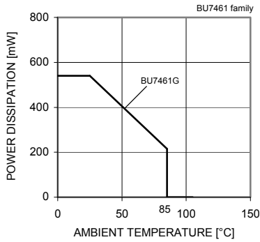
Fig.1 Derating curve
