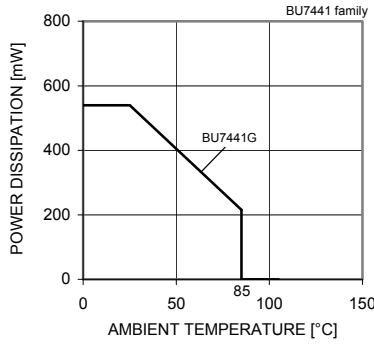
Fig.93 Derating curve
