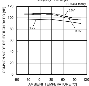
Fig. 65 Common Mode Rejection Ratio – Ambient Temperature
