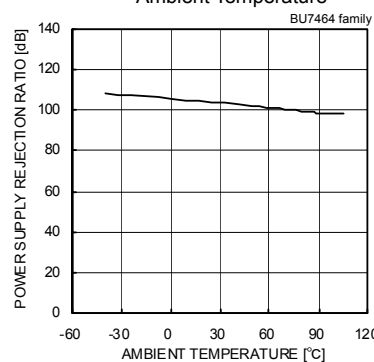
Fig. 66 Power Supply Rejection Ratio – Ambient Temperature
