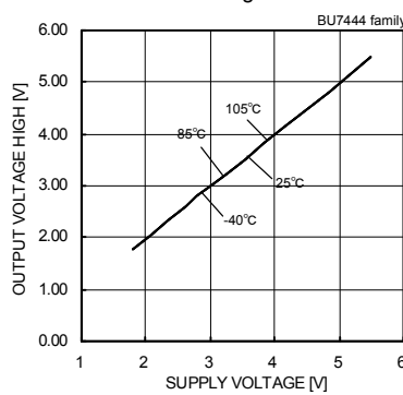
Fig. 143 Output Voltage High - Supply Voltage (RL=10[kΩ])
