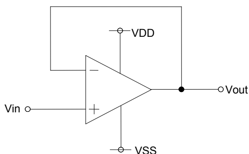
Fig.190 Voltage follower
