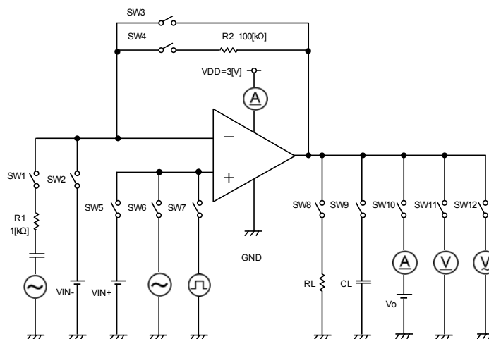
Fig.186 Test circuit 2
