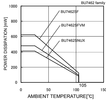
Fig.25 Derating curve
