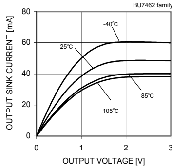
Fig.34 Output Sink Current – Output Voltage (VDD=3[V])
