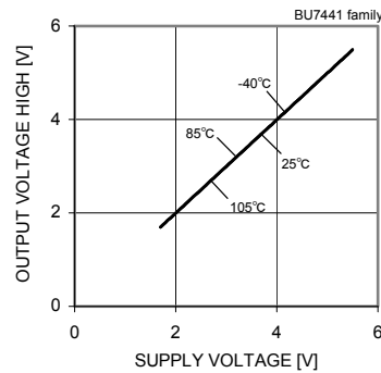
Fig.97 Output Voltage High – Supply Voltage ( R_L=10[k\Omega] )
