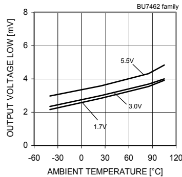
Fig.31 Output Voltage Low – Ambient Temperature (RL=10[kΩ])
