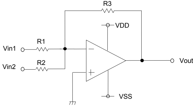
Fig.193 Adder circuit
