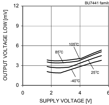
Fig.99 Output Voltage Low – Supply Voltage ( R_L=10[k\Omega] )
