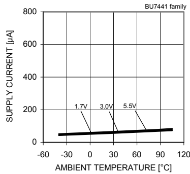
Fig.96 Supply Current – Ambient Temperature
