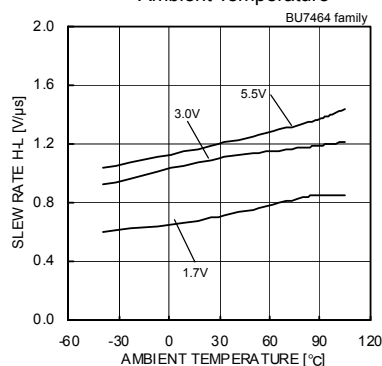
Fig. 68 Slew Rate H-L – Ambient Temperature
