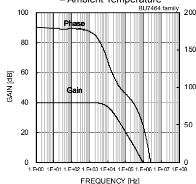
Fig. 69 Gain – Frequency
