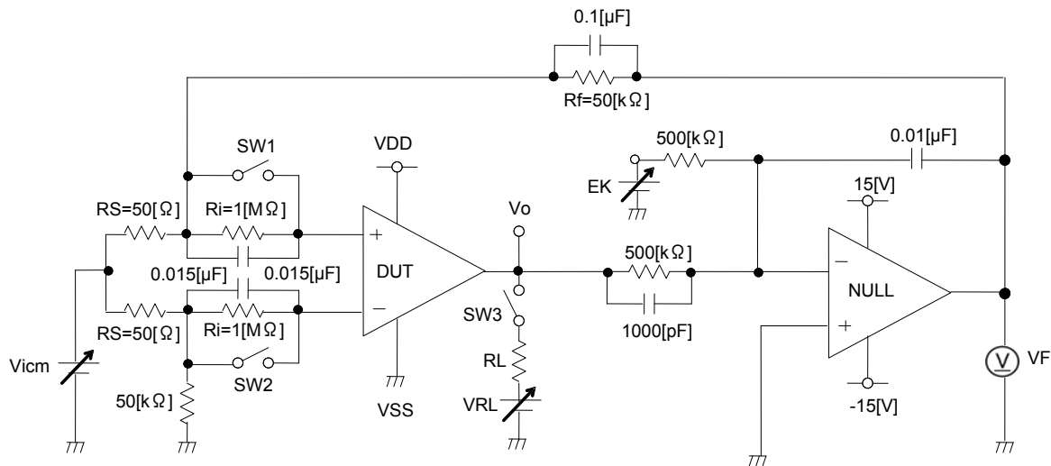
Fig. 185 Test circuit 1 (one channel only)
