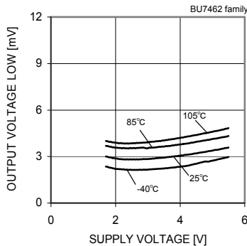
Fig.30 Output Voltage Low – Supply Voltage (RL=10[kΩ])
