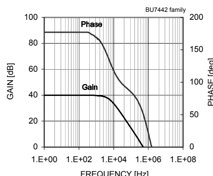
Fig. 138 Gain – Frequency
