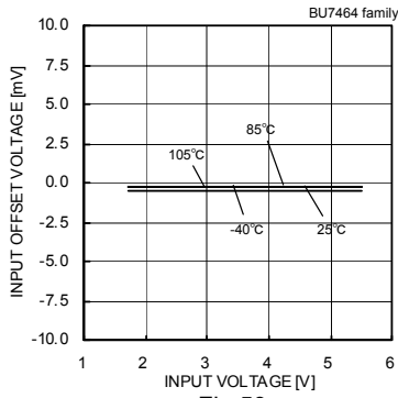
Fig. 59 Input Offset Voltage – Supply Voltage (Vicm= VDD-1.2[V], VOUT= VDD/2)
