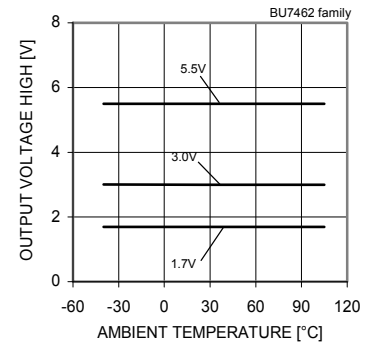
Fig.29 Output Voltage High – Ambient Temperature (RL=10[kΩ])
