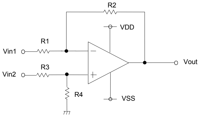
Fig.194 Differential amplifier
