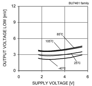
Fig.7 Output Voltage Low – Supply Voltage (RL=10[kΩ])
