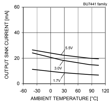
Fig.104 Output Sink Current – Ambient Temperature ( V_{OUT}=V_{SS}+0.4[V] )
