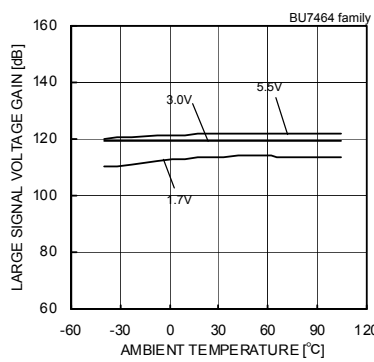
Fig. 63 Large Signal Voltage Gain – Ambient Temperature
