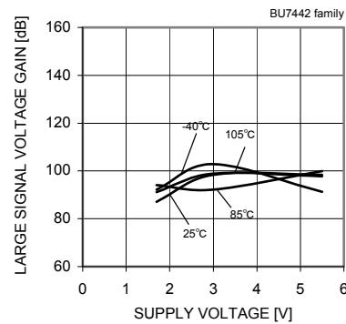
Fig. 131 Large Signal Voltage Gain – Supply Voltage
