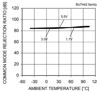
Fig. 134 Common Mode Rejection Ratio – Ambient Temperature
