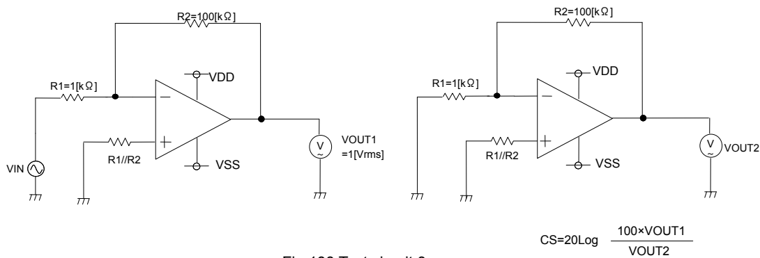
Fig.188 Test circuit 3
