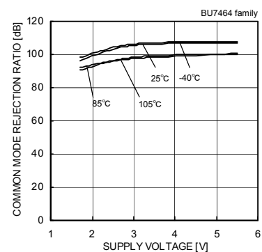
Fig. 64 Common Mode Rejection Ratio – Supply Voltage
