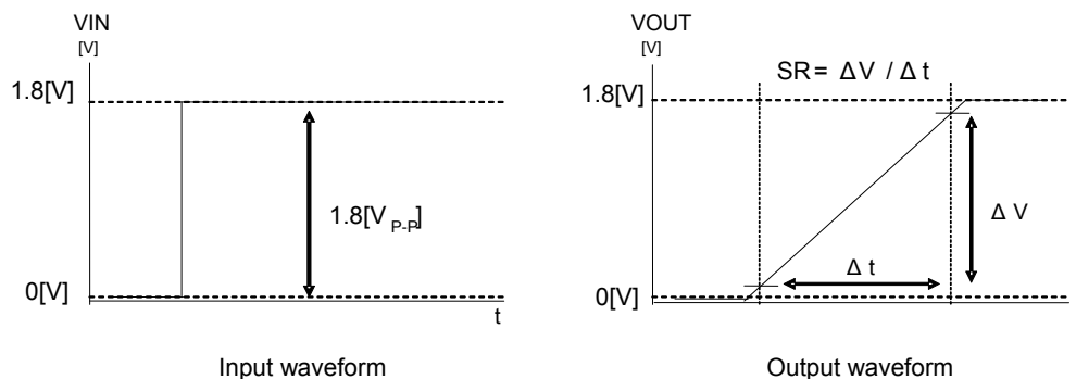
Fig.187 Slew rate input output wave
