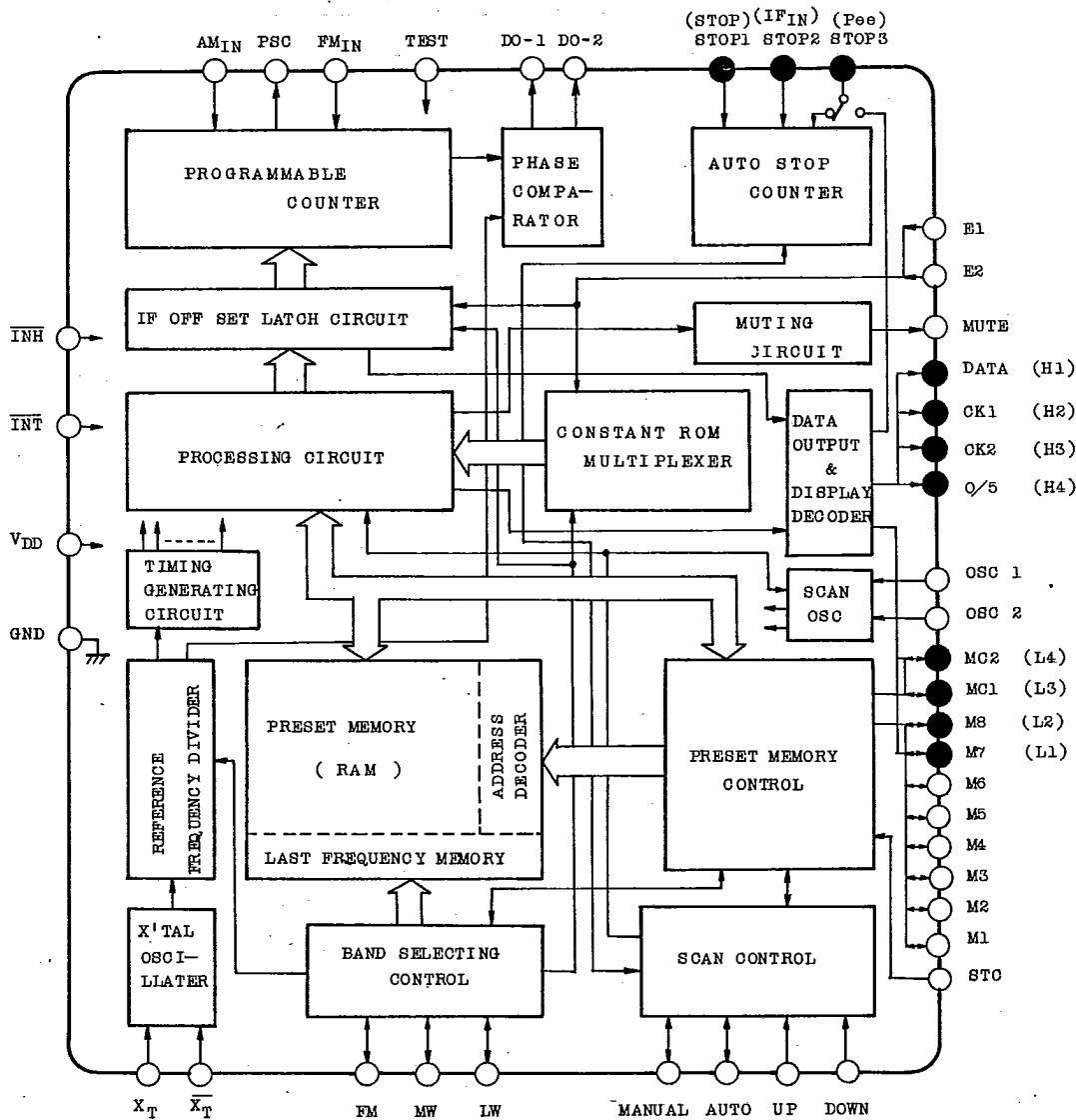
BLOCK DIAGRAM
