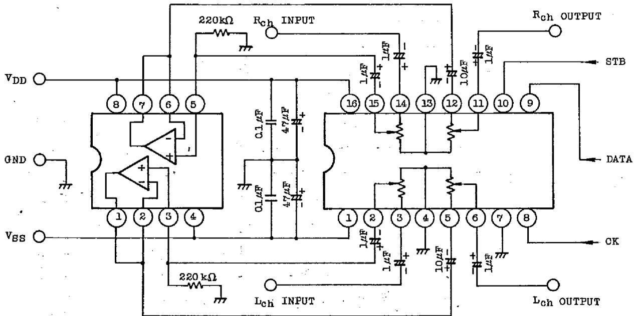
TC9176P APPLICATION CIRCUIT EXAMPLE
