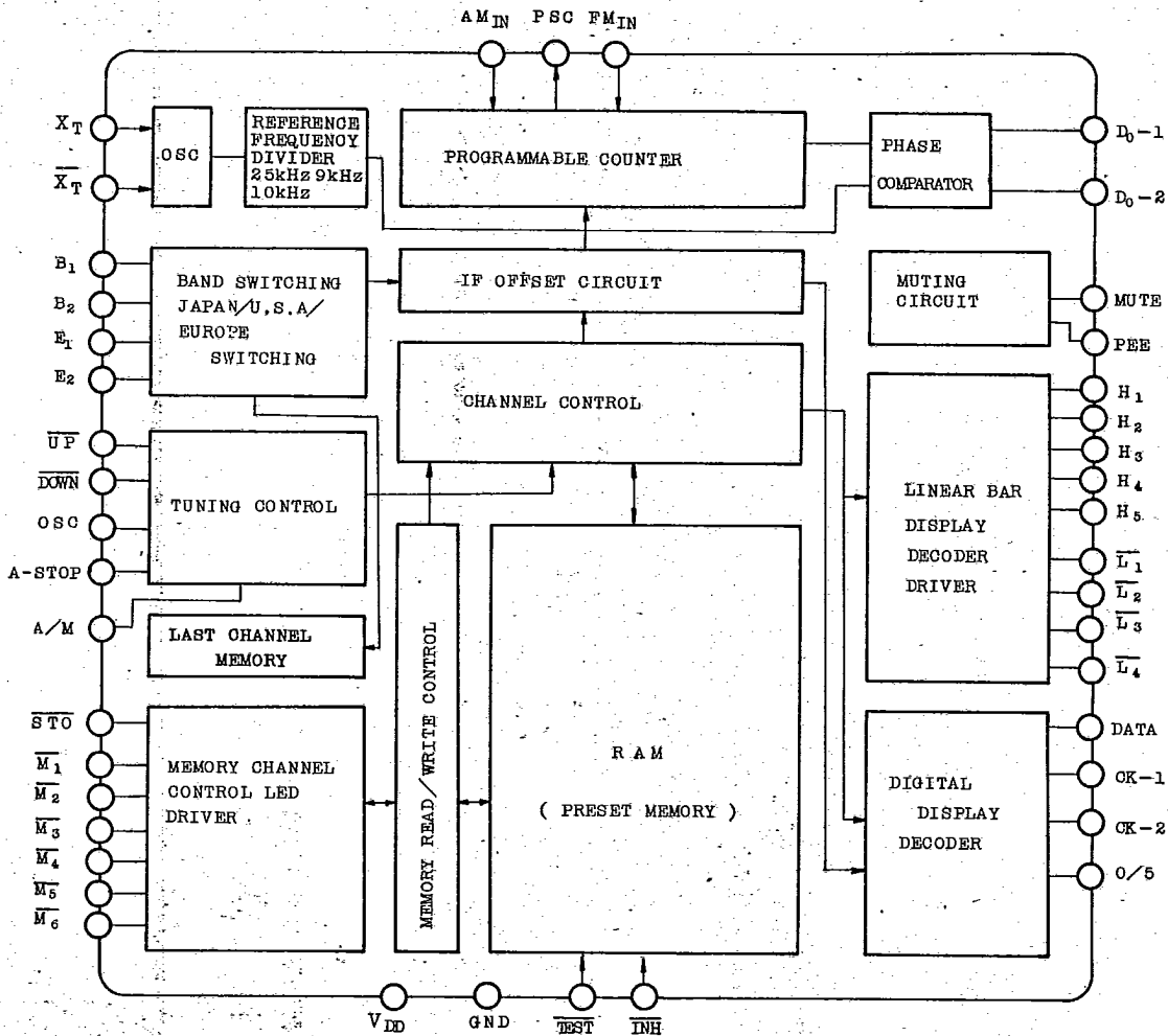
BLOCK DIAGRAM
