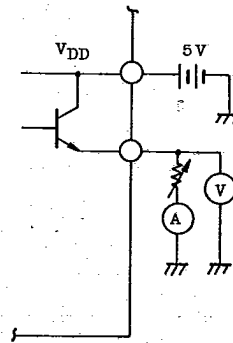
TEST CIRCUIT
