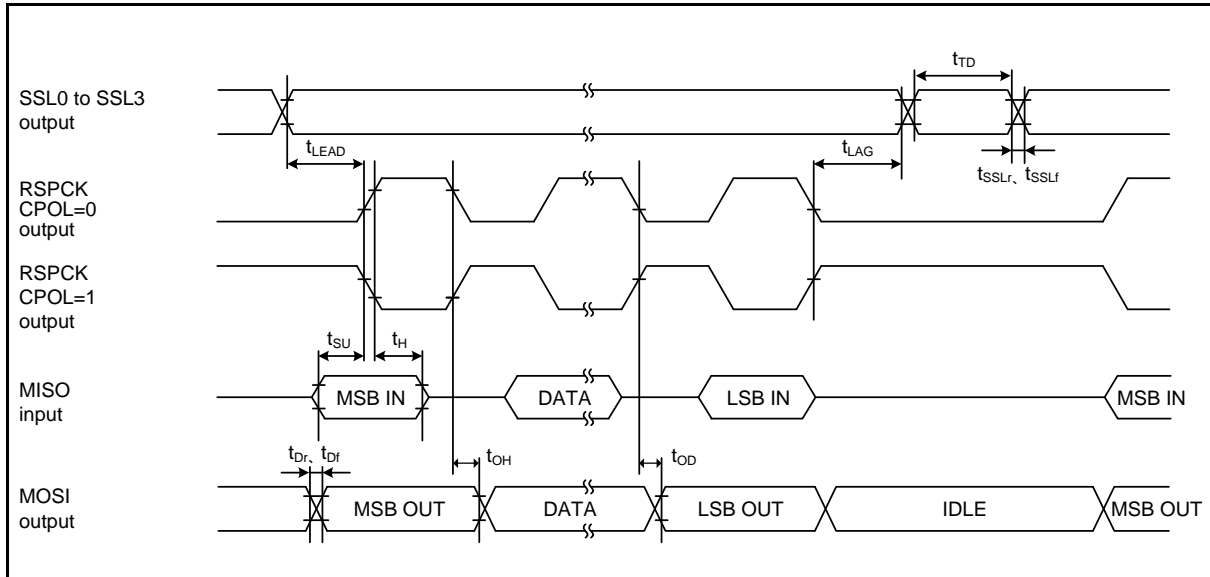
Figure 5.12 RSPCK Timing (Master, CPHA = 0)
