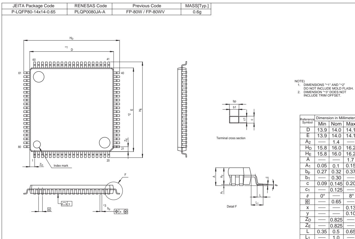
Figure C 80-Pin LQFP (PLQP0080JA-A) Package Dimensions
