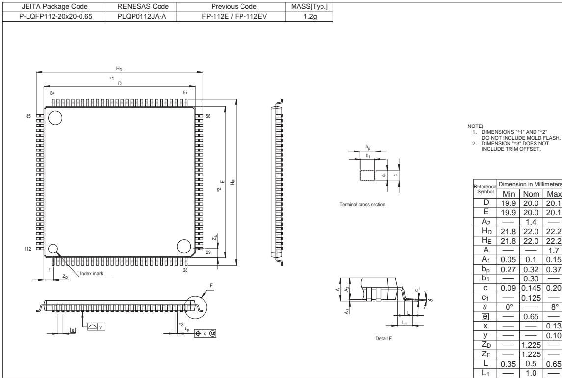
Figure A 112-Pin LQFP (PLQP0112JA-A) Package Dimensions
