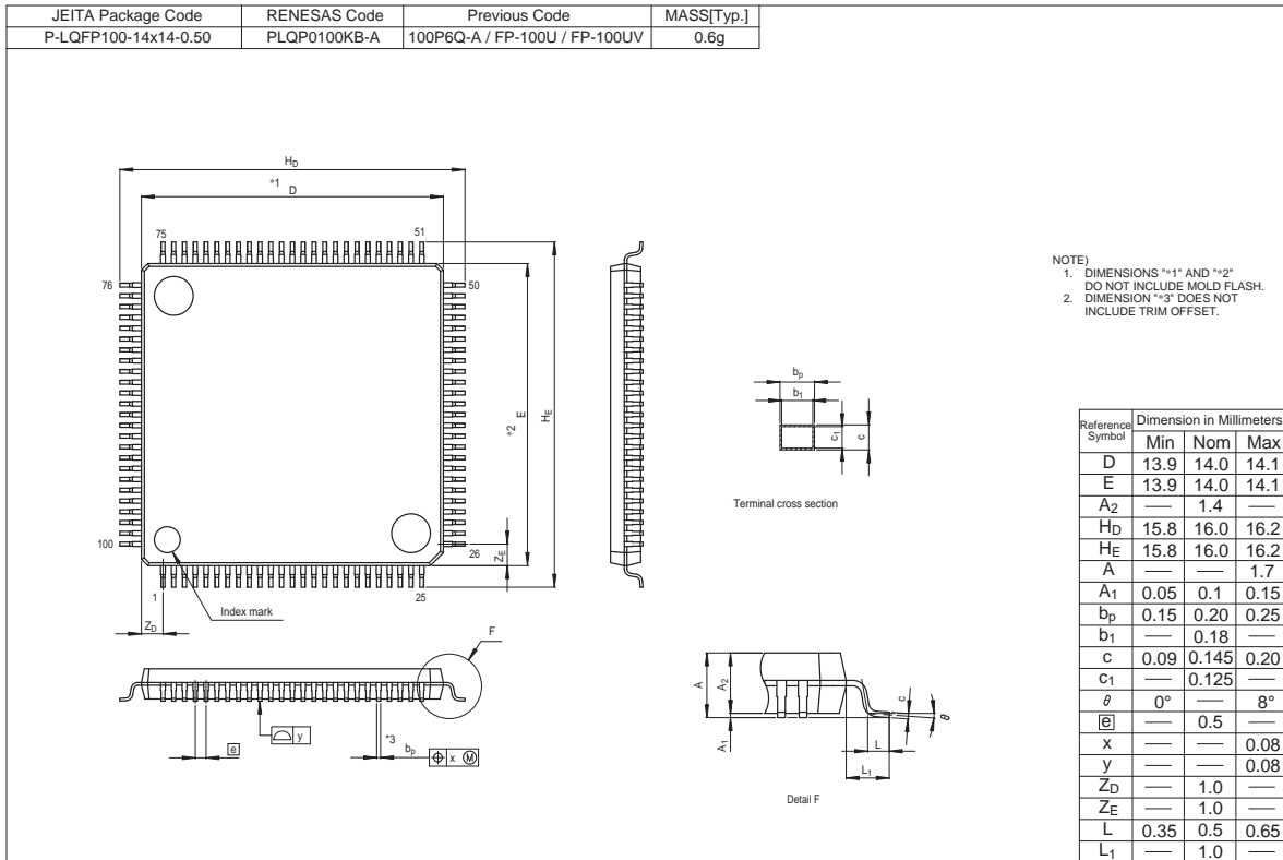
Figure B 100-Pin LQFP (PLQP0100KB-A) Package Dimensions
