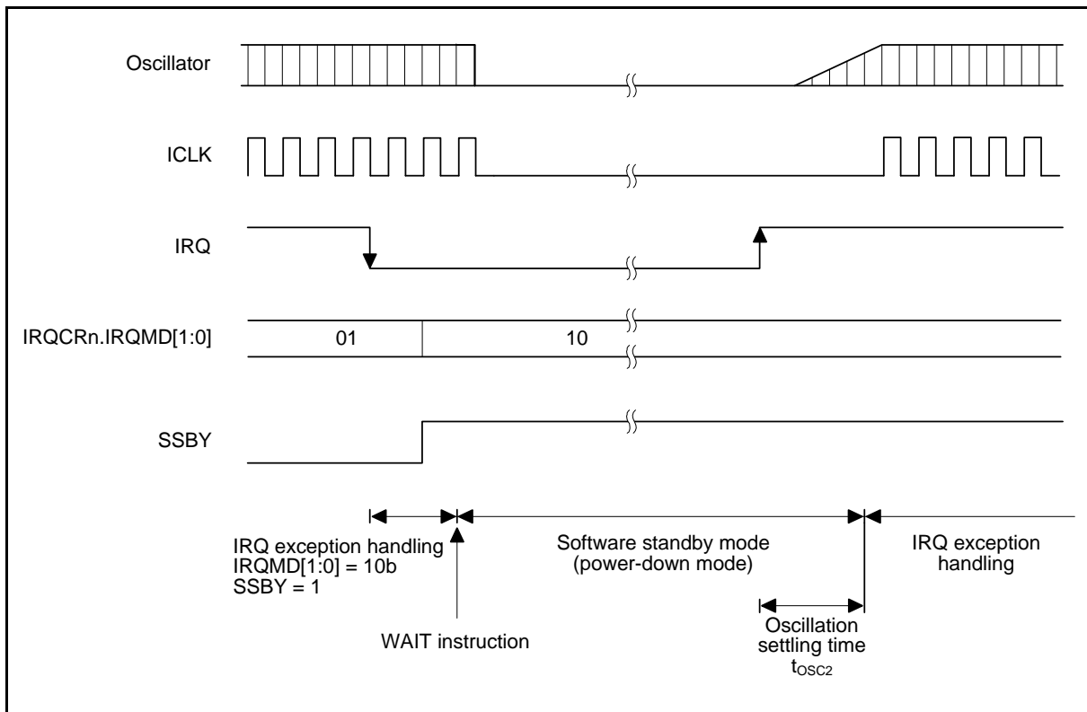
Figure 5.2 Oscillation Settling Timing after Software Standby Mode
