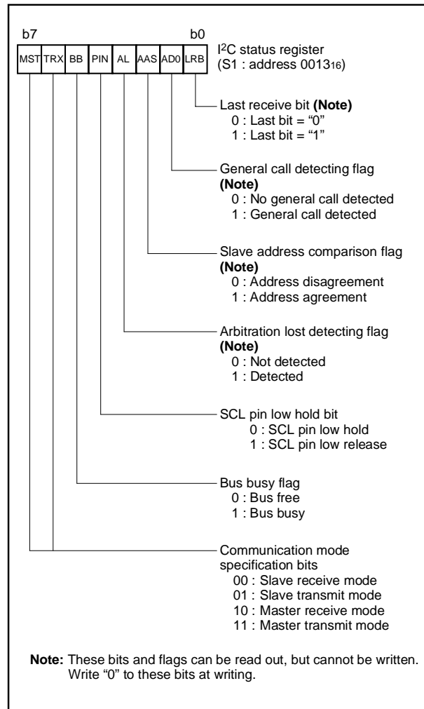
Fig. 68 Structure of I²C status register
