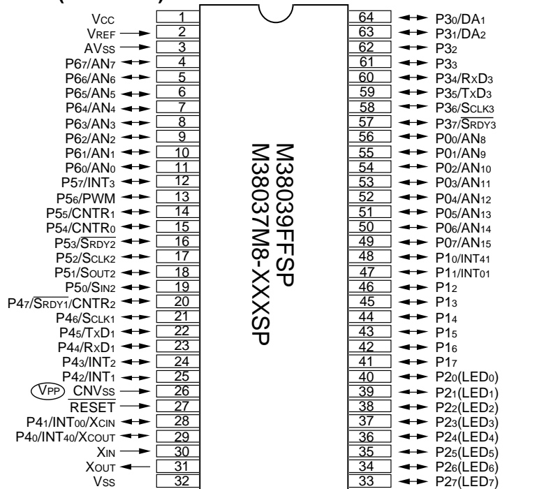
Fig. 2 3803 group pin configuration
