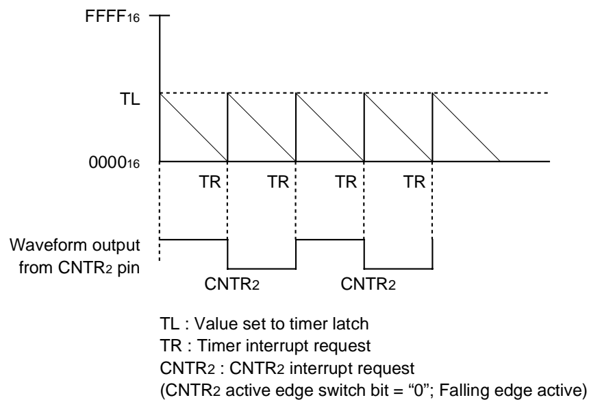
Fig. 35 Timing chart of pulse output mode
