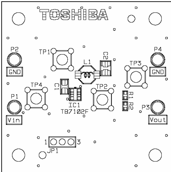
Component side silk
