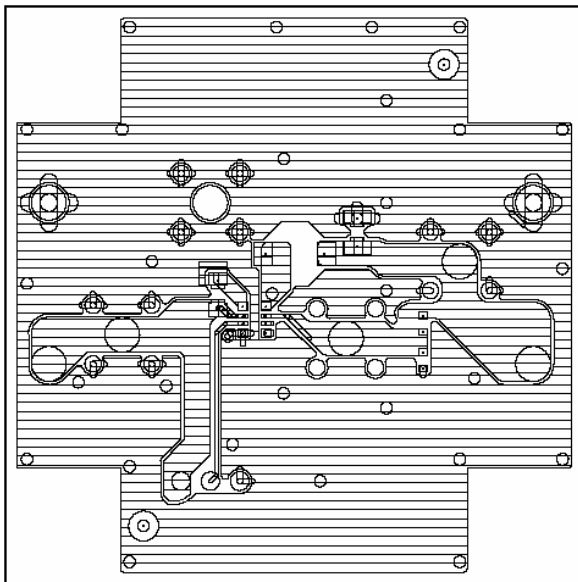
Component side pattern
