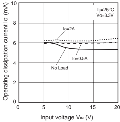
Fig.10 Operating Dissipation Current vs. Input Voltage
