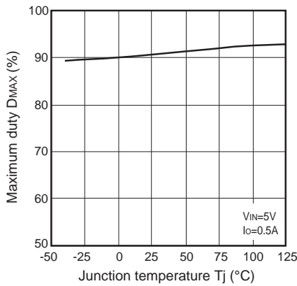
Fig.14 Maximum Duty vs. Junction Temperature
