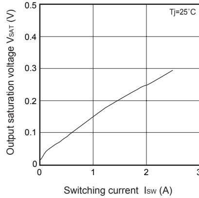
Fig.5 Output Saturation Voltage vs. Switching Current
