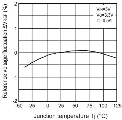
Fig.6 Reference Voltage Fluctuation vs. Junction Temperature
