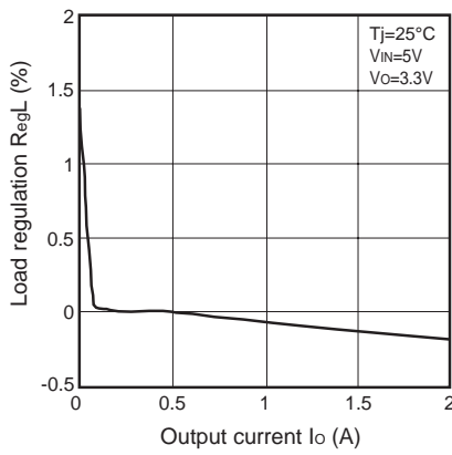
Fig.12 Load Regulation vs. Output Current
