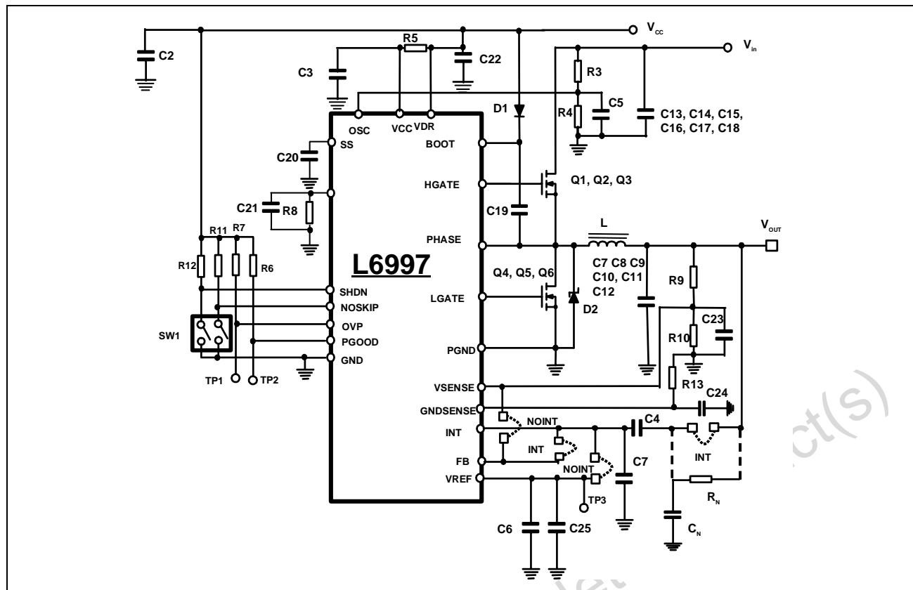
Figure 17. Schematic diagram
