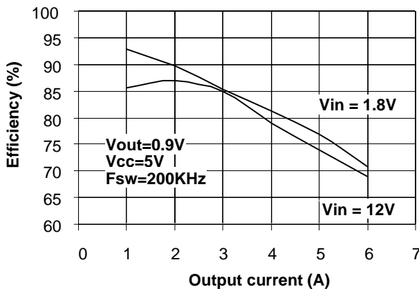
Figure 29. Eff. vs Output Current sink mode
