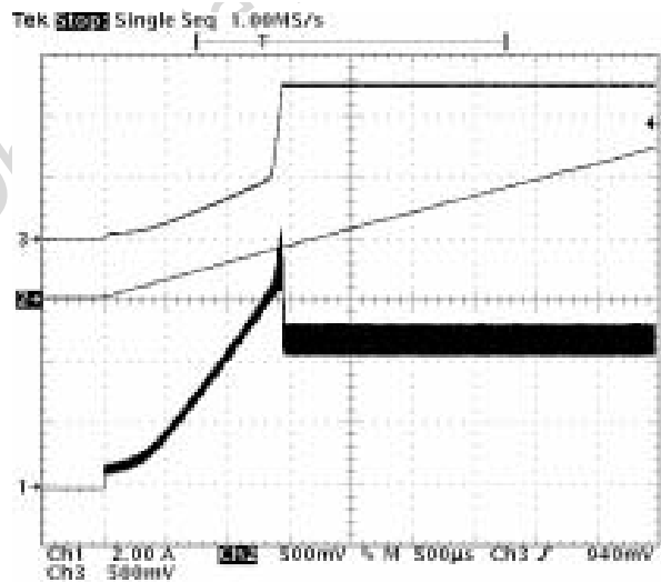
Figure 35. Start up waveform with 5A load..
