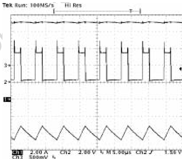
Figure 31. Normal functionality in SINK mode..
