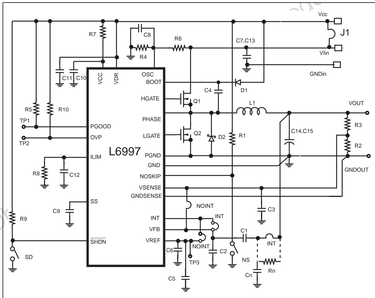
Figure 10. Demoboard Schematic Diagram
