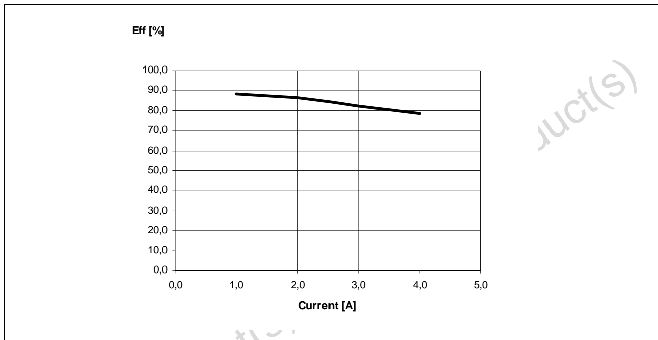
Figure 16. Efficiency vs output current
