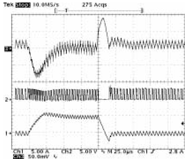
Figure 30. Load transient response from 0A to 5A..
