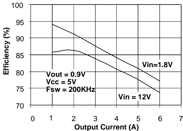
Figure 28. Eff. vs. Output Current Source Mode
