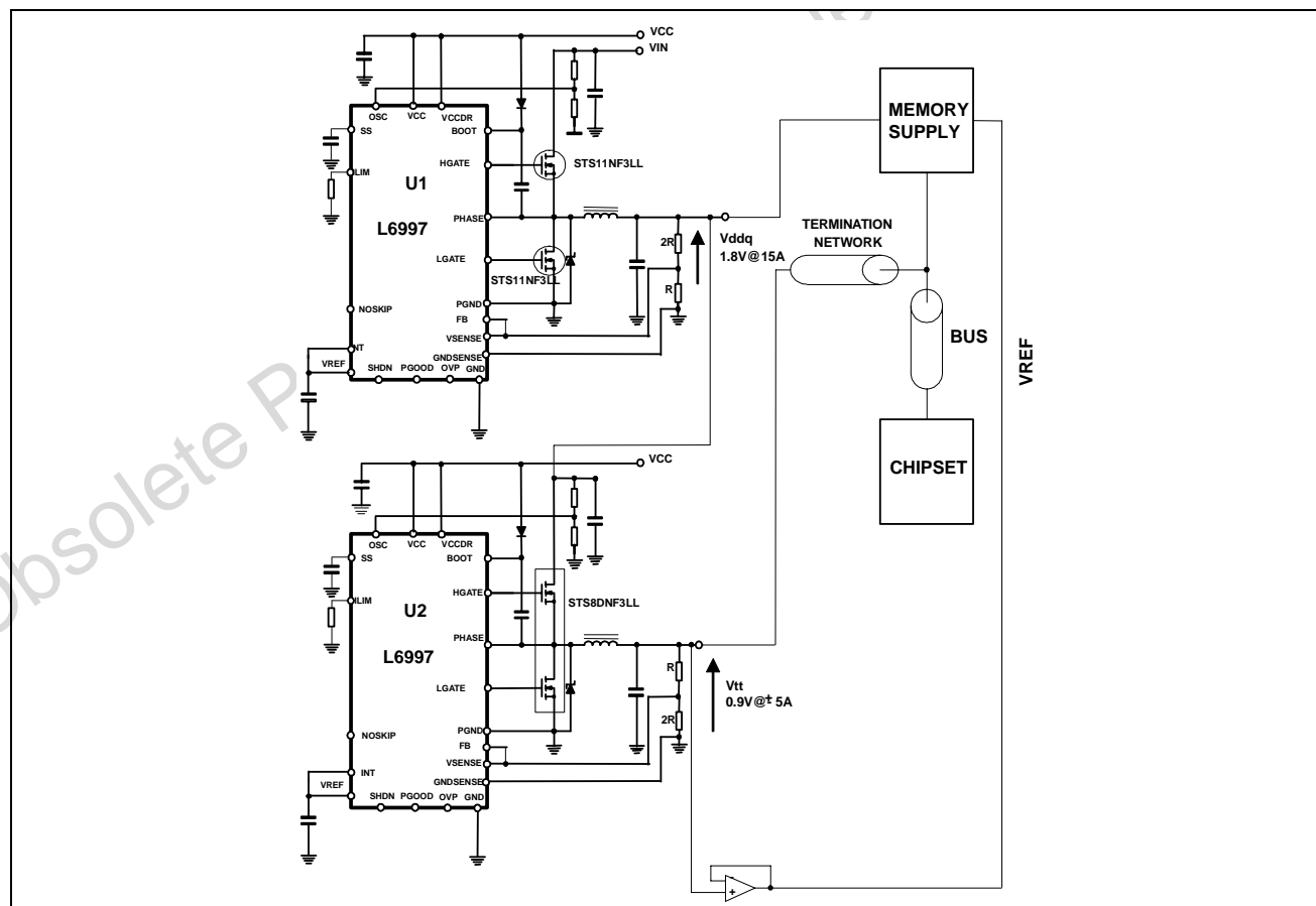
Figure 27. Application Idea: DDRII Memory Supply
