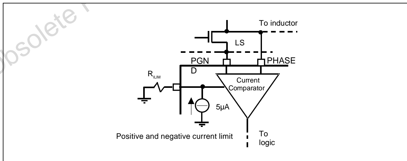
Figure 9. Current limit schematic
