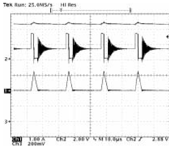
Figure 33. Normal functionality in PFM mode.
