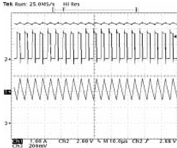
Figure 32. Normal functionality in PWM mode.
