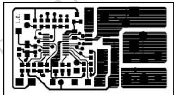
Figure 13. Top side layout
