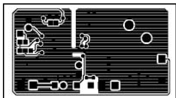
Figure 14. Bottom side layout
