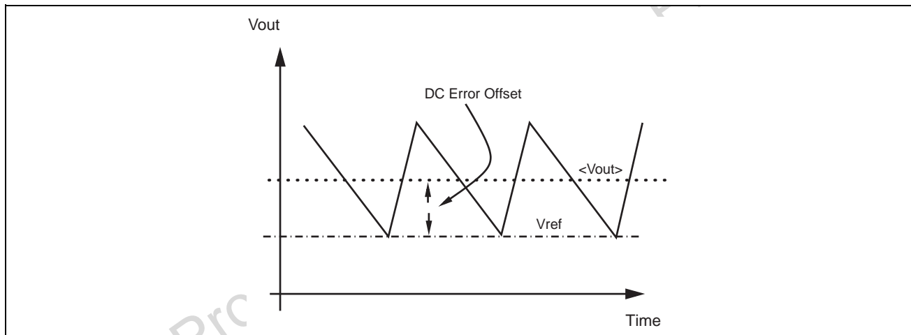
Figure 6. Valley regulation
