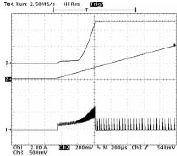
Figure 34. Start up waveform with 0A load.
