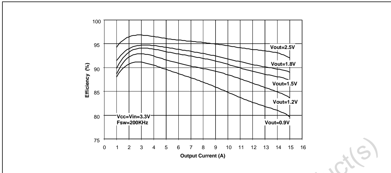
Figure 22. Efficiency vs output Current
