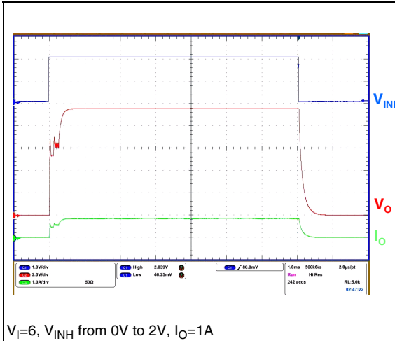
Figure 30. INH transient
