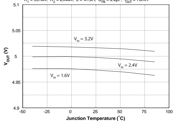
Temperature Reg. — PWM Mode ( V_{OUT} = 5.0V )
