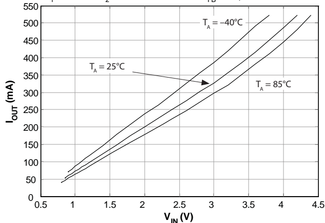
Max. I_{OUT} vs. V_{IN} ( V_{OUT} = 5.0V , all V_{IN} Ranges)
