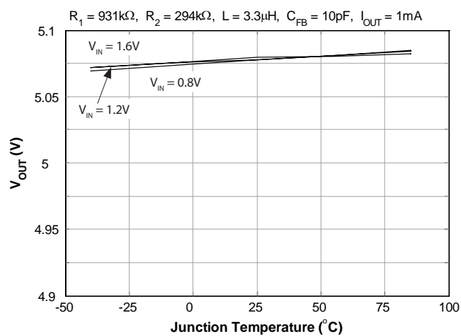
Temperature Reg. — PSAVE Mode ( V_{OUT} = 5.0V )
