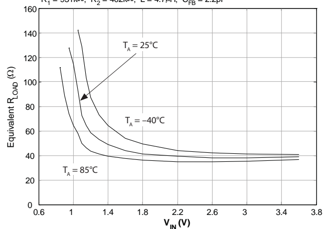
Startup Min. Load Resistance vs. V_{IN} ( V_{OUT} = 4.0V )
