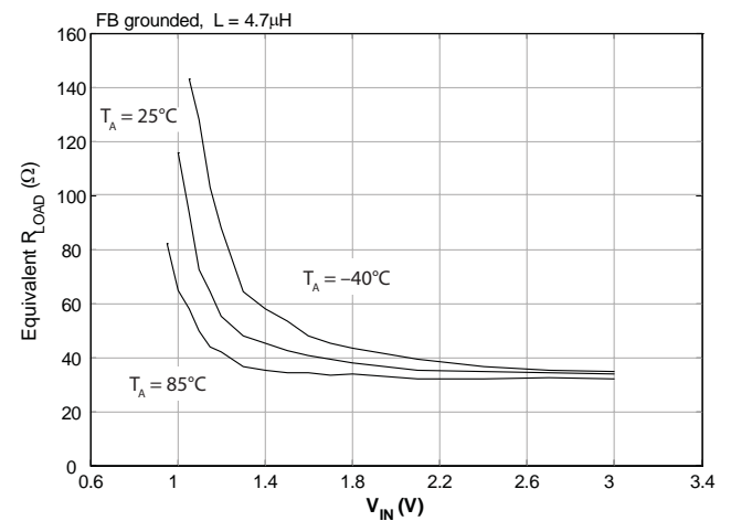
Startup Min. Load Resistance vs. V_{IN} ( V_{OUT} = 3.3V )
