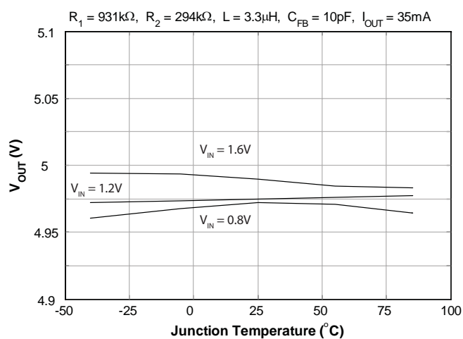
Temperature Reg. — PWM Mode ( V_{OUT} = 5.0V )
