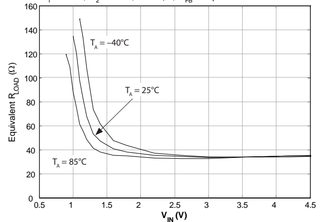
Startup Min Load Res. vs. V_{IN} ( V_{OUT} = 5.0V , all V_{IN} Ranges)
