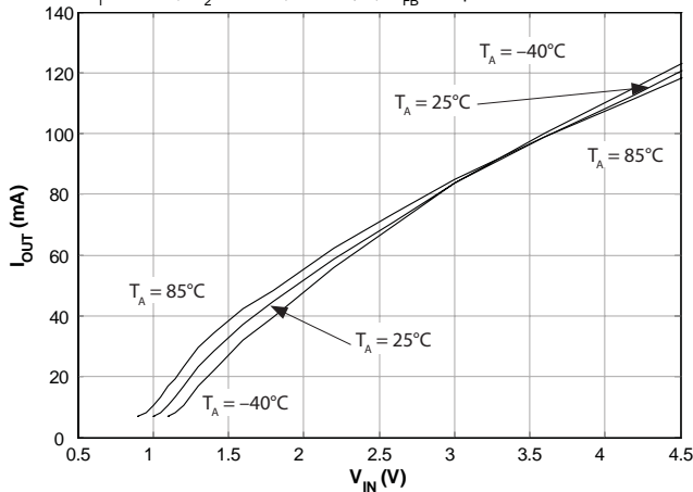
Startup Max Load Current vs. V_{IN} ( V_{OUT} = 5.0V , all V_{IN} 's)
