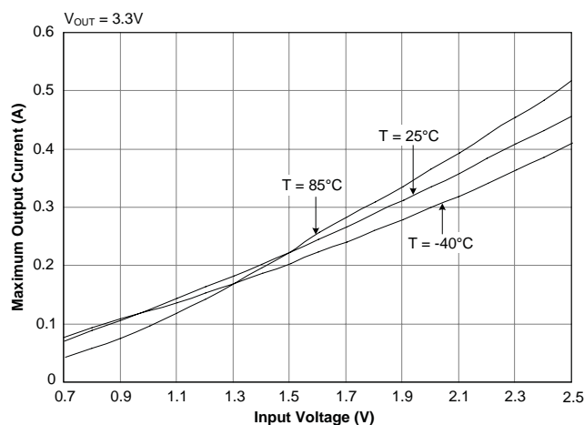
Max. I_{OUT} vs. V_{IN} ( V_{OUT} = 3.3V )
