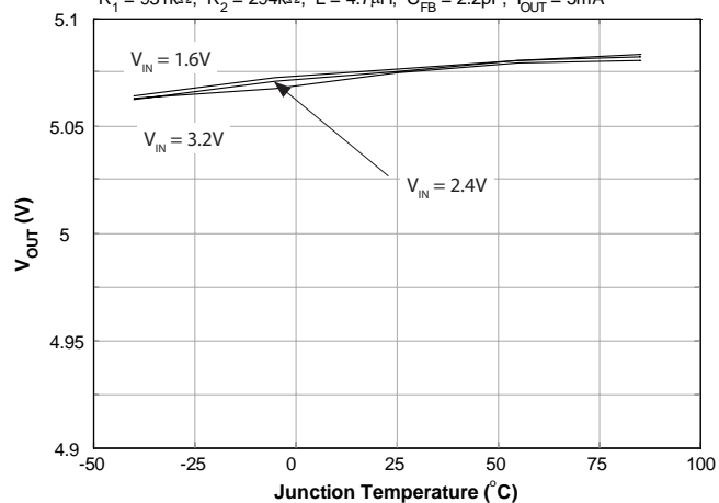
Temperature Reg. — PSAVE Mode ( V_{OUT} = 5.0V )
