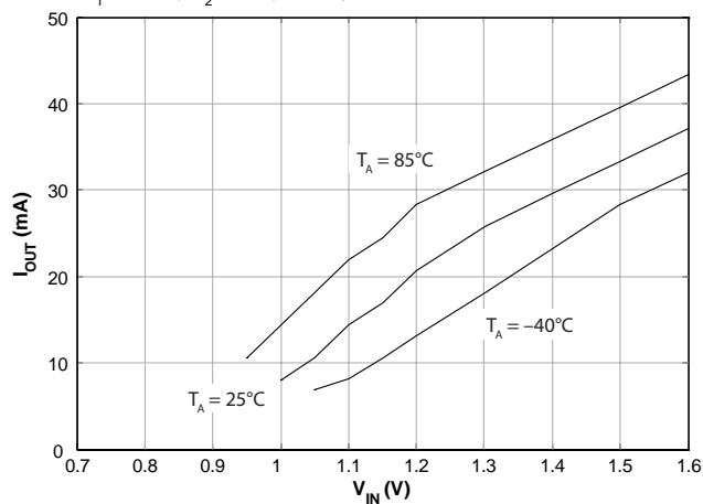
Startup Max. Load Current vs. V_{IN} ( V_{OUT} = 1.8V )
