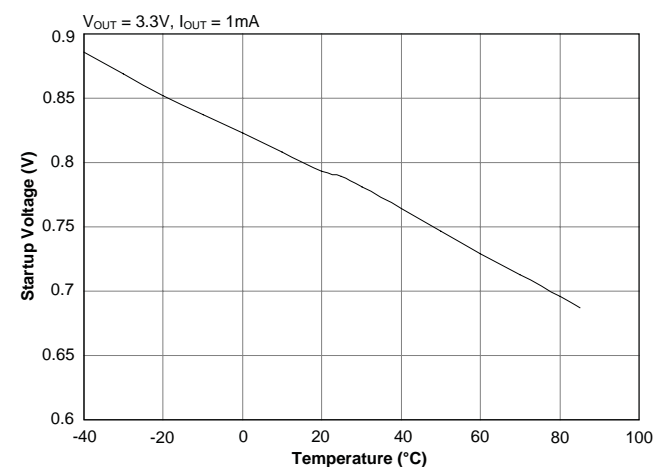
Min. Start-up Voltage vs. Temperature ( V_{OUT} = 3.3V )
