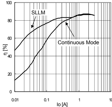
Fig.2 Io-Efficiency (VIN=12V, VOUT=2.5V)
