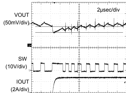
Fig.4 Transient Response (VIN=7V, VOUT=2.5V)
