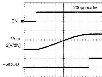
Fig.10 PGOOD Rising Waveform
