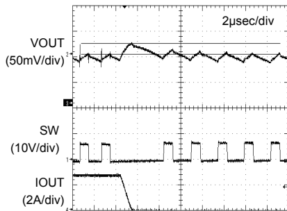
Fig.7 Transient Response (VIN=7V, VOUT=2.5V)
