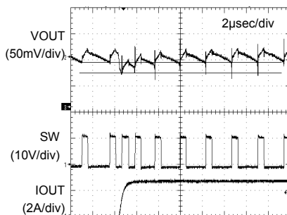
Fig.5 Transient Response (VIN=12V, VOUT=2.5V)
