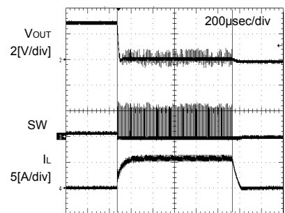
Fig.12 SCP Timer Latch Waveform
