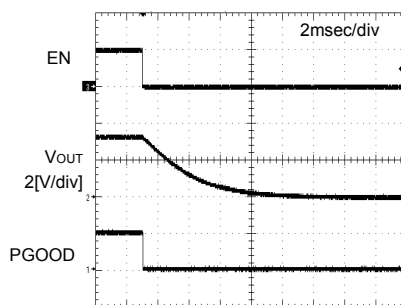
Fig.11 PGOOD Falling Waveform
