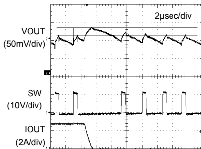
Fig.8 Transient Response (VIN=12V, VOUT=2.5V)
