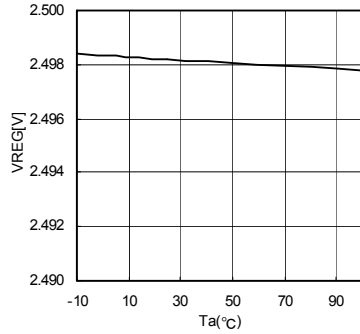
Fig.1 Ta vs VREG
