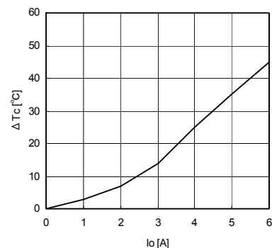
Fig.30 Iout vs ΔTc
