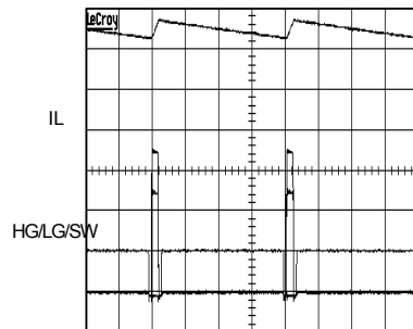
Fig.24 OCP Status (IO=5A)
