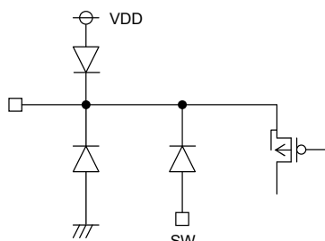
38pin (BOOT)
