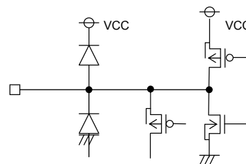
9pin (SS/TRACK)
