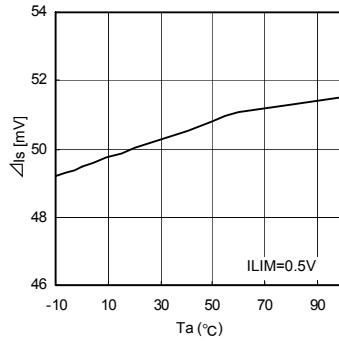
Fig.8 Ta vs Current Limit Threshold
