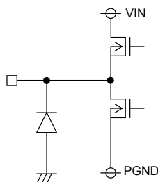
38pin (BOOT)
