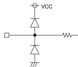
9pin (SS/TRACK)
