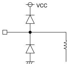
11pin (VOUT)
