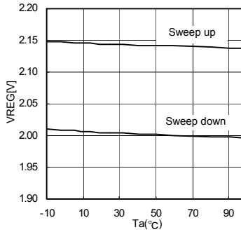
Fig.5 Ta vs EN Threshold
