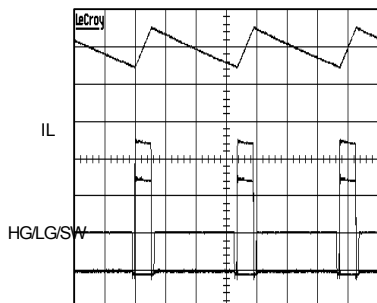
Fig.23 Continuous Mode (IO=4A)
