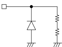
40pin (MODE)
