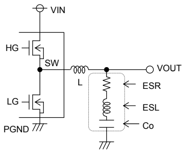
Output Capacitor
