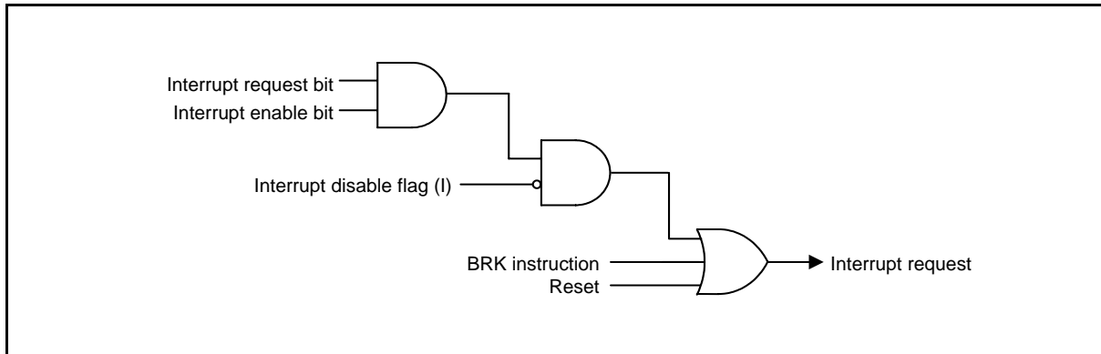
Fig 19. Interrupt control
