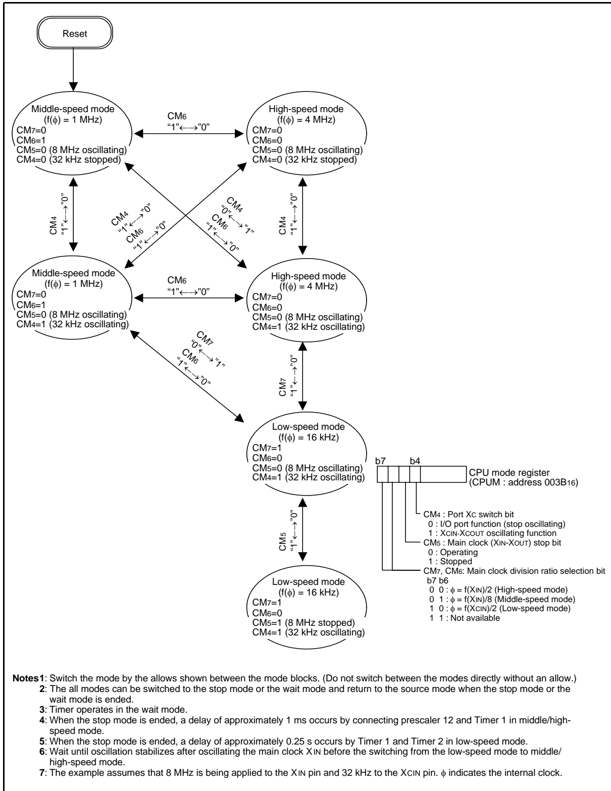
Fig 62. State transitions of system clock
