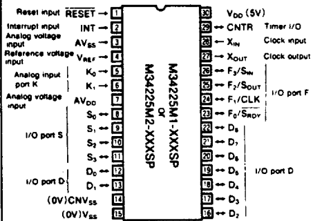
Outline 30P4B
