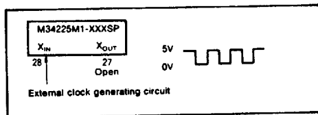
Fig.10 External clock input circuit
