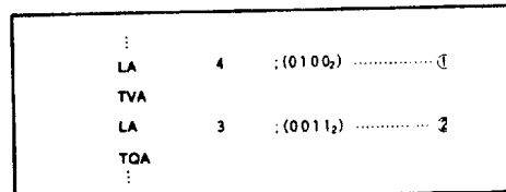
Fig.11 Example program-1
