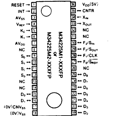
Outline 36P2R
