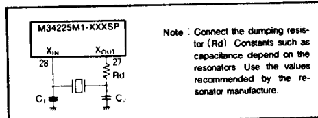
Fig.9 External ceramic resonator circuit
