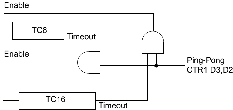
Figure 29. Ping-Pong Mode
