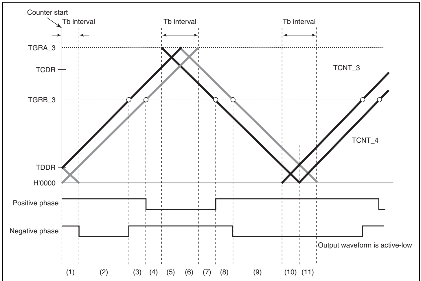
Figure 10.56 Timing for Synchronous Counter Clearing
