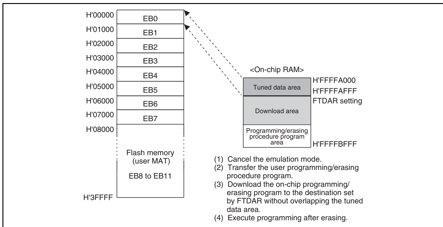
Figure 22.19 Programming of Tuned Data
