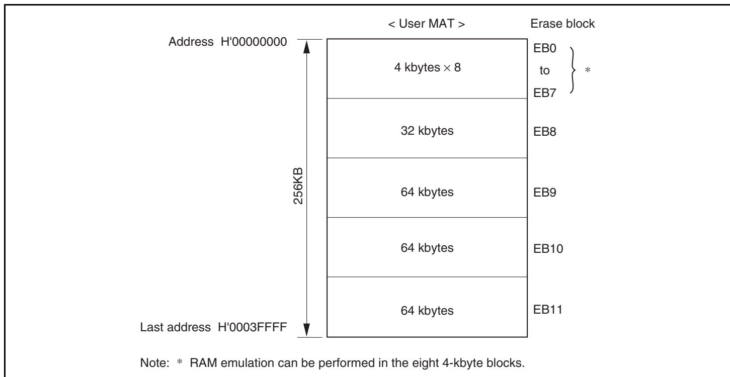
Figure 22.4 Block Division of User MAT
