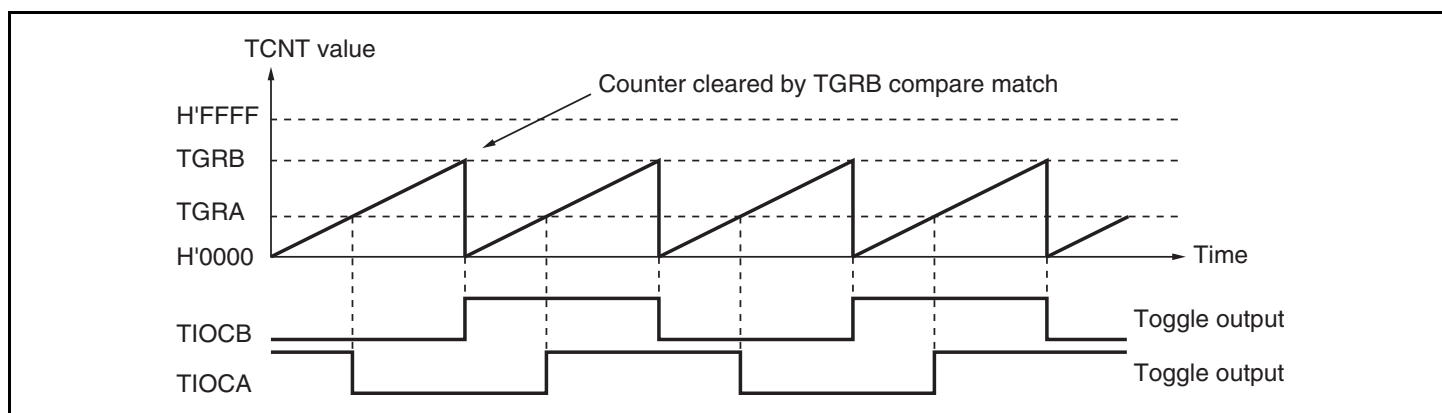
Figure 10.9 Example of Toggle Output Operation
