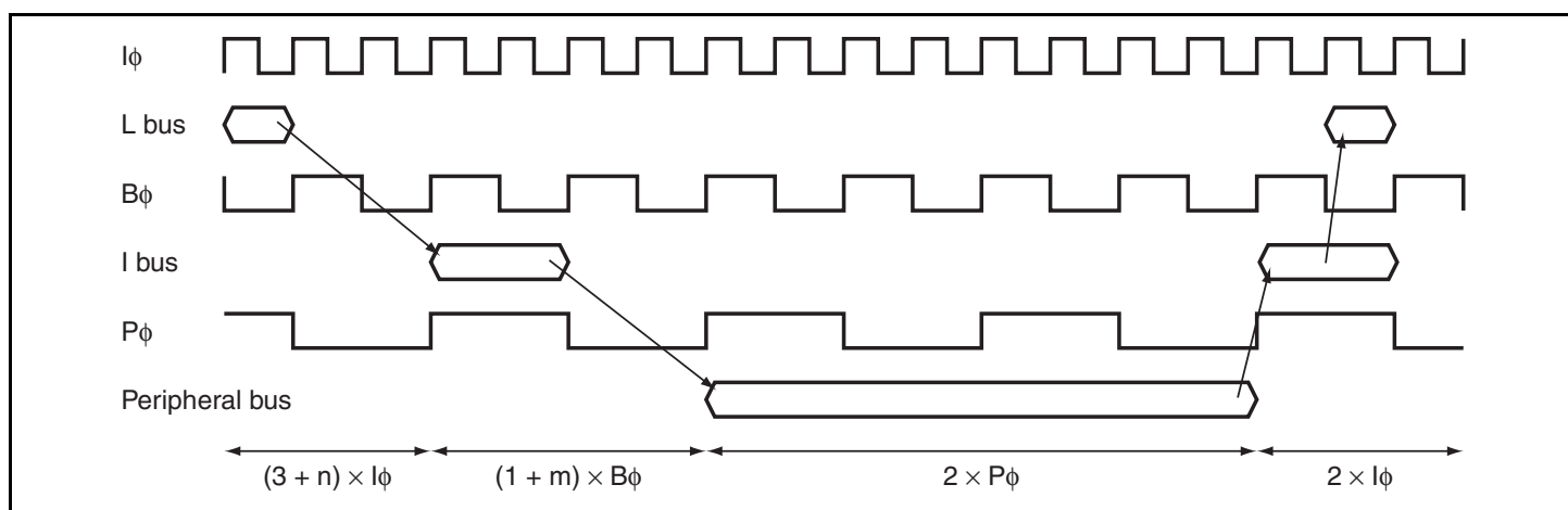
Figure 9.12 Timing of Read Access to On-Chip Peripheral I/O Registers When I\phi:B\phi:P\phi = 4:2:1
