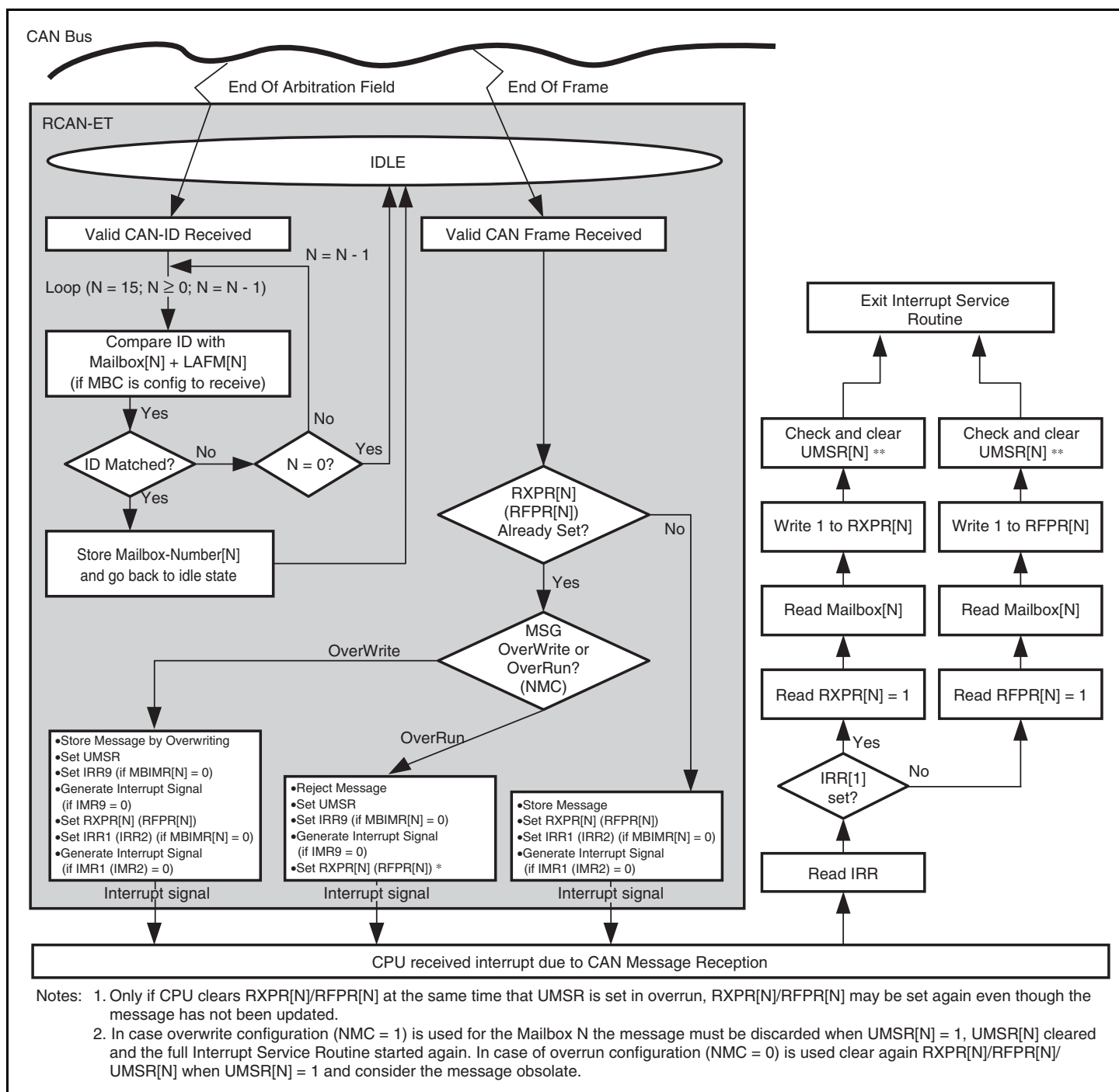
Figure 19.12 Message Receive Sequence
