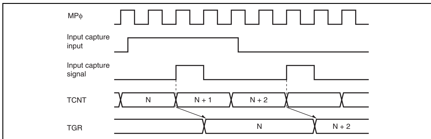
Figure 10.99 Input Capture Input Signal Timing
