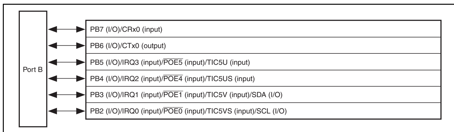
Figure 21.3 Port B (SH7136)
