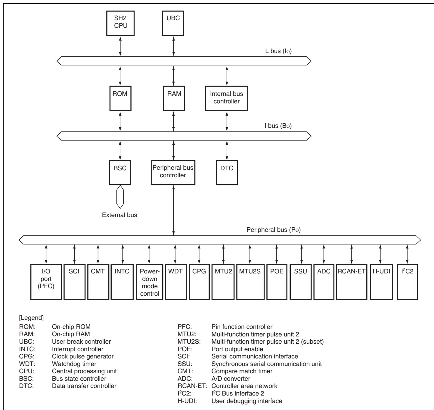
Figure 1.1 Block Diagram
