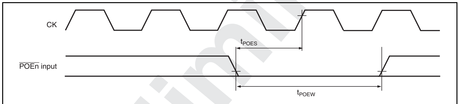
Figure 26.28 POE Input Timing
