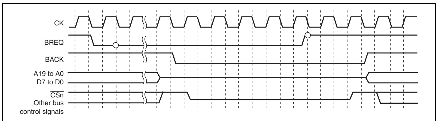
Figure 9.10 Bus Arbitration Timing
