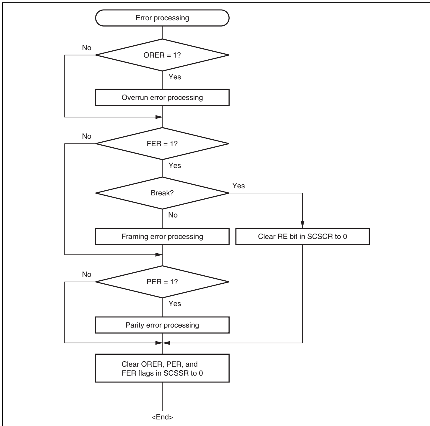
Figure 14.6 Sample Flowchart for Receiving Serial Data (2)
