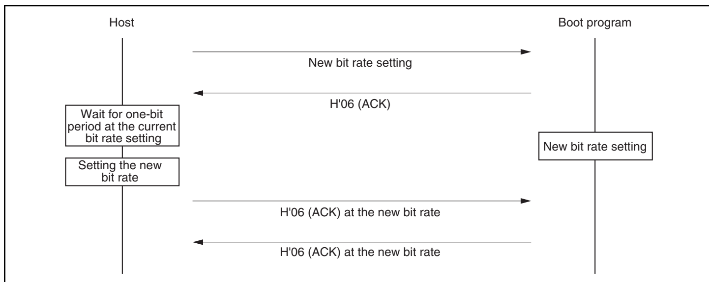
Figure 22.25 Sequence of New Bit Rate Selection
