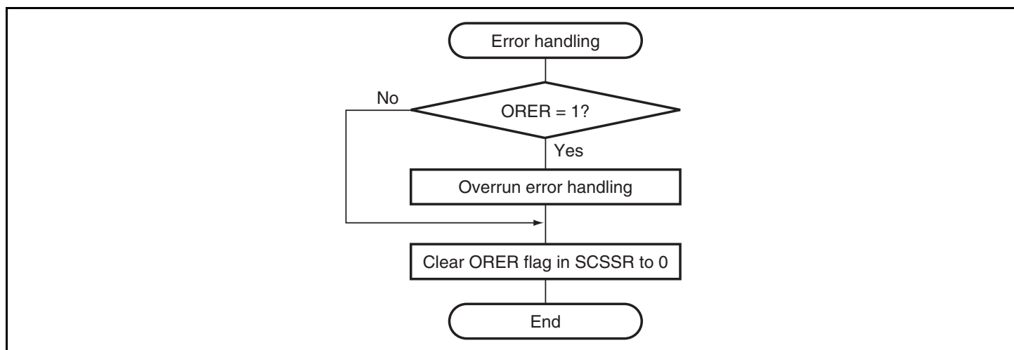
Figure 14.12 Sample Flowchart for Receiving Serial Data (2)
