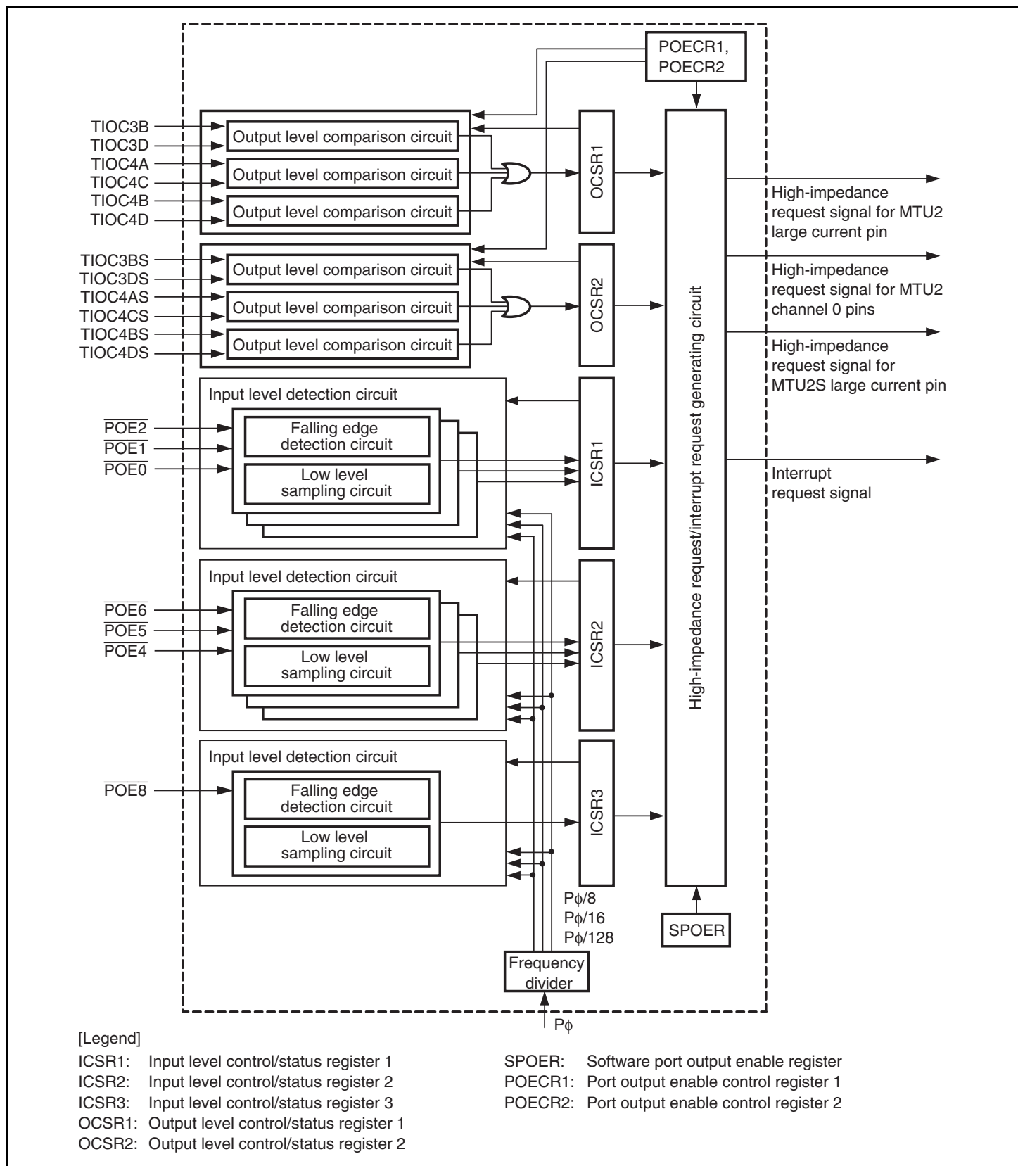
Figure 12.1 Block Diagram of POE
