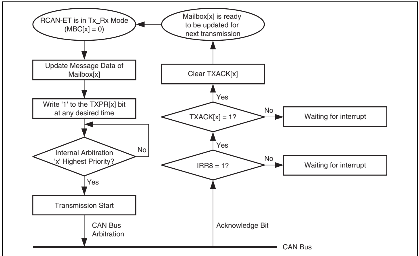
Figure 19.10 Transmission Request
