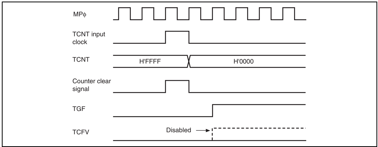
Figure 10.134 Contention between Overflow and Counter Clearing
