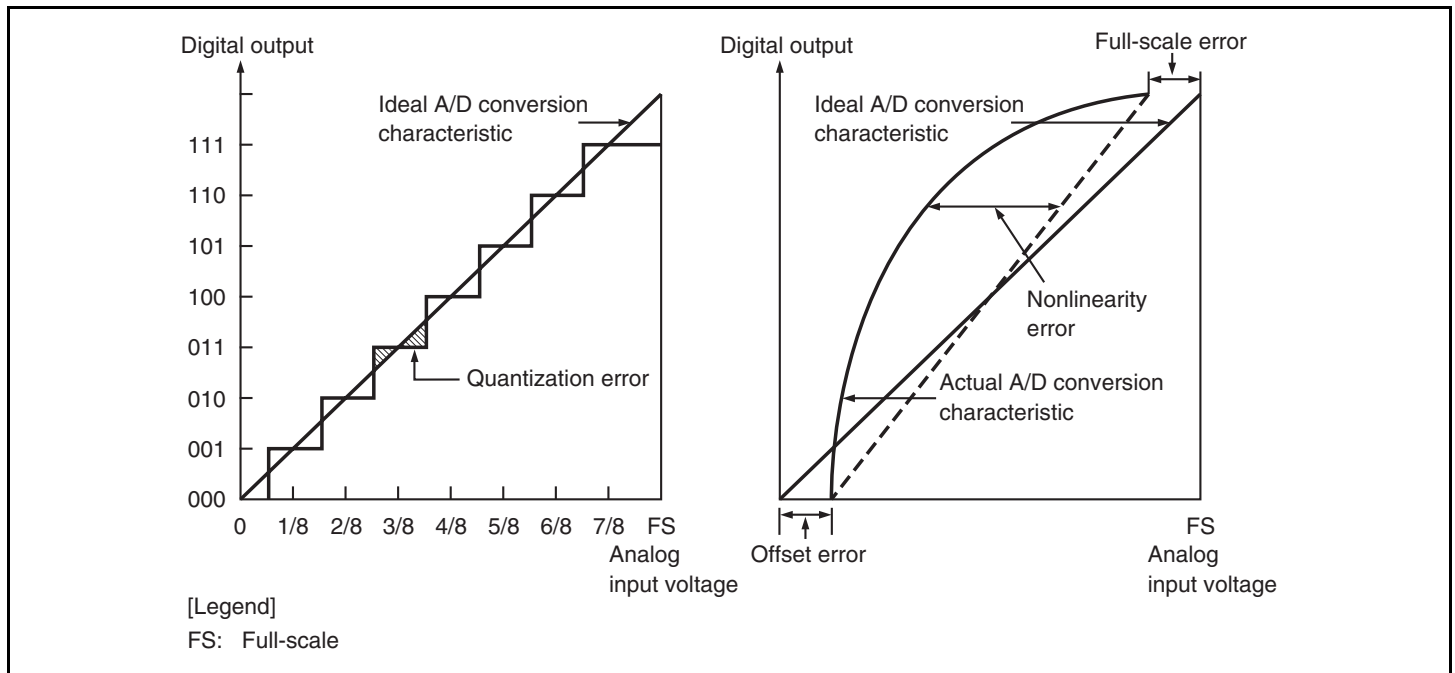
Figure 17.8 Definitions of A/D Conversion Accuracy
