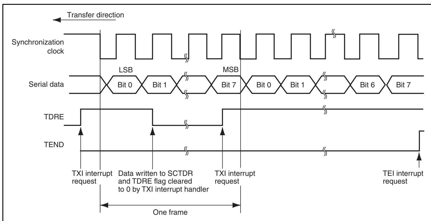
Figure 14.11 Example of SCI Transmit Operation
