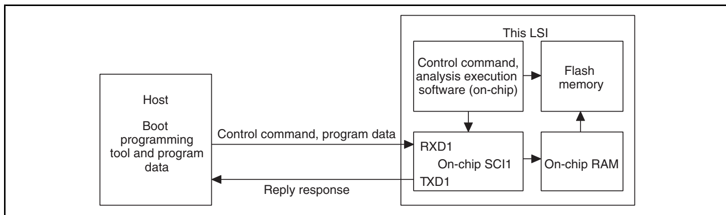
Figure 22.6 System Configuration in Boot Mode
