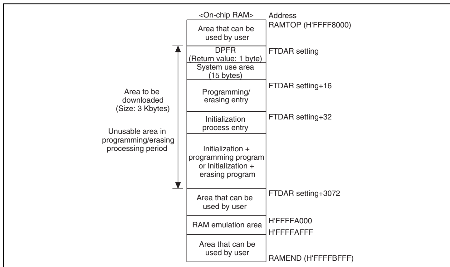
Figure 22.10 RAM Map after Download
