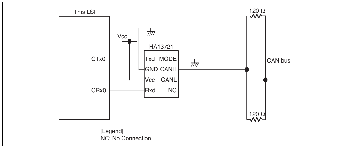
Figure 19.15 High-Speed CAN Interface Using HA13721
