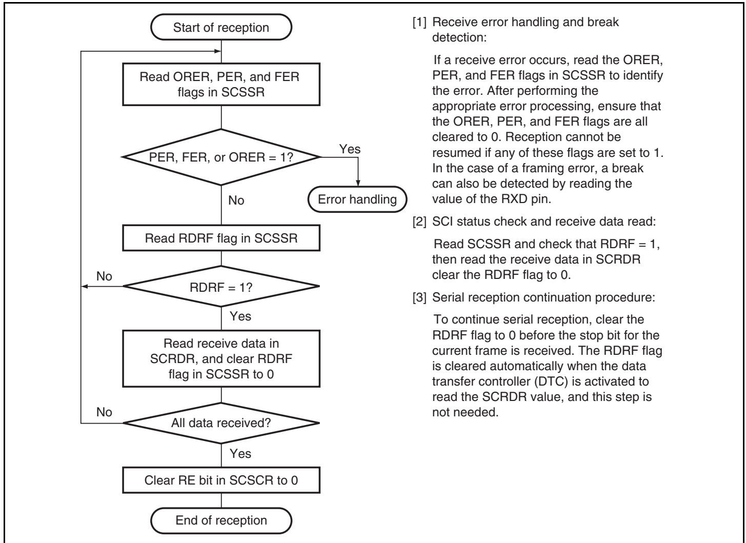
Figure 14.6 Sample Flowchart for Receiving Serial Data (1)
