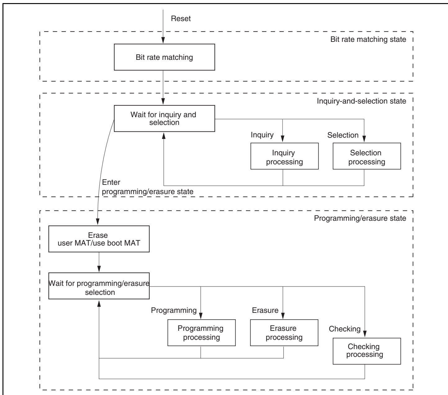
Figure 22.22 Flow of Processing by the Boot Program
