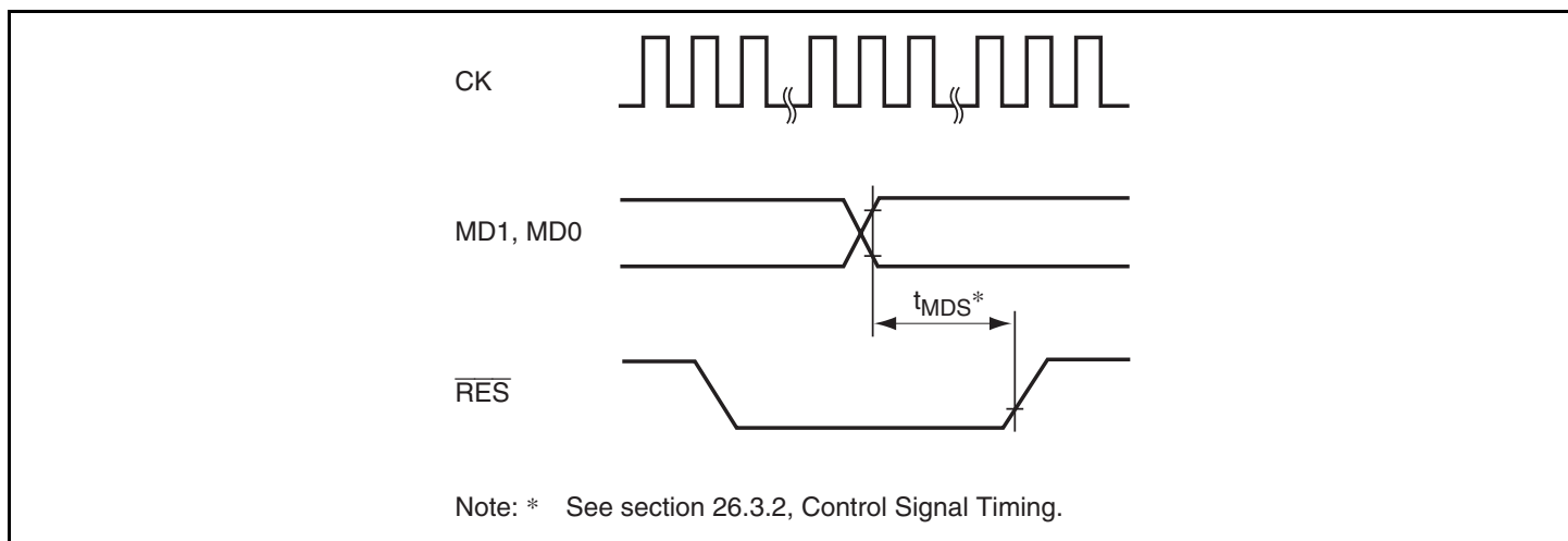
Figure 3.3 Reset Input Timing when Changing Operating Mode
