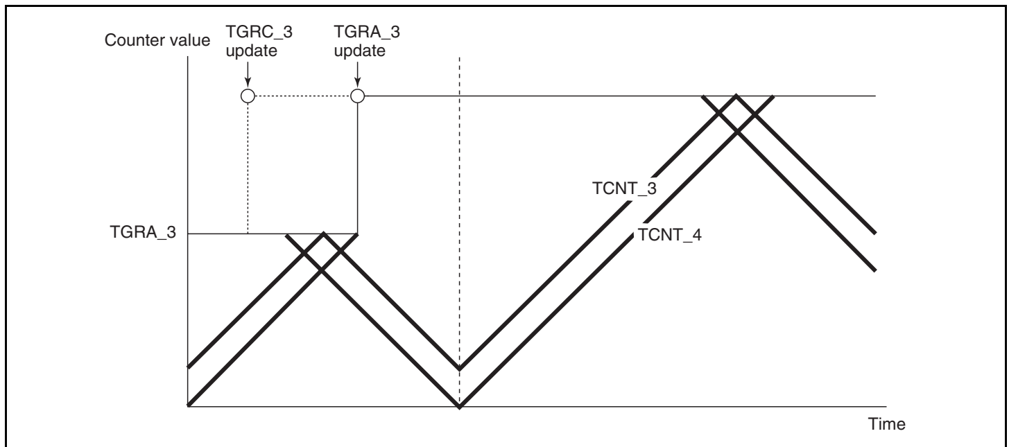
Figure 10.42 Example of PWM Cycle Updating
