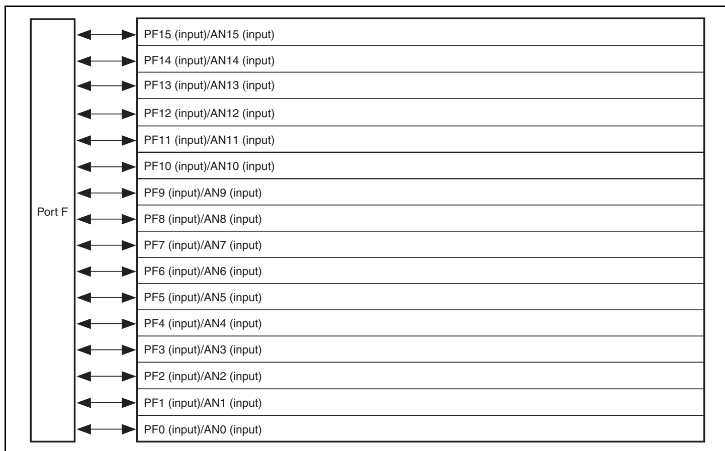
Figure 21.9 Port F (SH7137)
