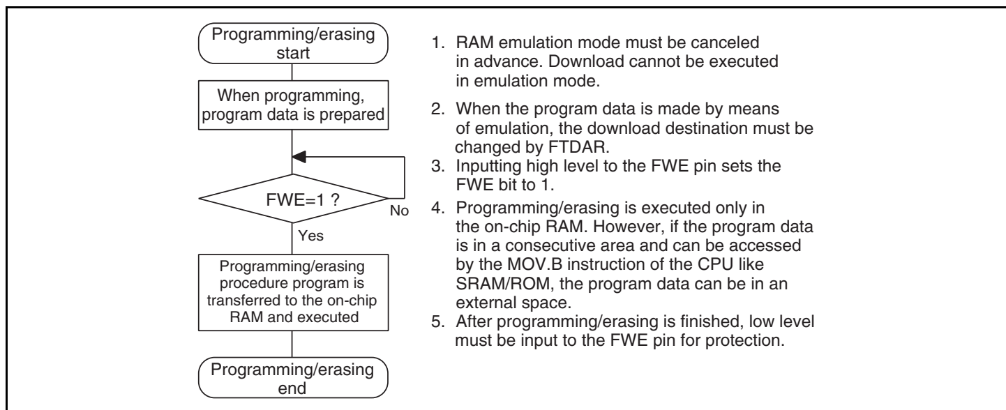
Figure 22.9 Programming/Erasing Overview Flow
