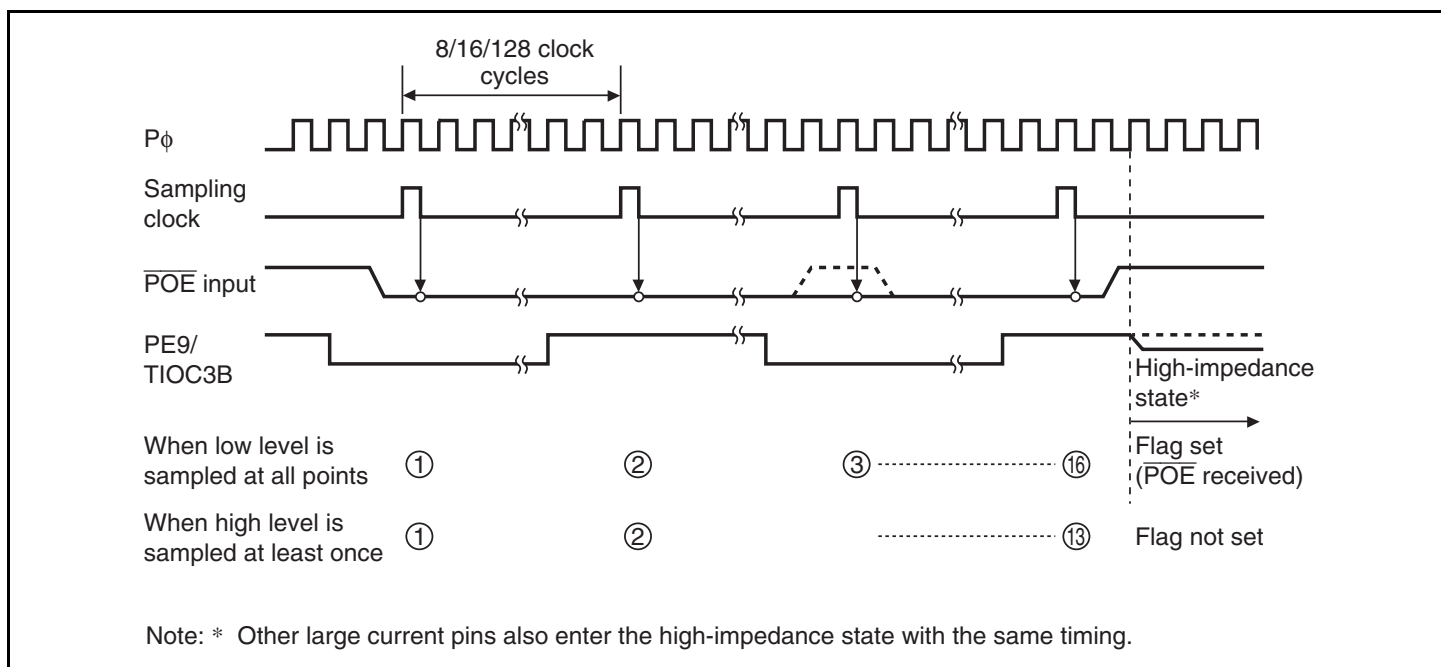
Figure 12.3 Low-Level Detection Operation
