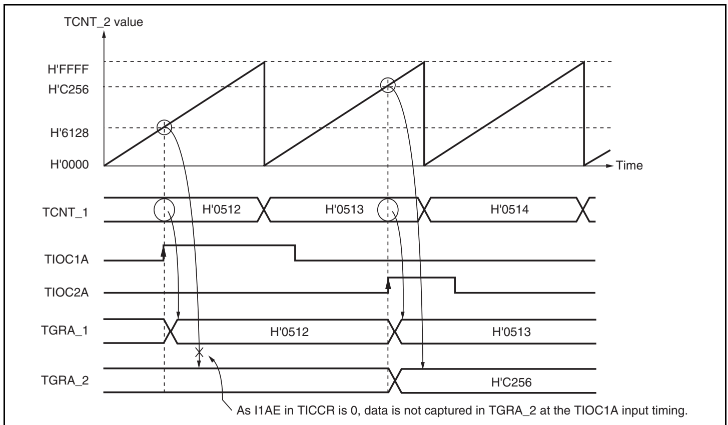
Figure 10.22 Cascaded Operation Example (b)
