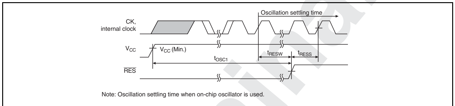
Figure 26.3 Power-On Oscillation Settling Timing
