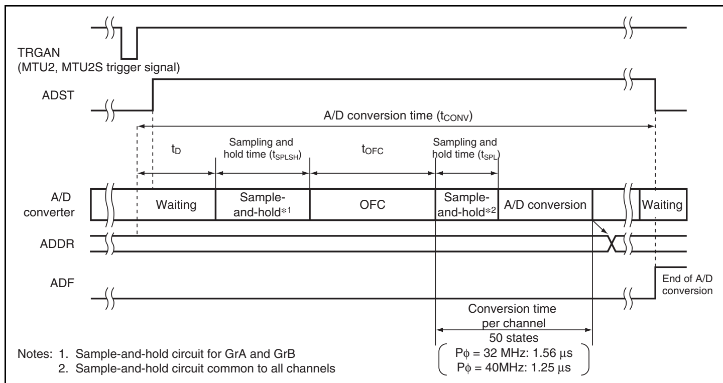
Figure 17.5 A/D Conversion Timing (Single-Cycle Scan Mode)
