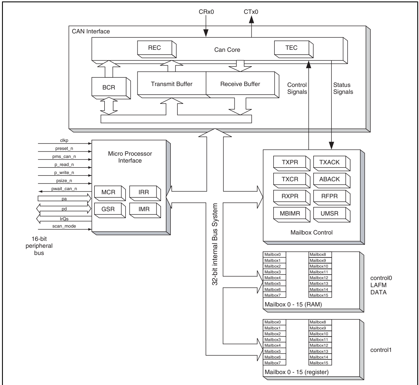
Figure 19.1 RCAN-ET Architecture
