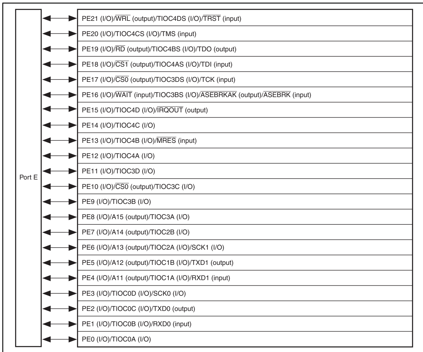
Figure 21.7 Port E (SH7137)
