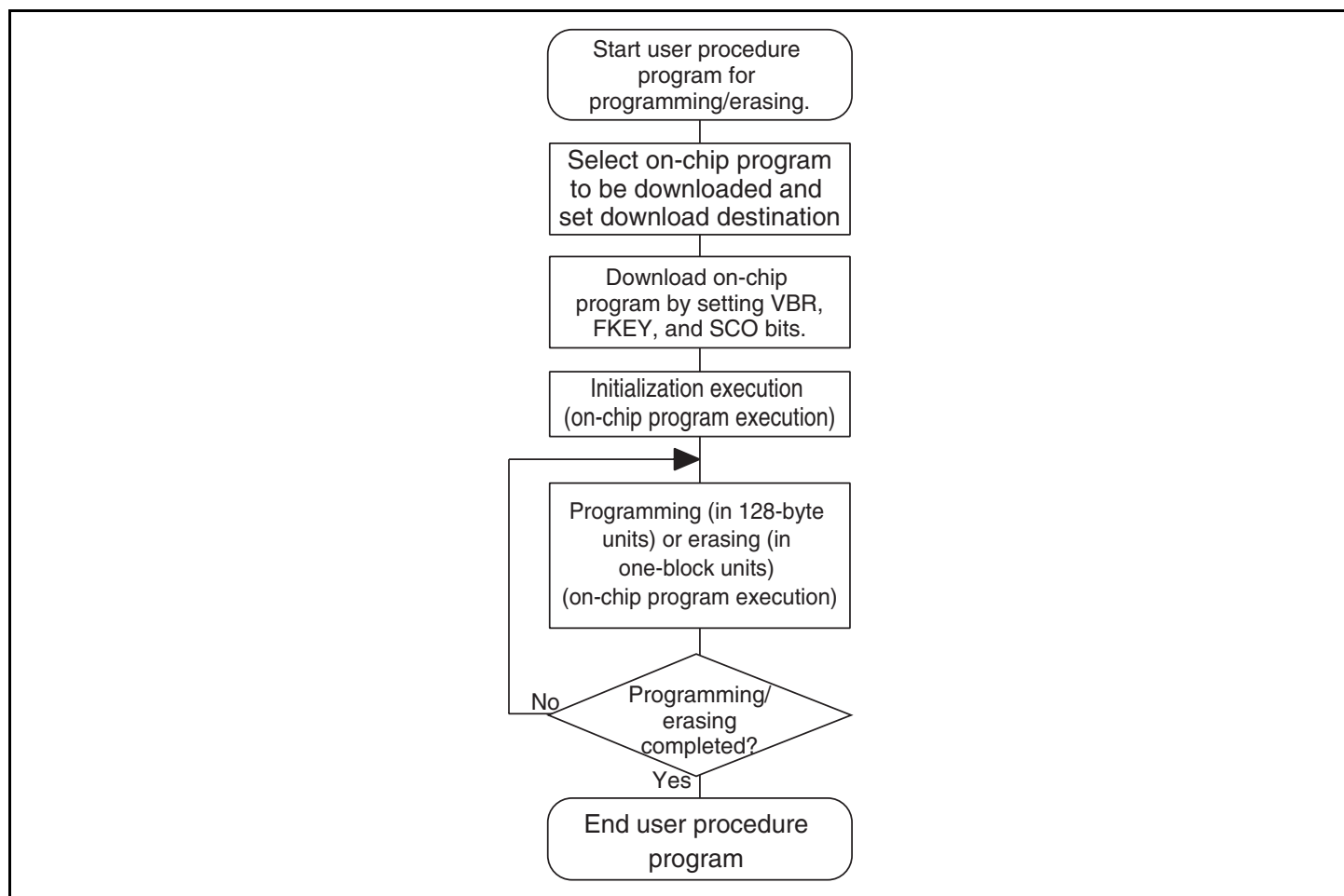
Figure 22.5 Overview of User Procedure Program
