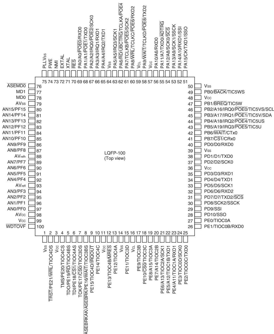
Figure 1.3 SH7137 Pin Assignments
