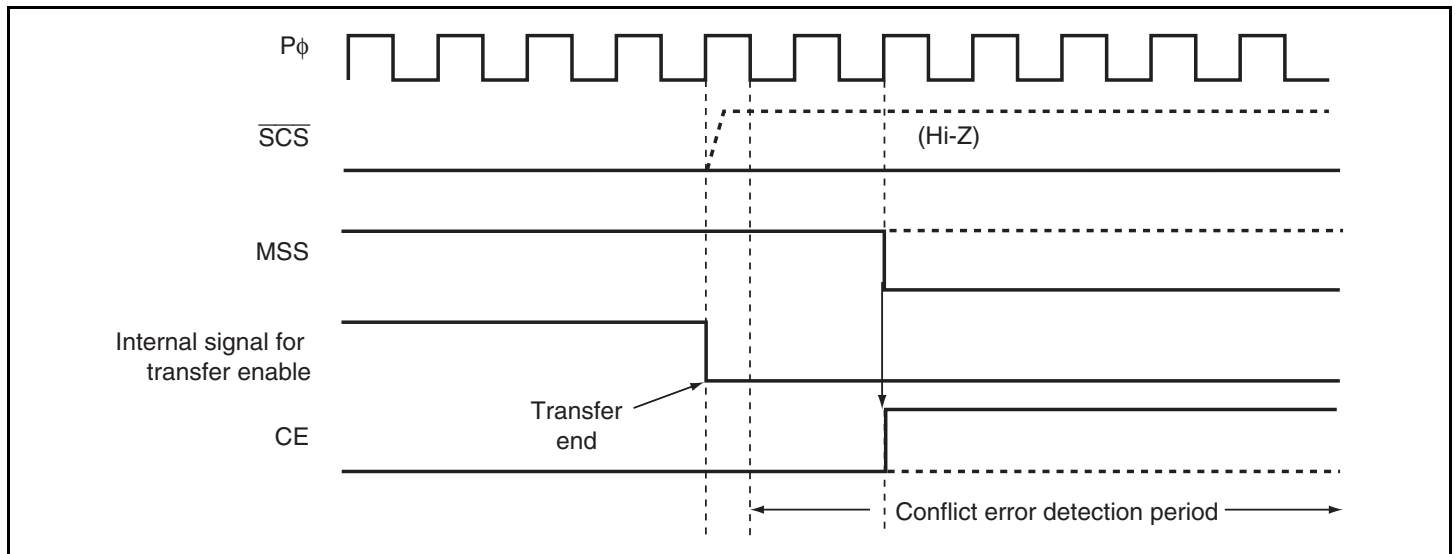
Figure 15.11 Conflict Error Detection Timing (After Transfer End)
