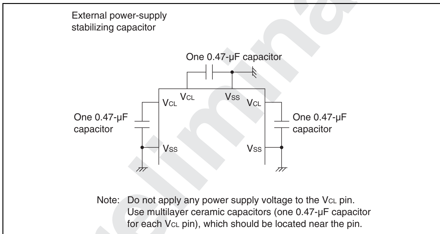
Figure 26.33 Connection of V_{CL} Capacitor
