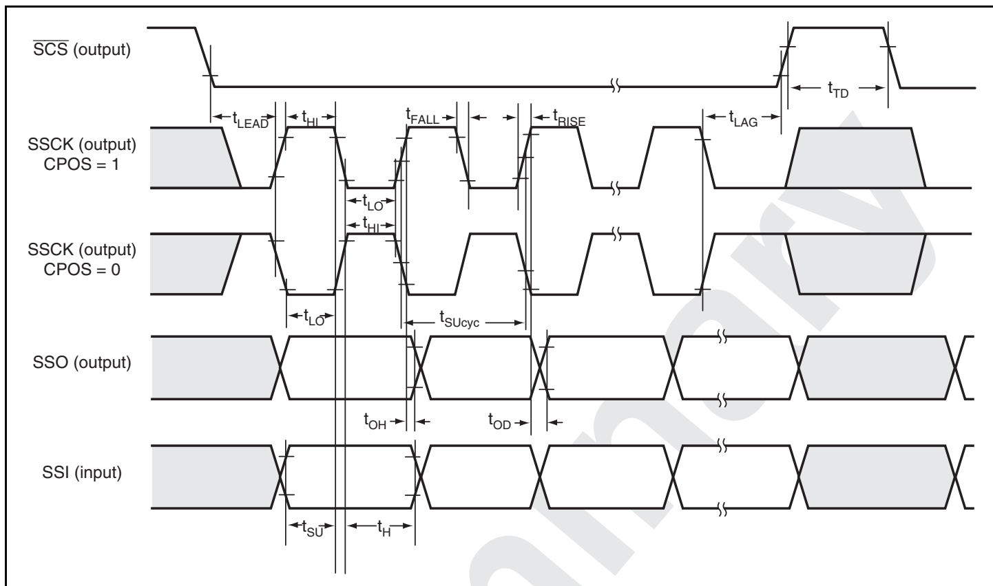
Figure 26.24 SSU Timing (Master, CPHS = 0)
