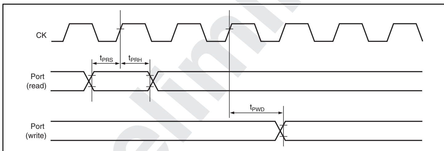
Figure 26.19 I/O Port Input/Output Timing
