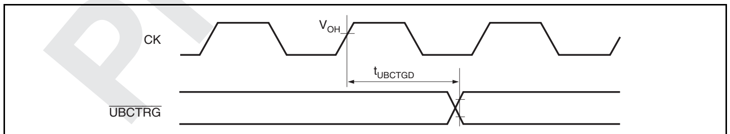
Figure 26.30 UBC Trigger Timing
