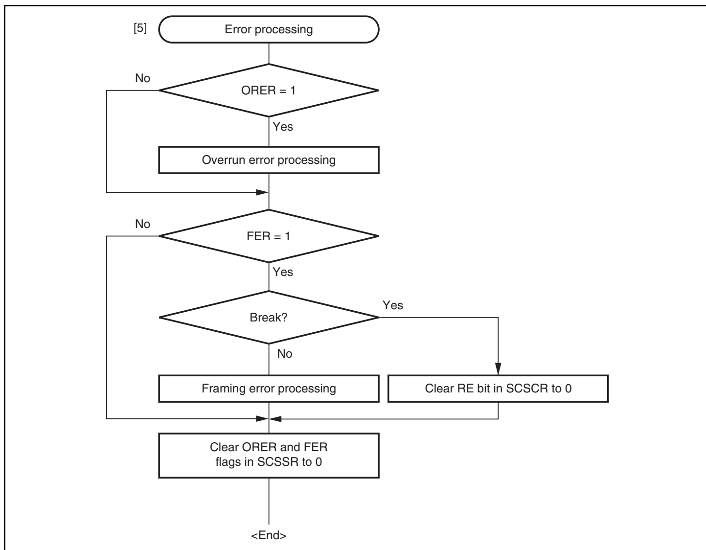
Figure 14.18 Sample Multiprocessor Serial Reception Flowchart (2)
