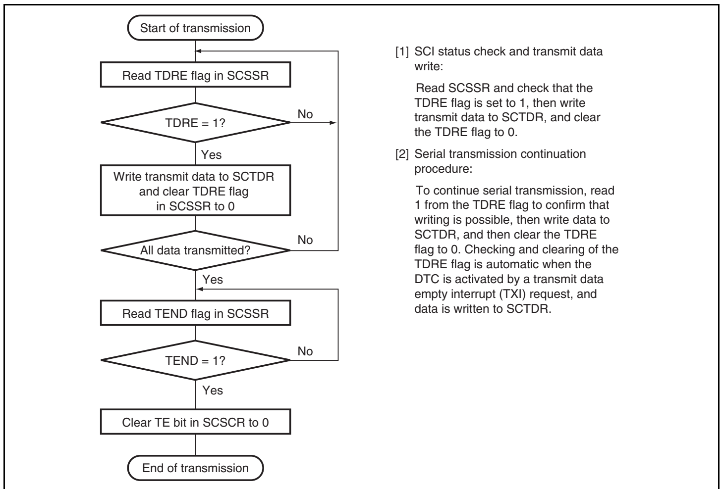
Figure 14.10 Sample Flowchart for Transmitting Serial Data
