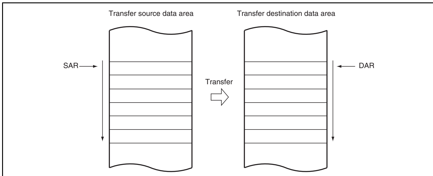
Figure 8.6 Memory Map in Normal Transfer Mode
