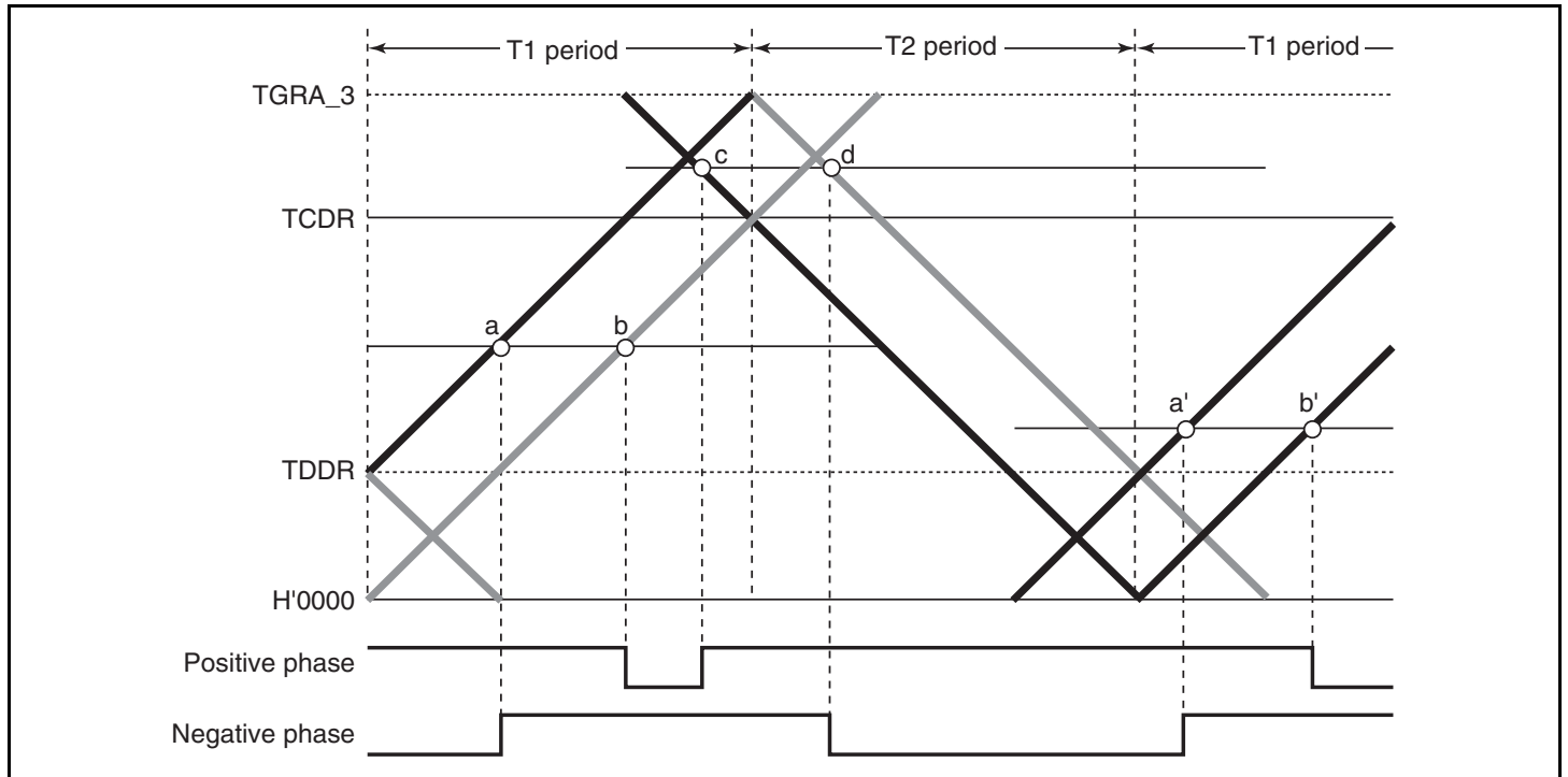
Figure 10.46 Example of Complementary PWM Mode Waveform Output (1)
