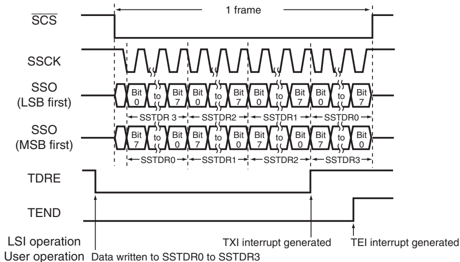
Figure 15.5 Example of Transmission Operation (SSU Mode)
