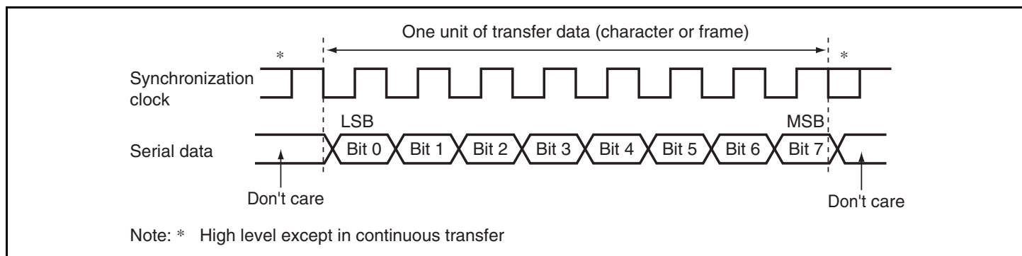
Figure 14.8 Data Format in Clock Synchronous Communication
