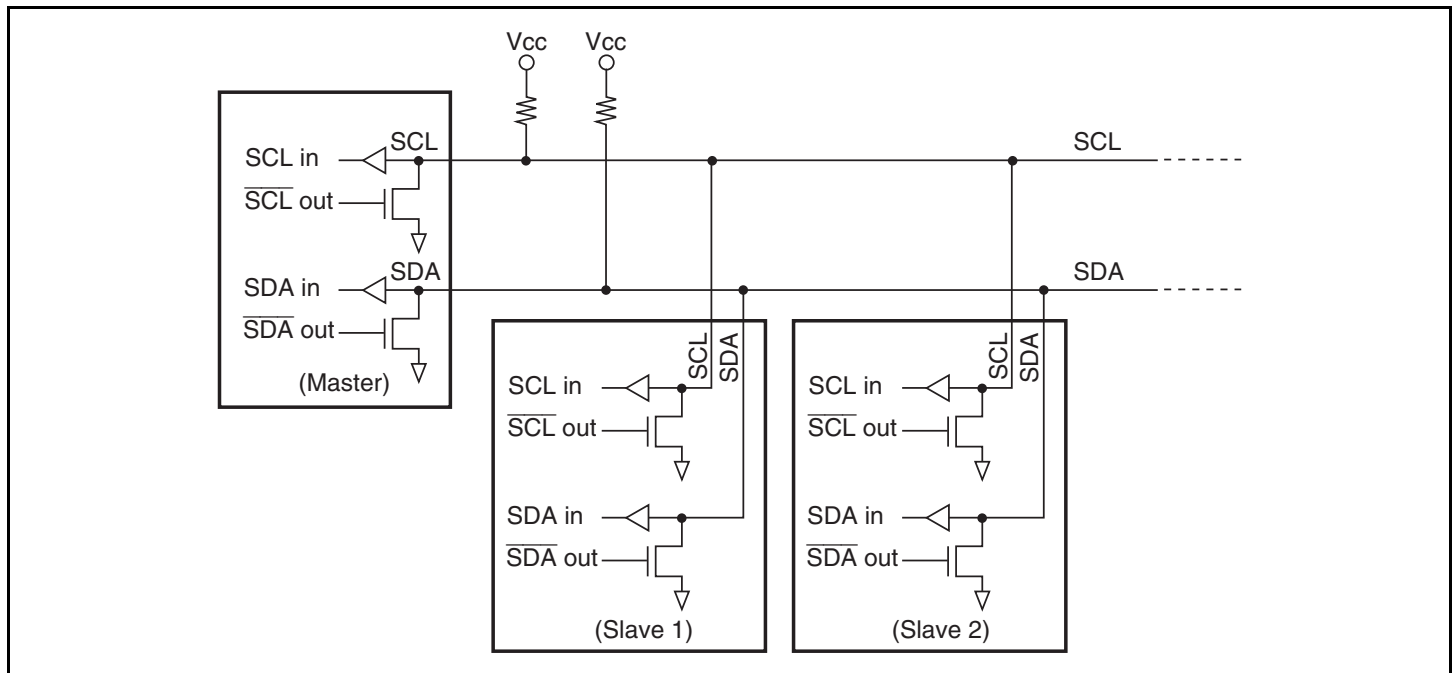
Figure 16.2 External Circuit Connections of I/O Pins
