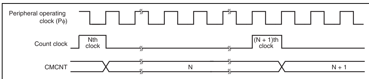
Figure 18.3 Count Timing
