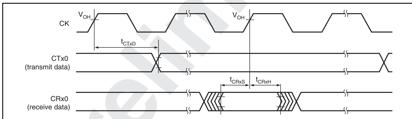
Figure 26.27 RCAN-ET Input/Output Timing
