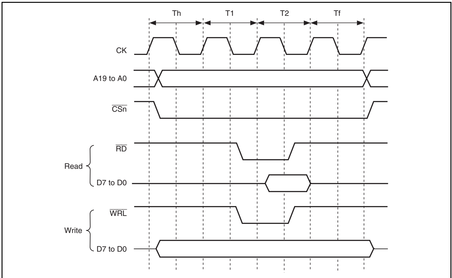
Figure 9.8 \overline{\text{CSn}} Assert Period Extension
