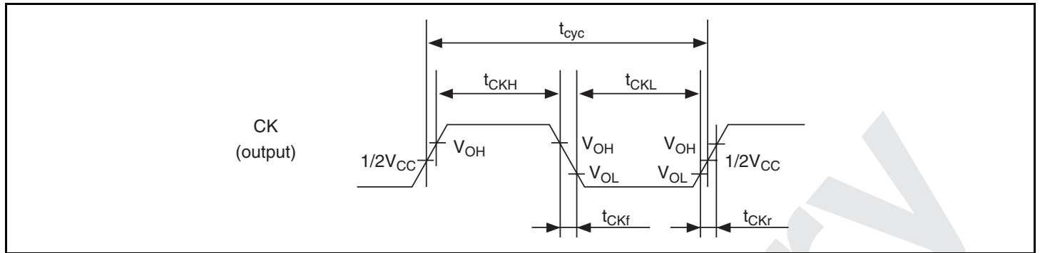
Figure 26.2 CK Clock Output Timing
