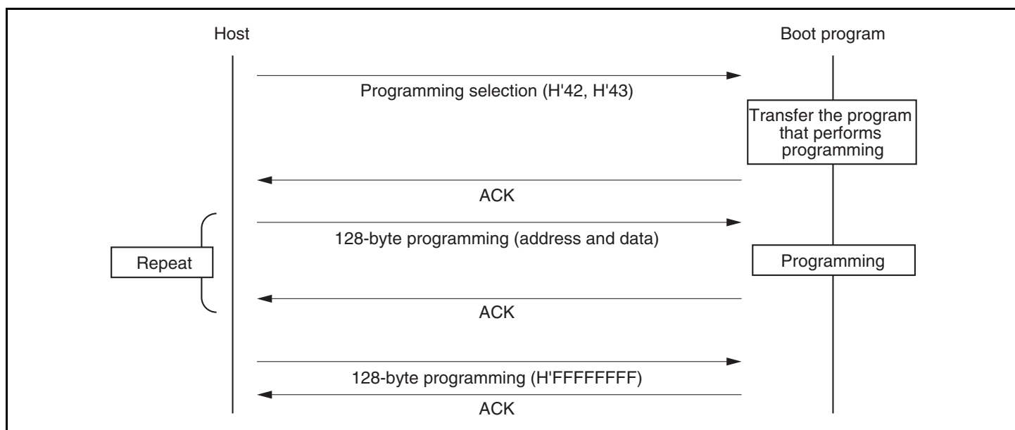
Figure 22.26 Sequence of Programming
