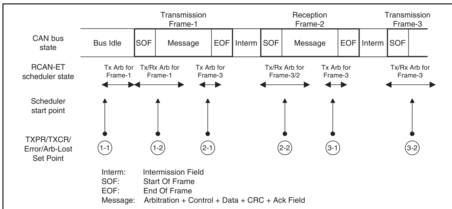
Figure 19.11 Internal Arbitration for Transmission
