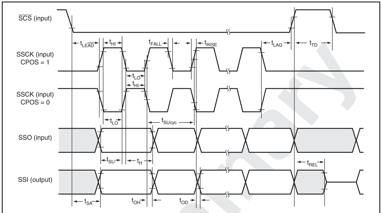
Figure 26.26 SSU Timing (Slave, CPHS = 0)
