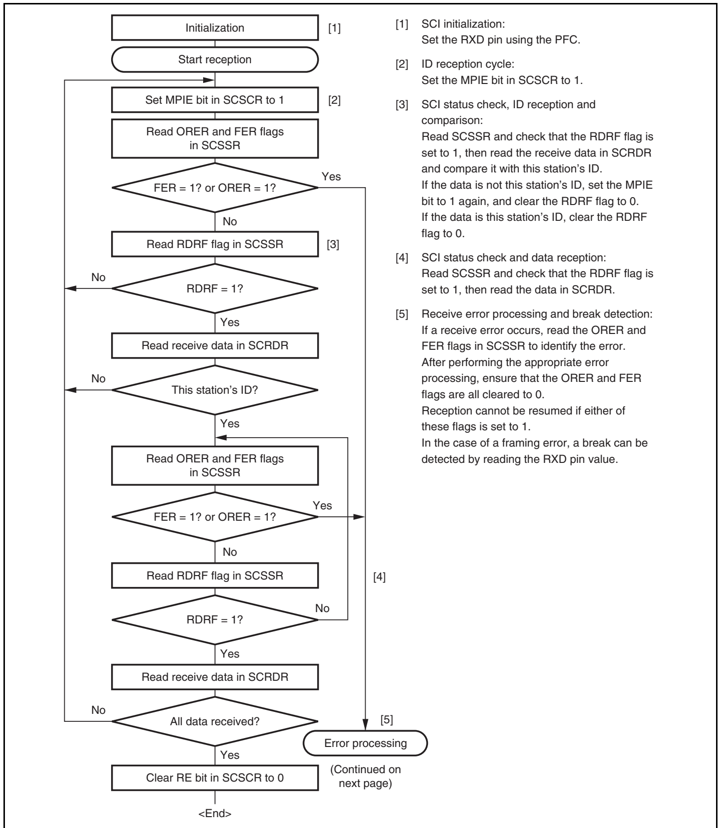
Figure 14.18 Sample Multiprocessor Serial Reception Flowchart (1)
