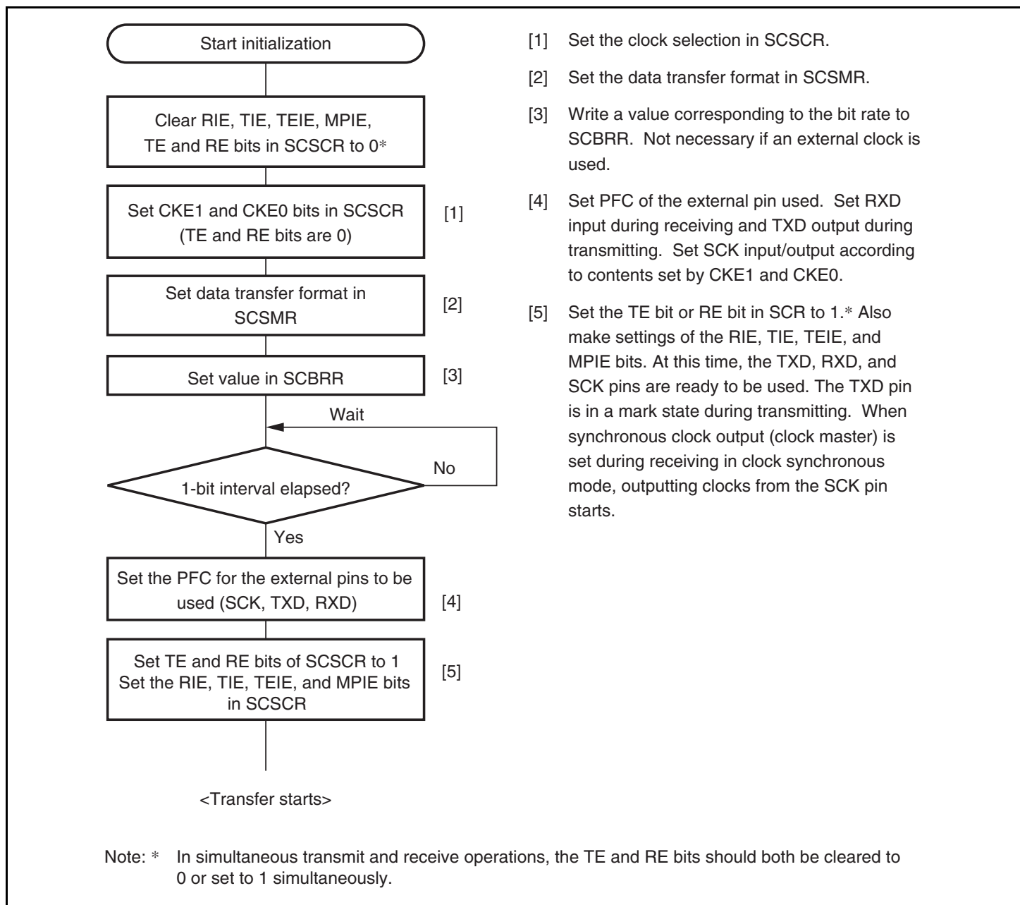
Figure 14.9 Sample Flowchart for SCI Initialization
