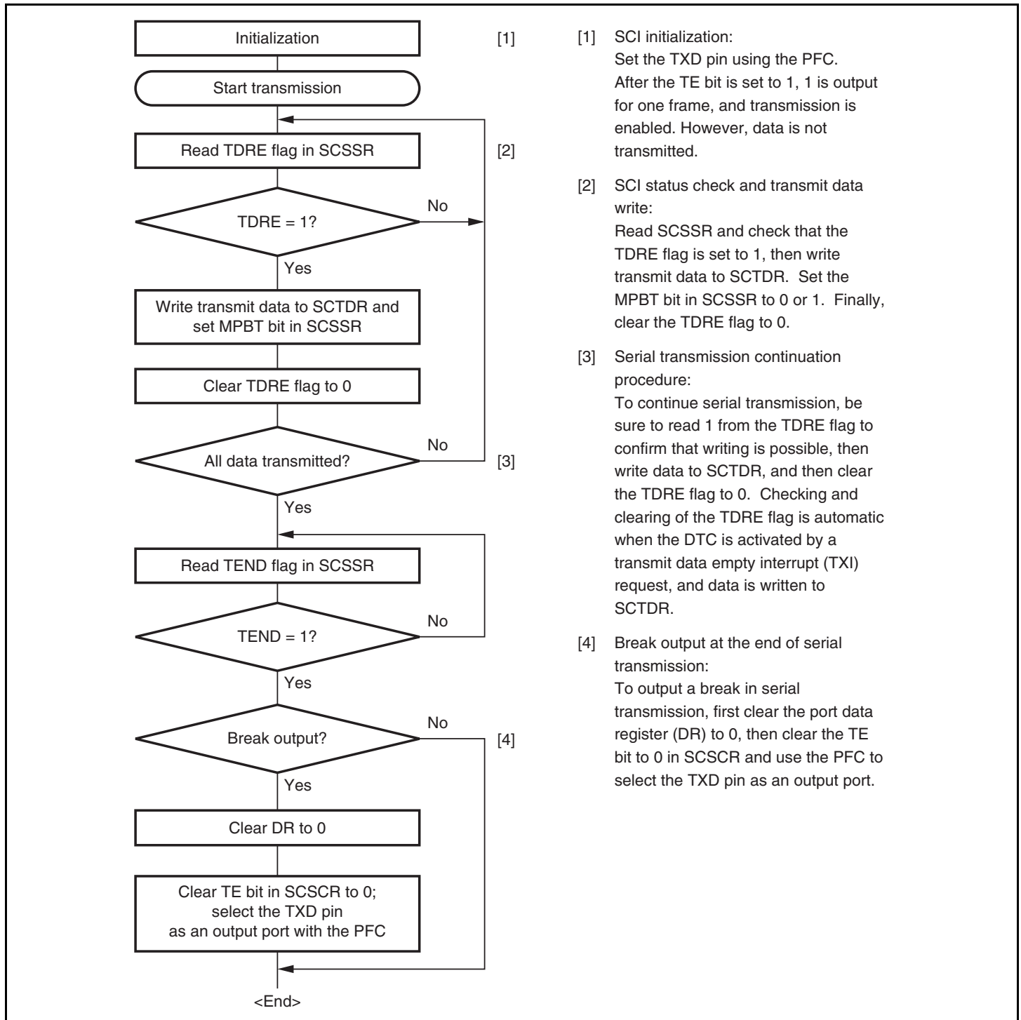
Figure 14.16 Sample Multiprocessor Serial Transmission Flowchart
