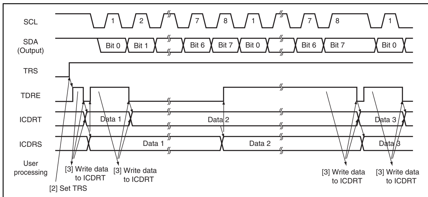
Figure 16.14 Transmit Mode Operation Timing
