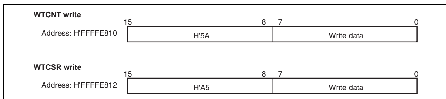
Figure 13.2 Writing to WTCNT and WTCSR
