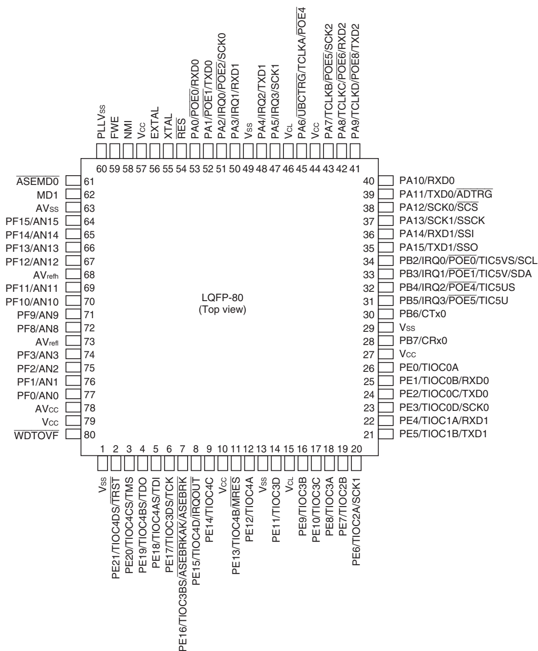
Figure 1.2 SH7136 Pin Assignments
