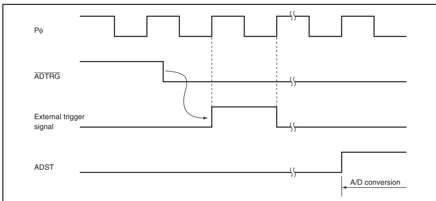
Figure 17.6 External Trigger Input Timing
