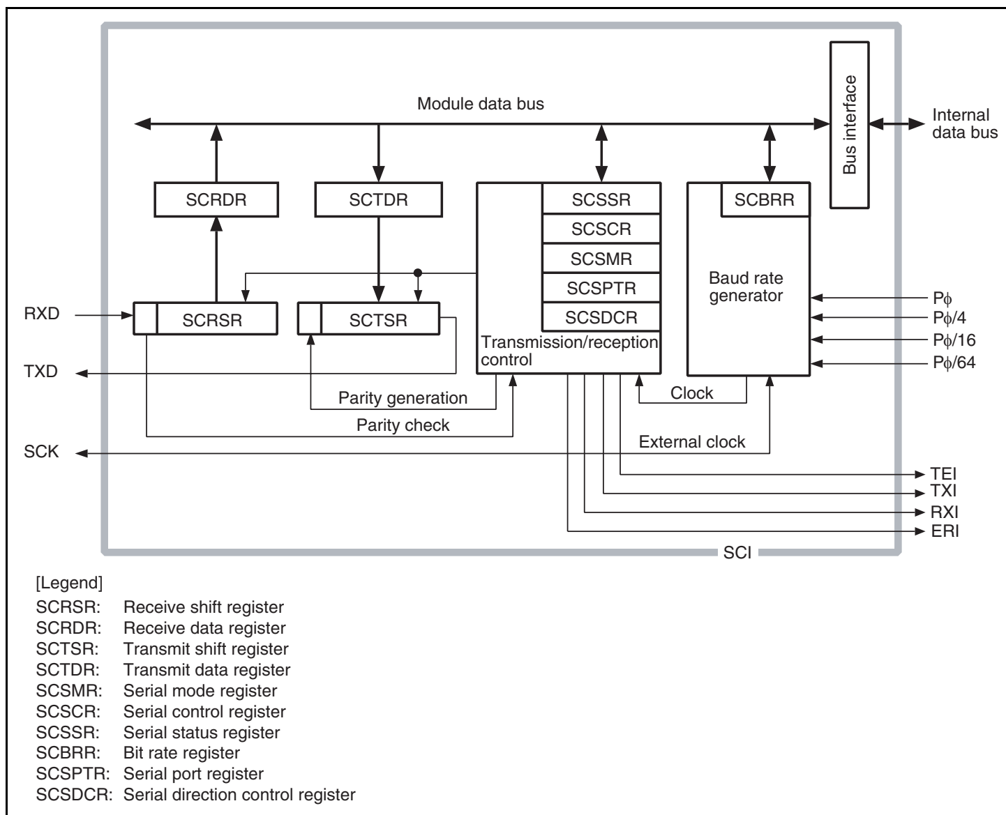
Figure 14.1 Block Diagram of SCI
