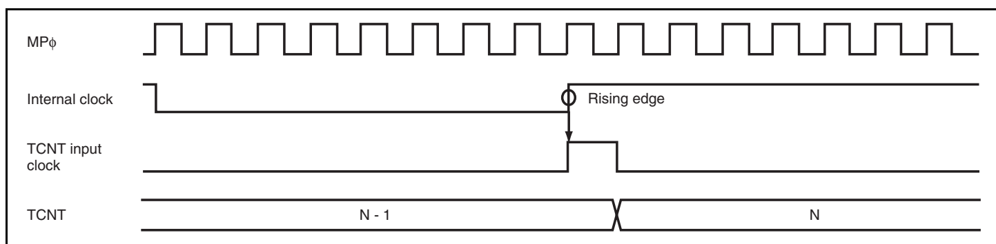
Figure 10.94 Count Timing in Internal Clock Operation (Channel 5)
