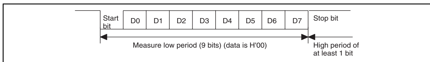
Figure 22.7 Automatic Adjustment Operation of SCI Bit Rate
