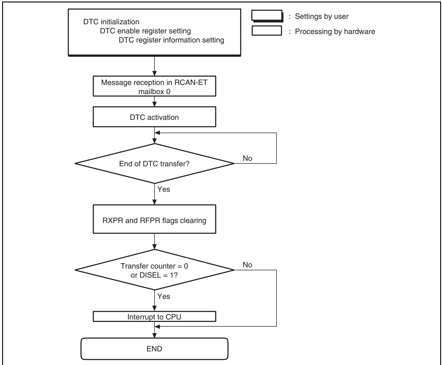
Figure 19.14 DTC Transfer Flowchart
