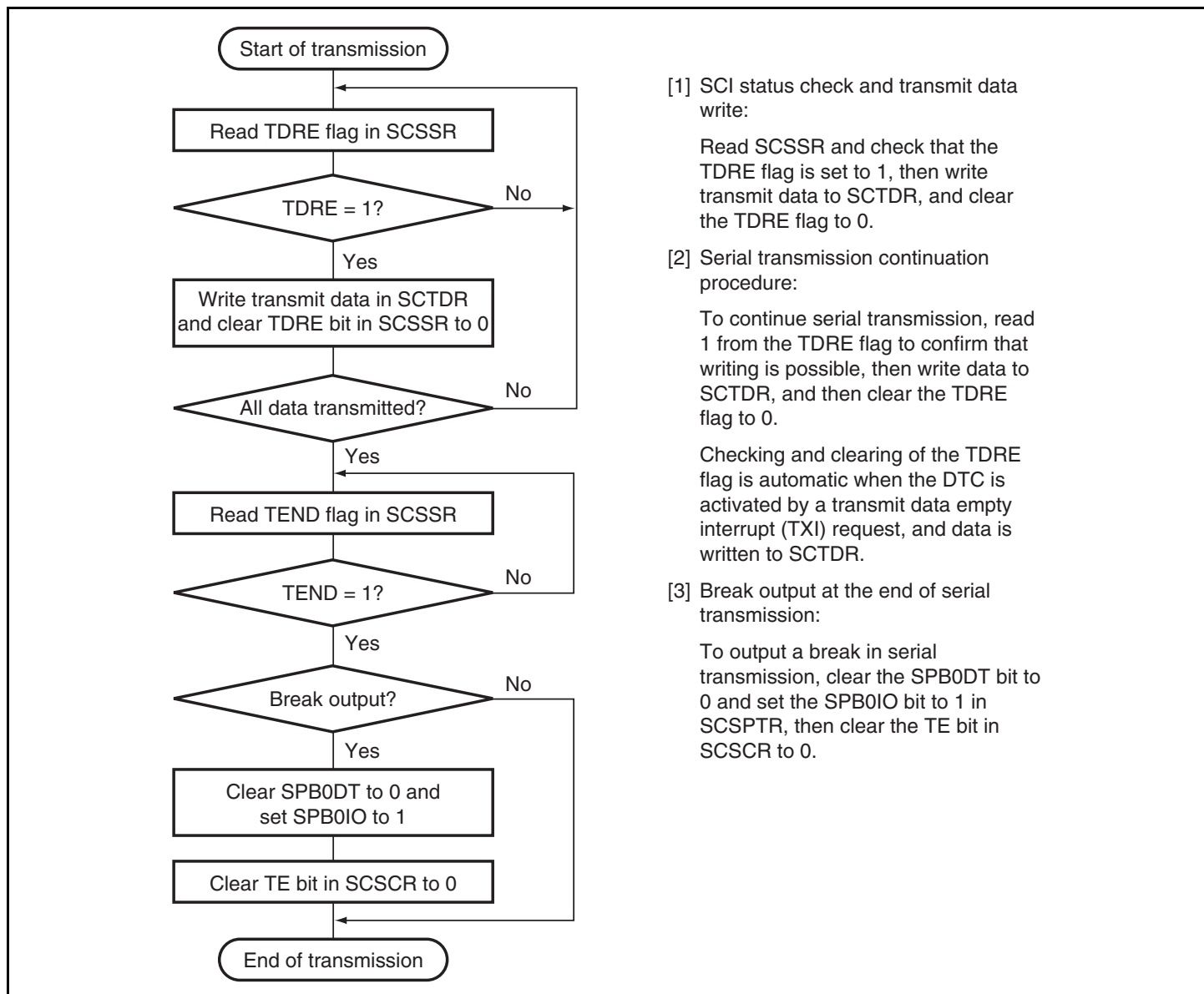
Figure 14.4 Sample Flowchart for Transmitting Serial Data
