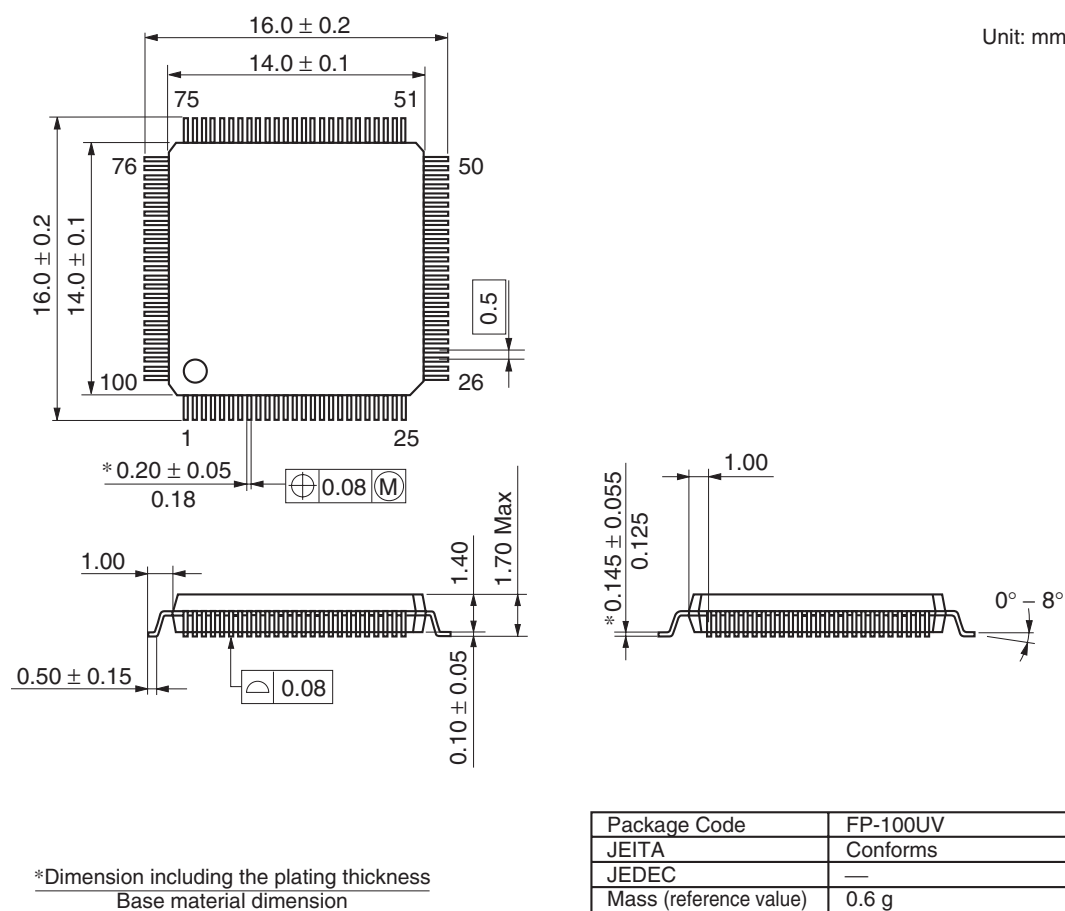
Figure D.2 FP-100UV
