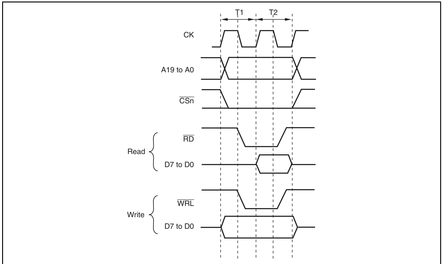
Figure 9.2 Normal Space Basic Access Timing (Access Wait 0)
