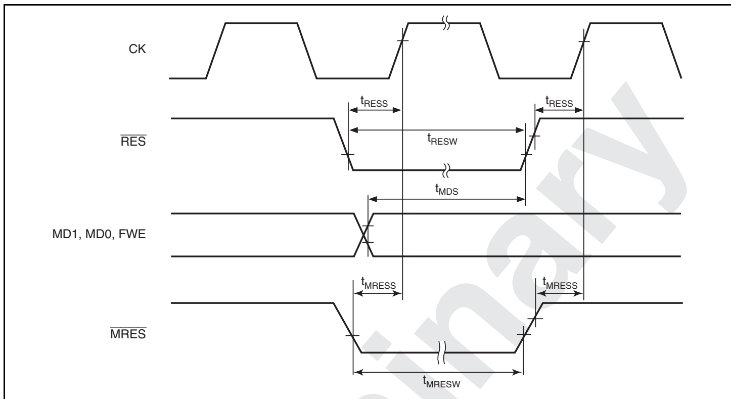
Figure 26.6 Reset Input Timing
