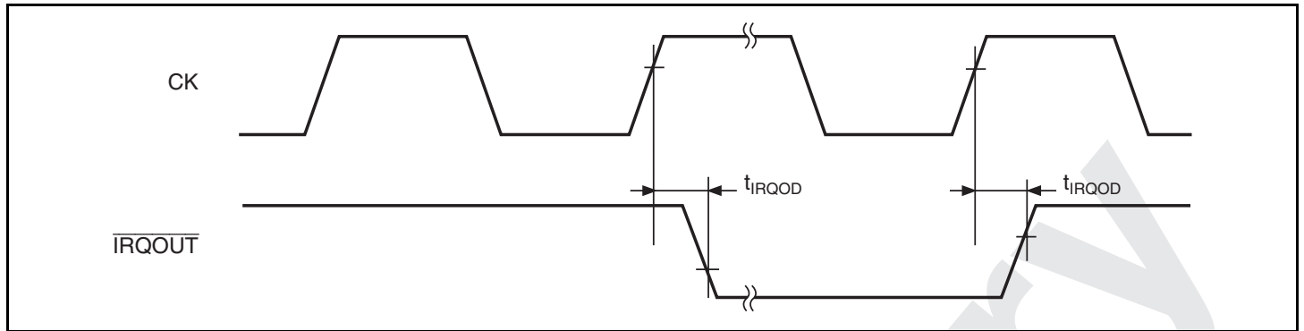
Figure 26.8 Interrupt Signal Output Timing
