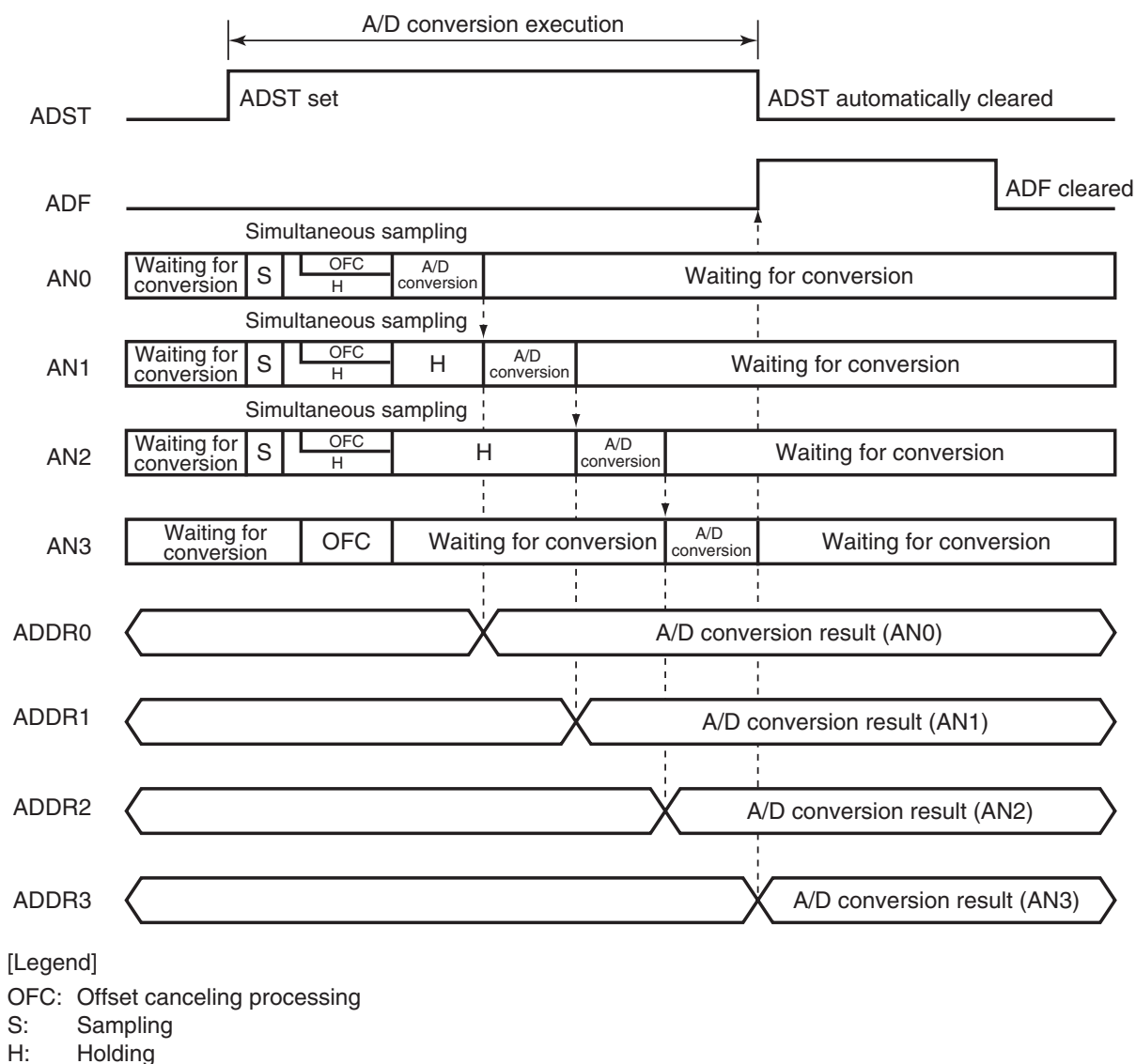
Figure 17.3 Example of A/D_0 Converter Operation (Single-Cycle Scan Mode)
