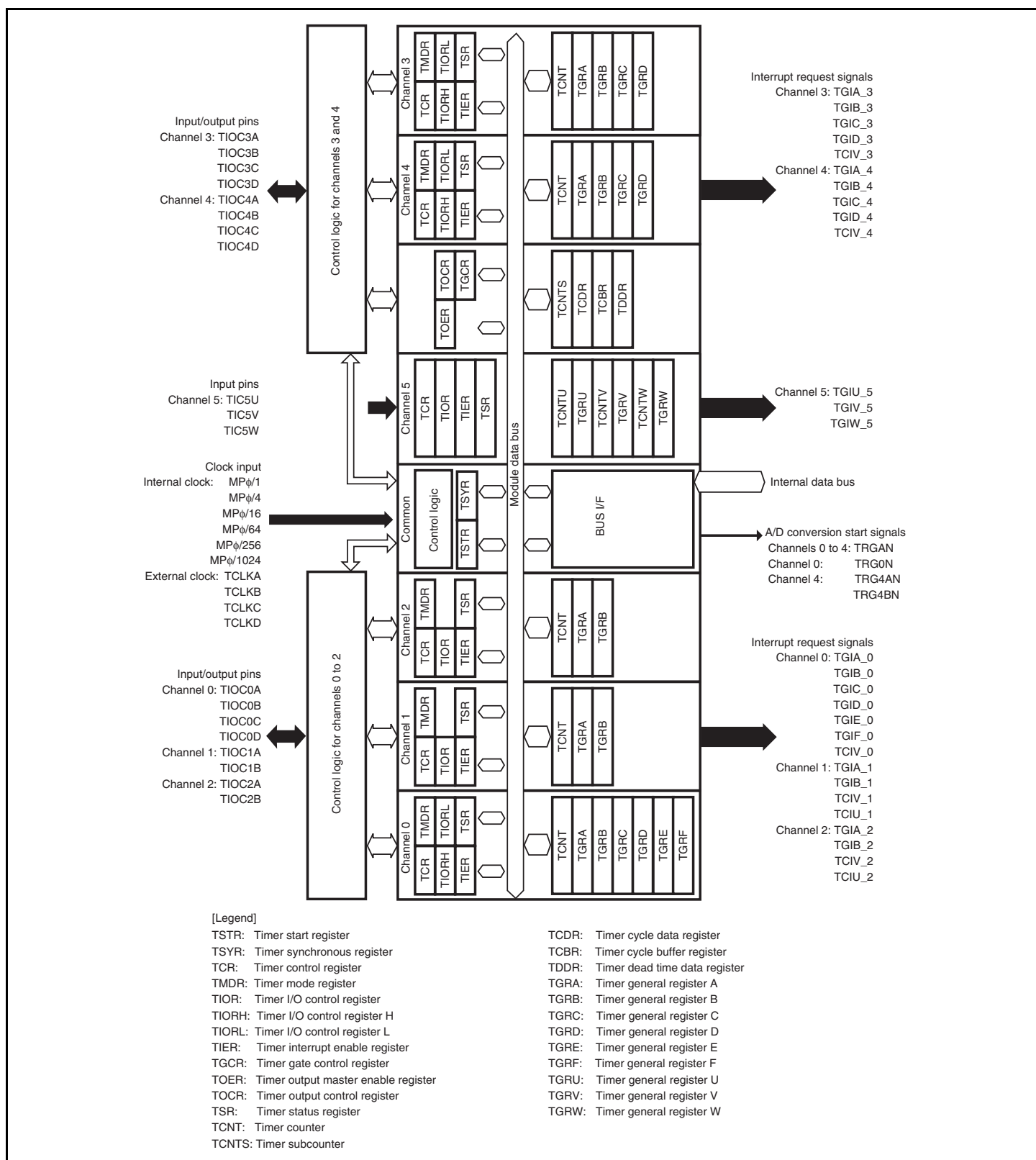
Figure 10.1 Block Diagram of MTU2
