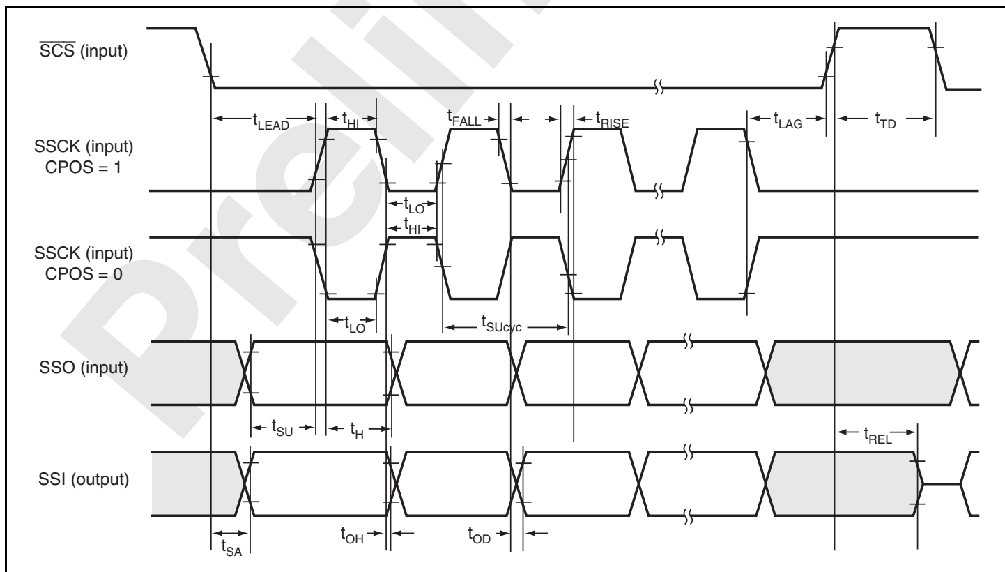
Figure 26.25 SSU Timing (Slave, CPHS = 1)
