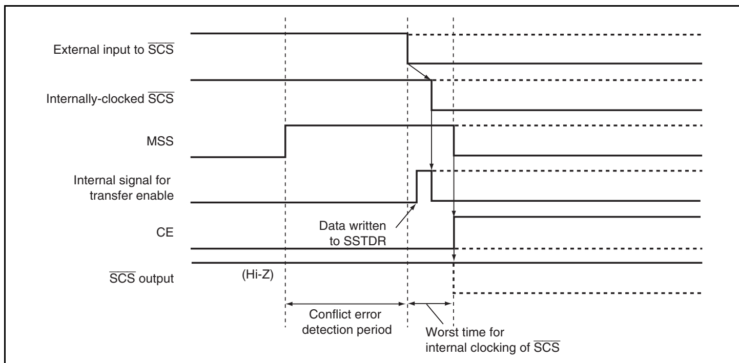
Figure 15.10 Conflict Error Detection Timing (Before Transfer)
