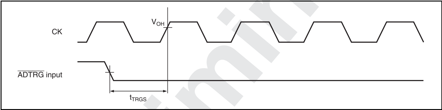
Figure 26.31 External Trigger Input Timing
