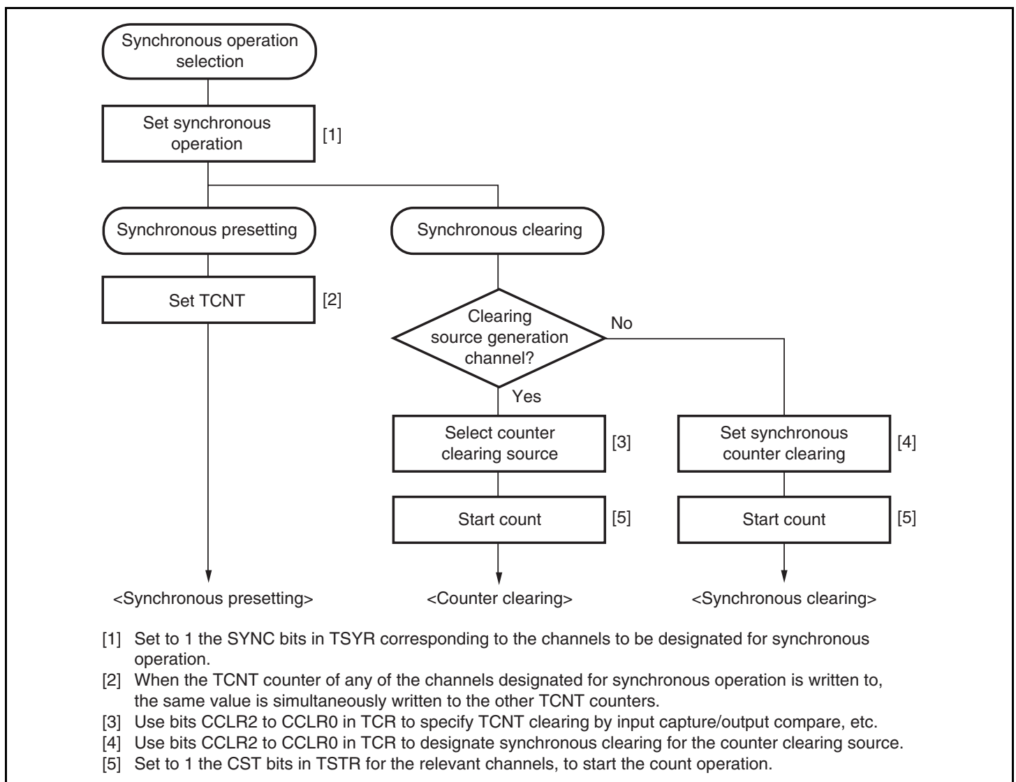
Figure 10.12 Example of Synchronous Operation Setting Procedure
