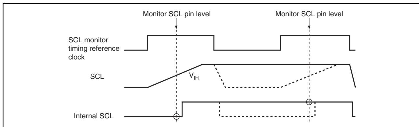
Figure 16.22 The Timing of the Bit Synchronous Circuit
