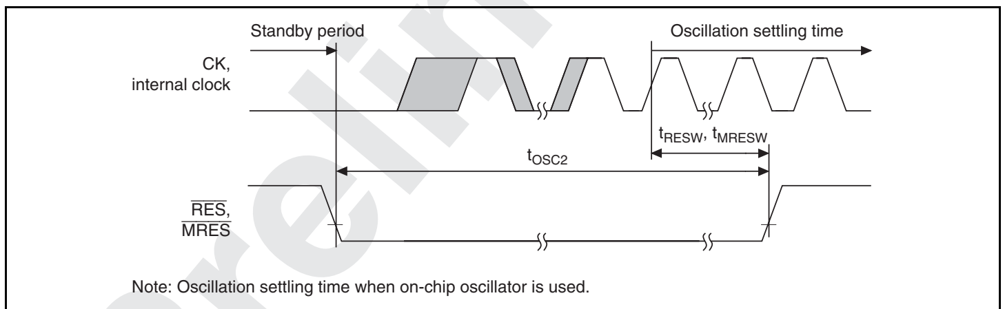
Figure 26.4 Oscillation Settling Timing on Return from Standby (Return by Reset)
