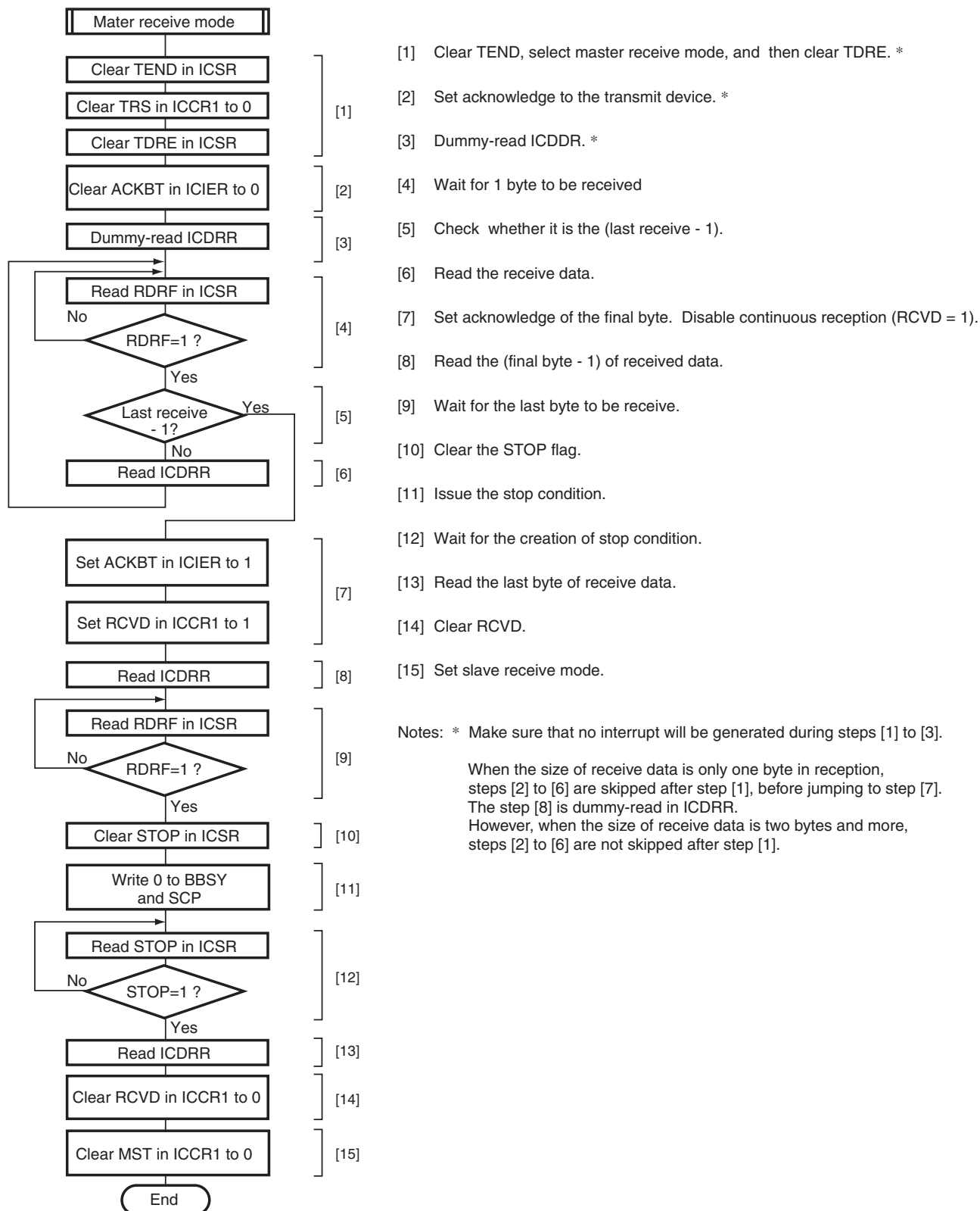
Figure 16.19 Sample Flowchart for Master Receive Mode
