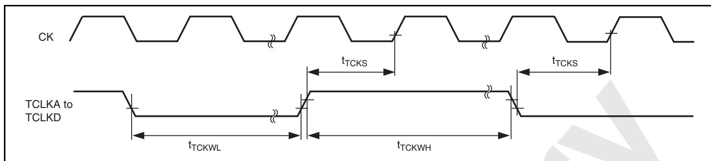
Figure 26.17 MTU2 Clock Input Timing
