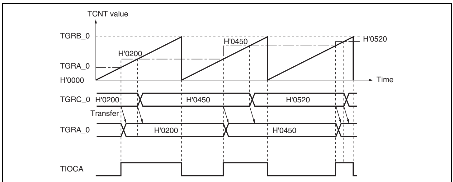
Figure 10.17 Example of Buffer Operation (1)
