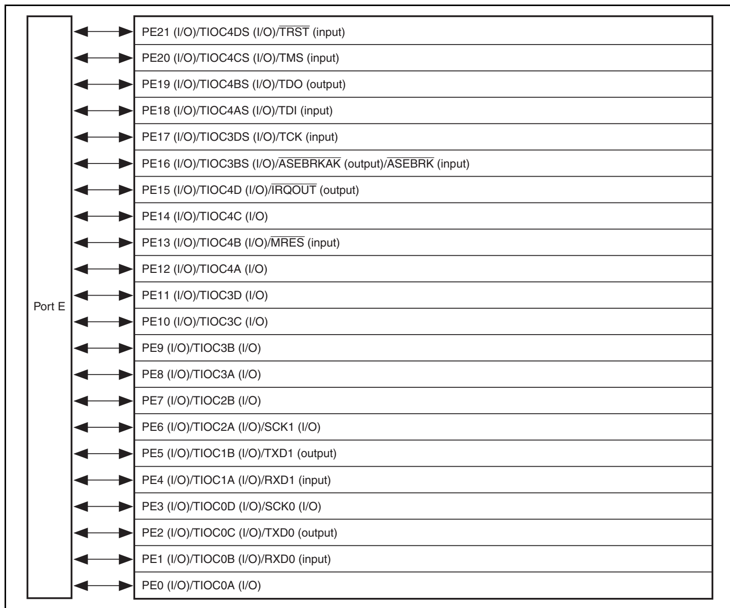
Figure 21.6 Port E (SH7136)
