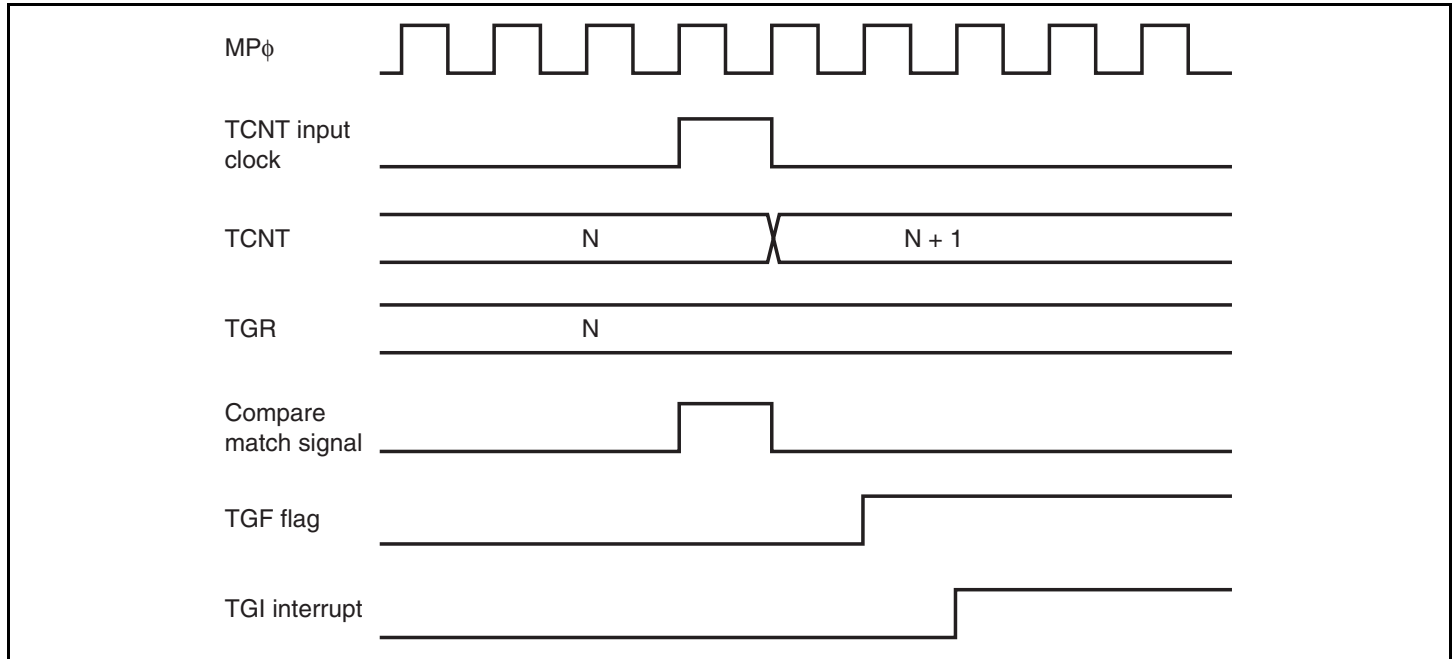
Figure 10.109 TGI Interrupt Timing (Compare Match) (Channels 0 to 4)
