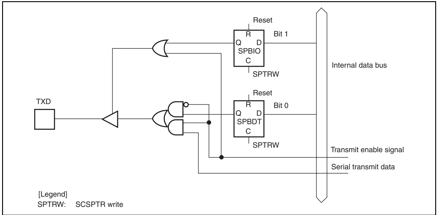
Figure 14.20 SPBIO Bit, SPBDT Bit, and TXD Pin
