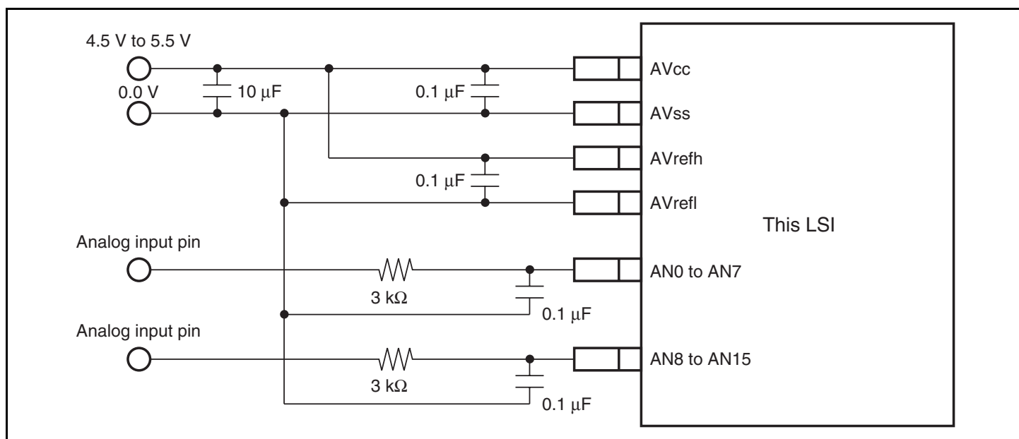
Figure 17.9 Example of Analog Input Pin Protection Circuit
