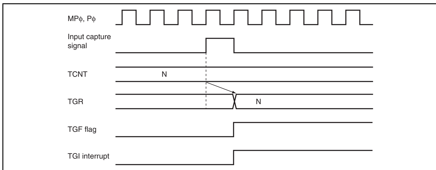
Figure 10.112 TGI Interrupt Timing (Input Capture) (Channel 5)
