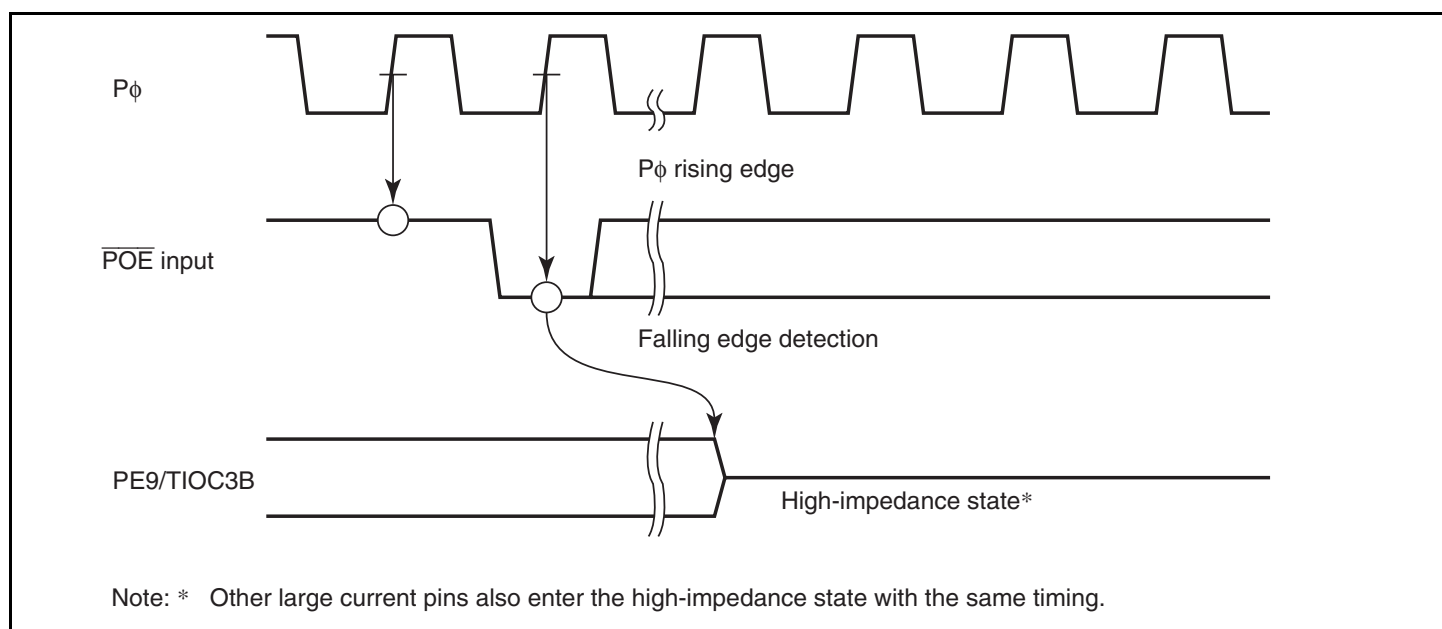
Figure 12.2 Falling Edge Detection
