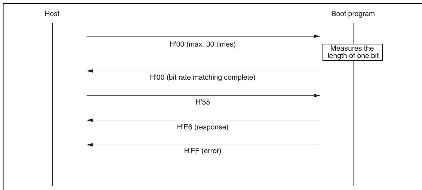
Figure 22.23 Sequence of Bit-Rate Matching
