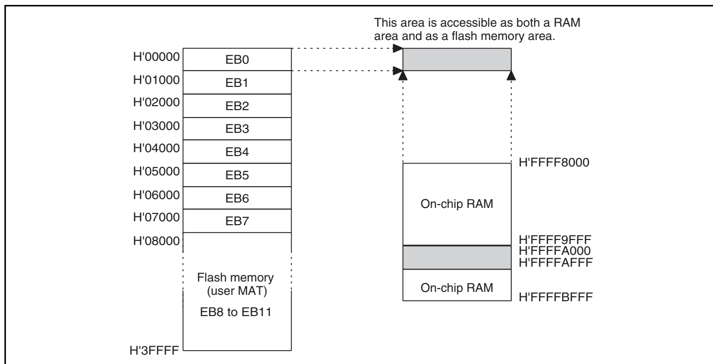
Figure 22.18 Example of Overlapped RAM Operation
