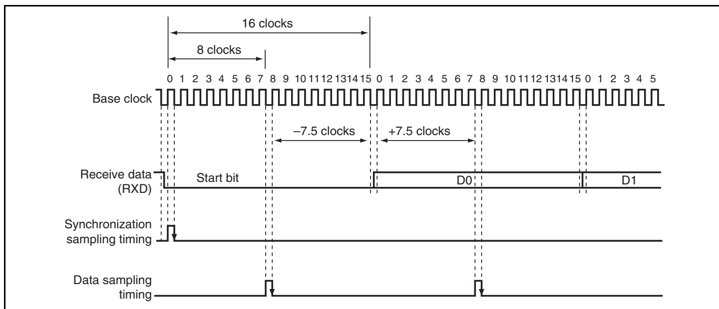
Figure 14.21 Receive Data Sampling Timing in Asynchronous Mode
