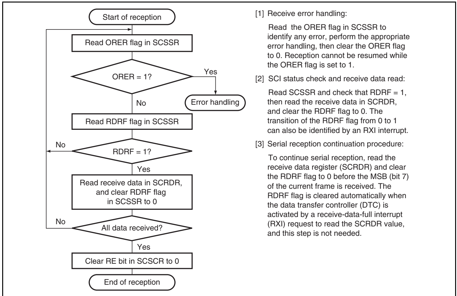
Figure 14.12 Sample Flowchart for Receiving Serial Data (1)
