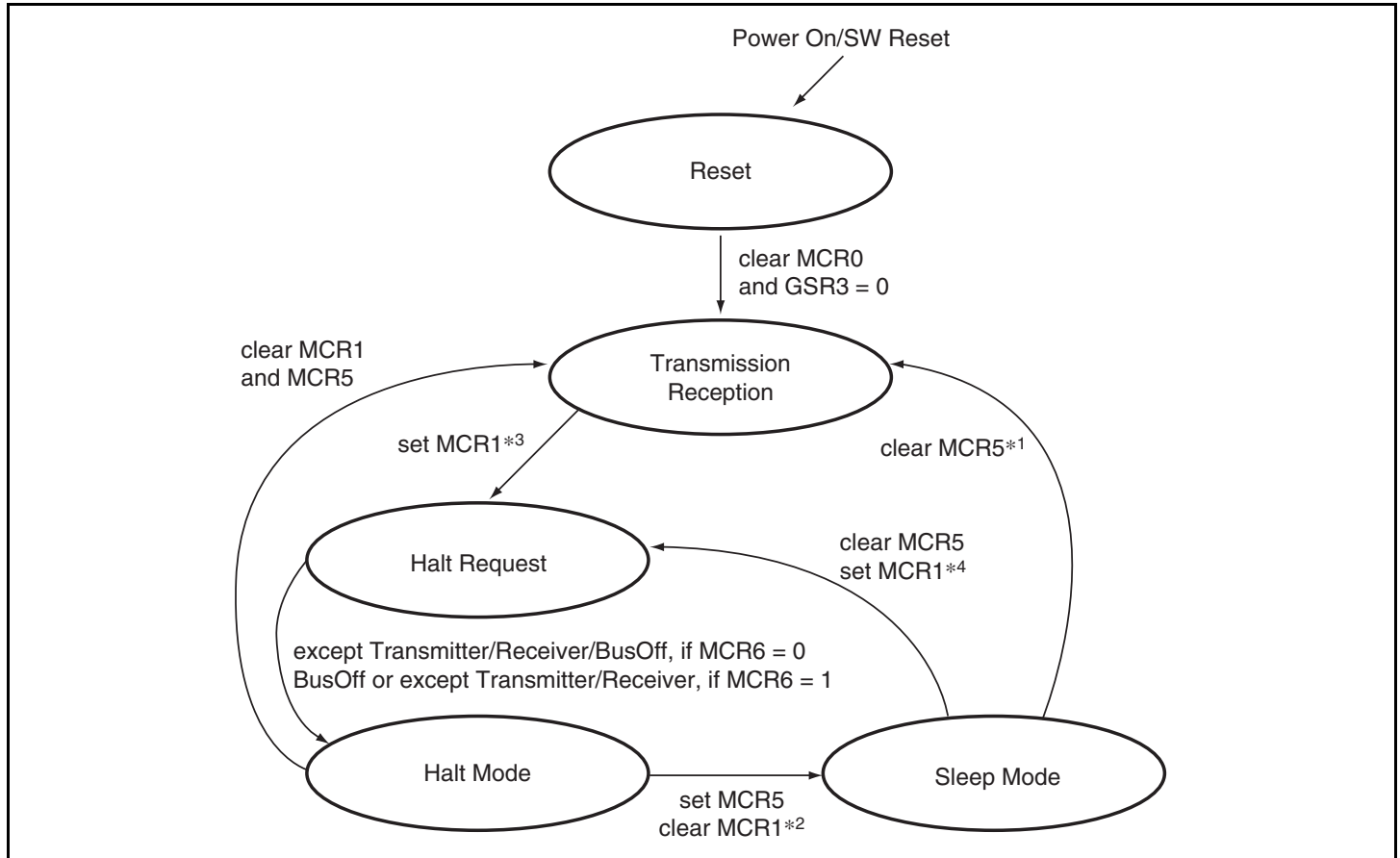
Figure 19.9 Halt Mode / Sleep Mode
