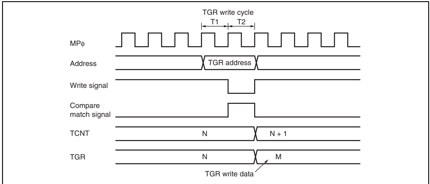
Figure 10.122 Contention between TGR Write and Compare Match
