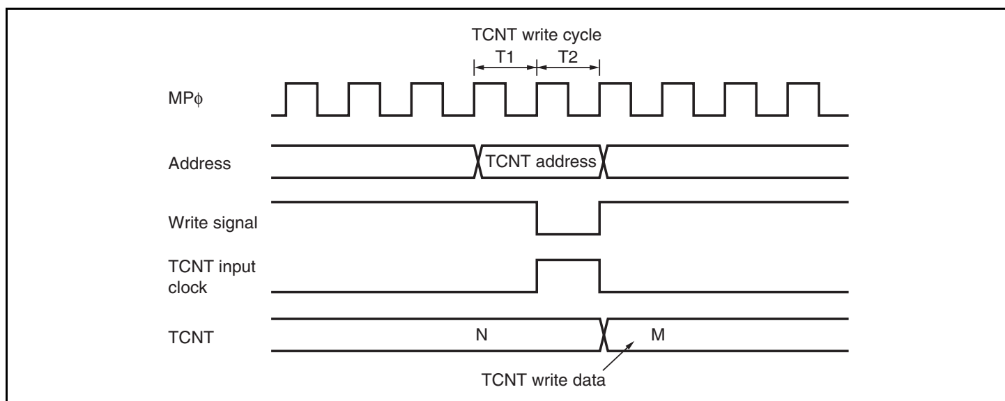
Figure 10.121 Contention between TCNT Write and Increment Operations
