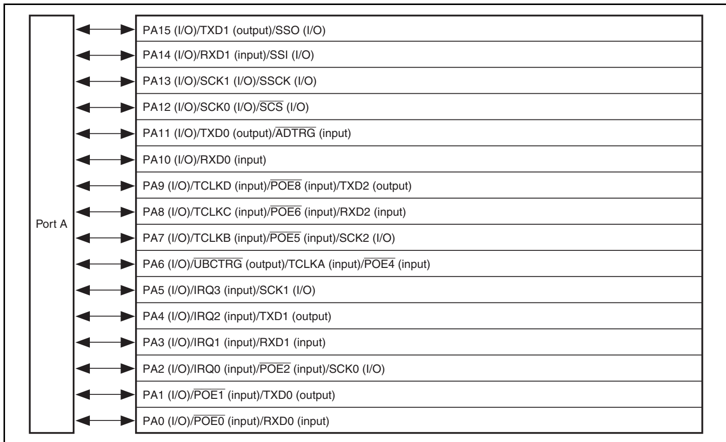
Figure 21.1 Port A (SH7136)
