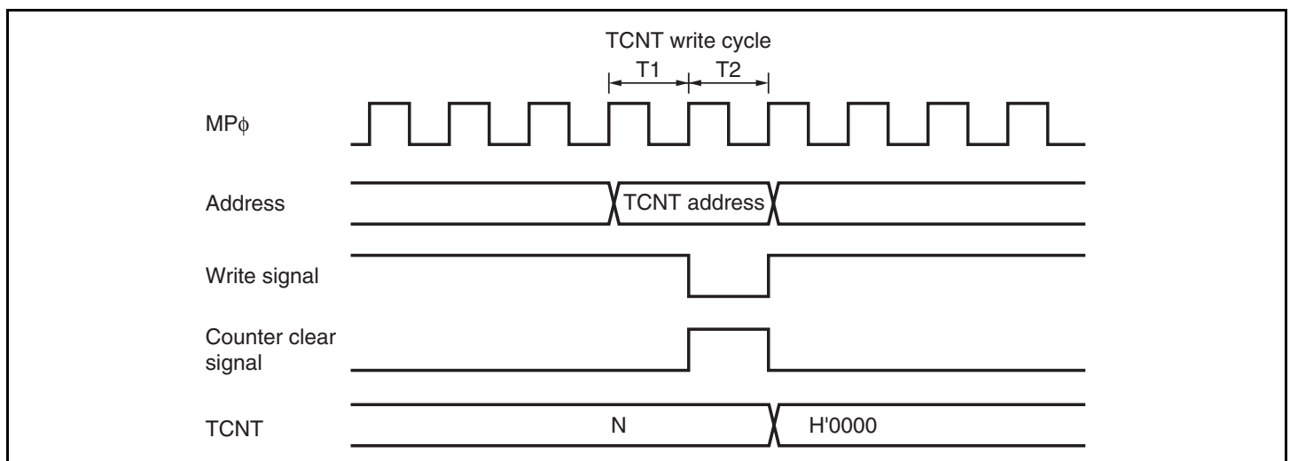
Figure 10.120 Contention between TCNT Write and Clear Operations
