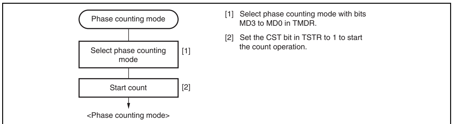
Figure 10.29 Example of Phase Counting Mode Setting Procedure
