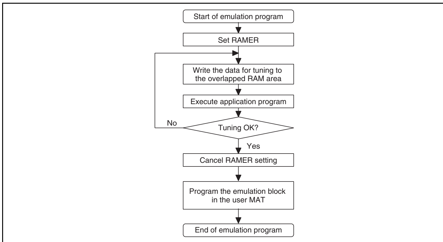
Figure 22.17 Emulation of Flash Memory in RAM
