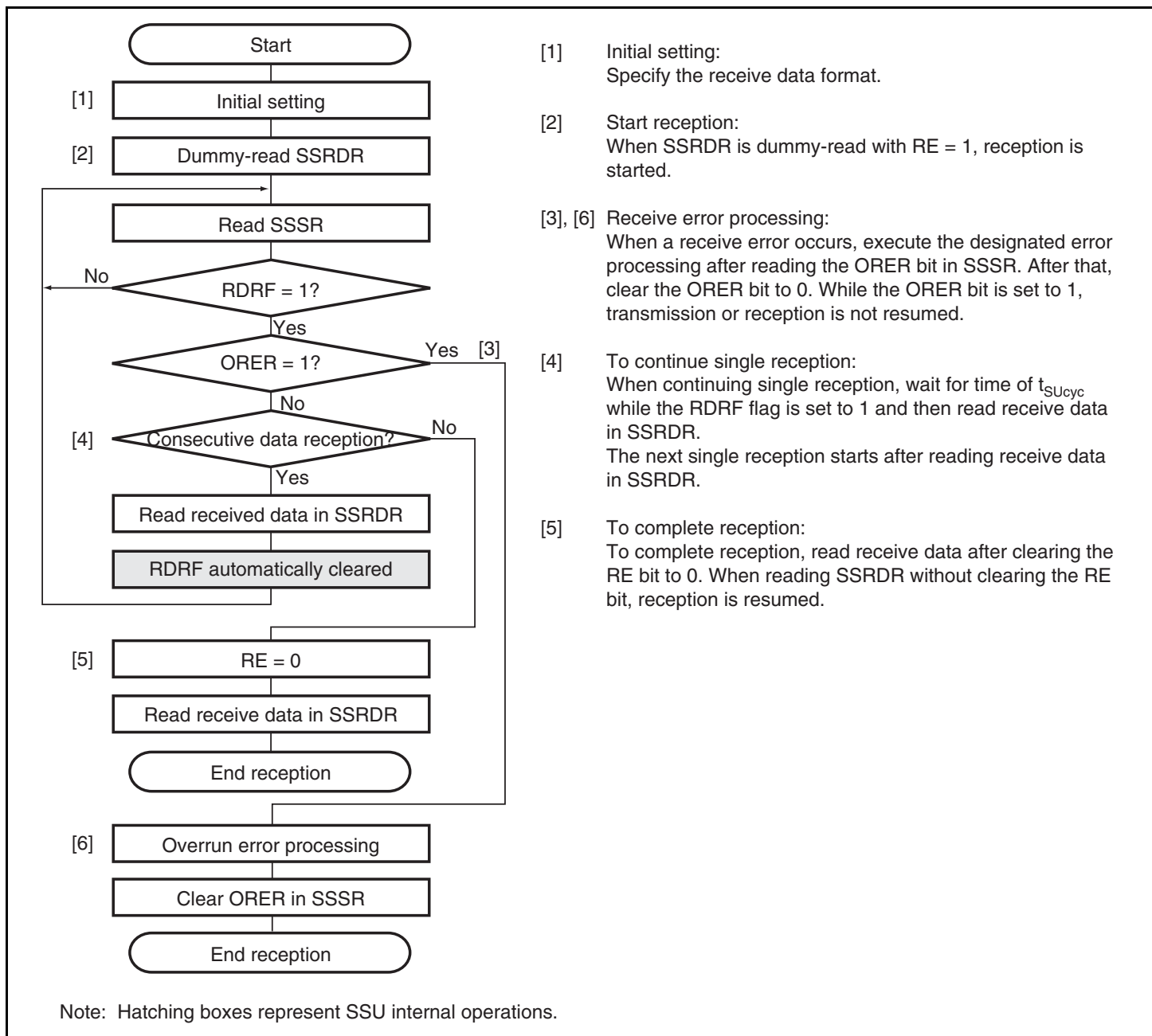
Figure 15.8 Flowchart Example of Data Reception (SSU Mode)
