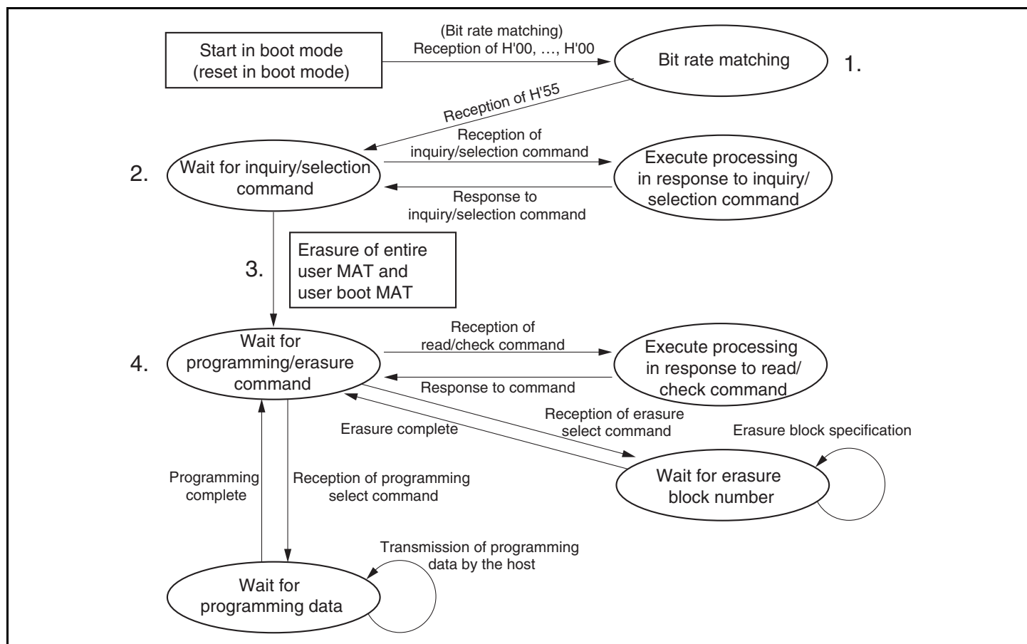
Figure 22.8 State Transitions in Boot Mode
