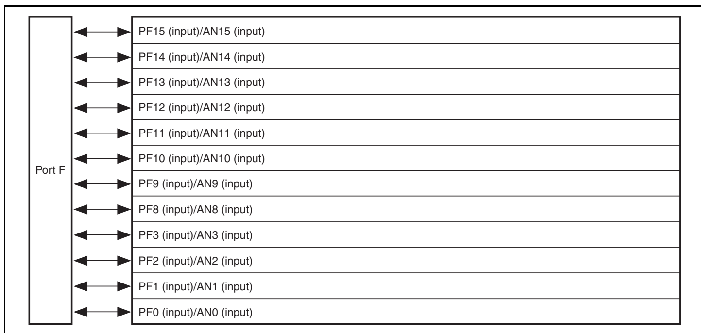
Figure 21.8 Port F (SH7136)
