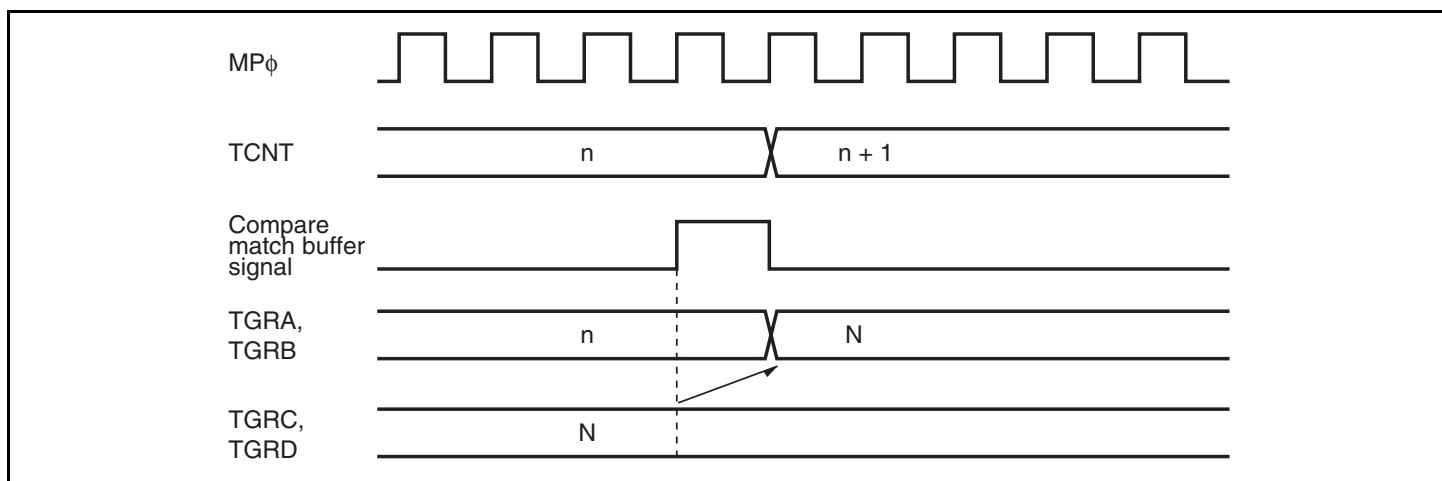
Figure 10.103 Buffer Operation Timing (Compare Match)
