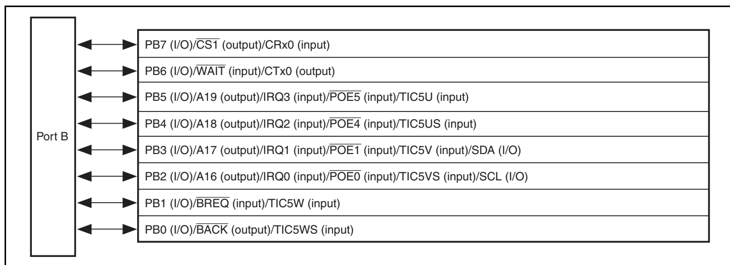
Figure 21.4 Port B (SH7137)
