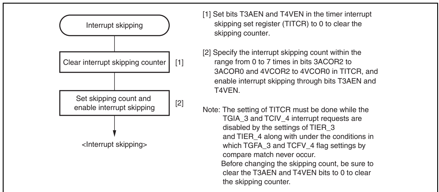
Figure 10.73 Example of Interrupt Skipping Operation Setting Procedure
