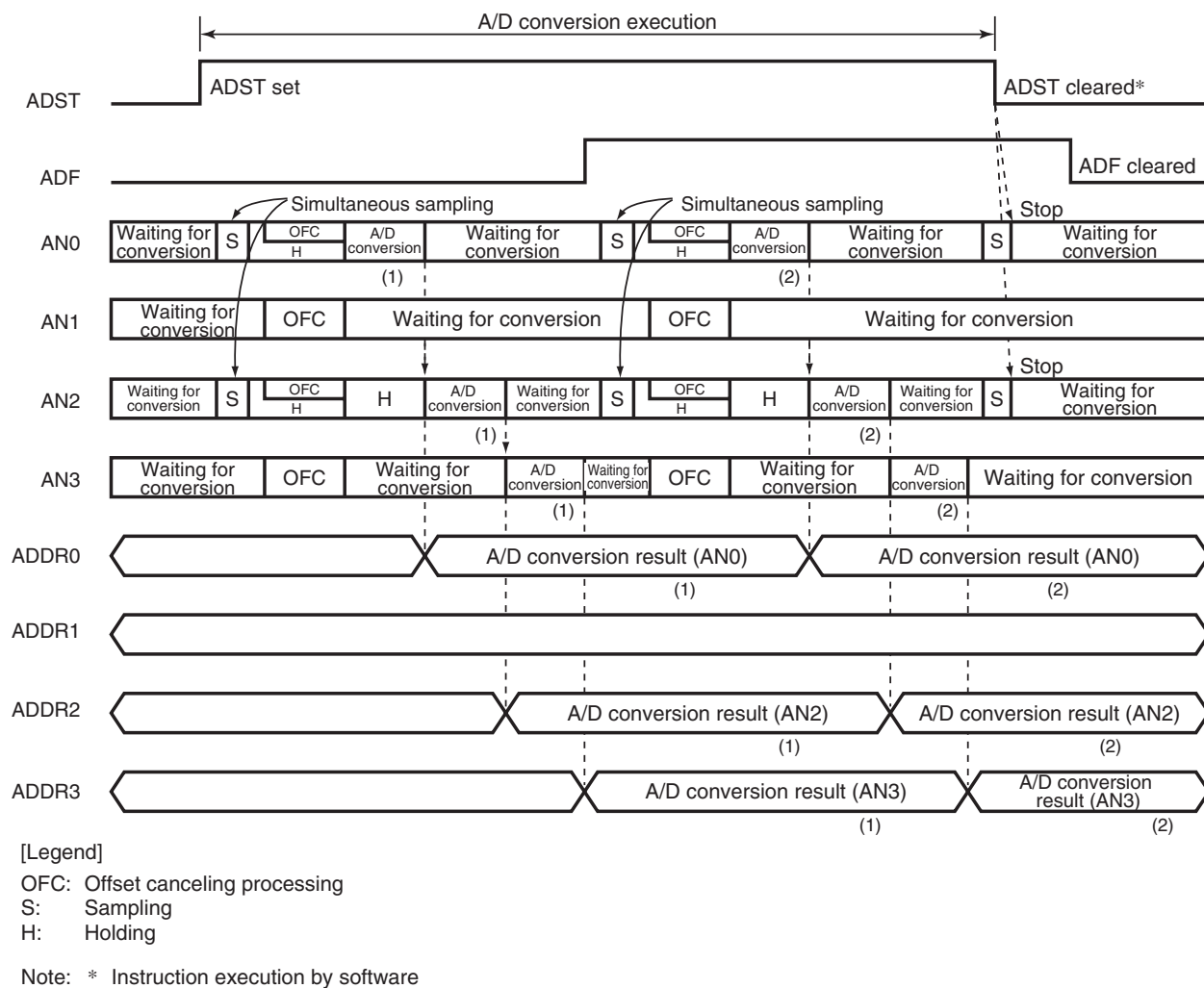
Figure 17.4 Example of A/D_0 Converter Operation (Continuous Scan Mode)
