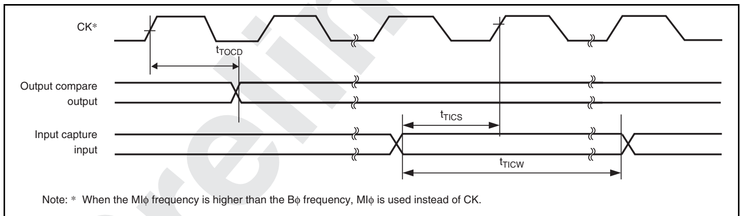
Figure 26.18 MTU2S Input/Output Timing
