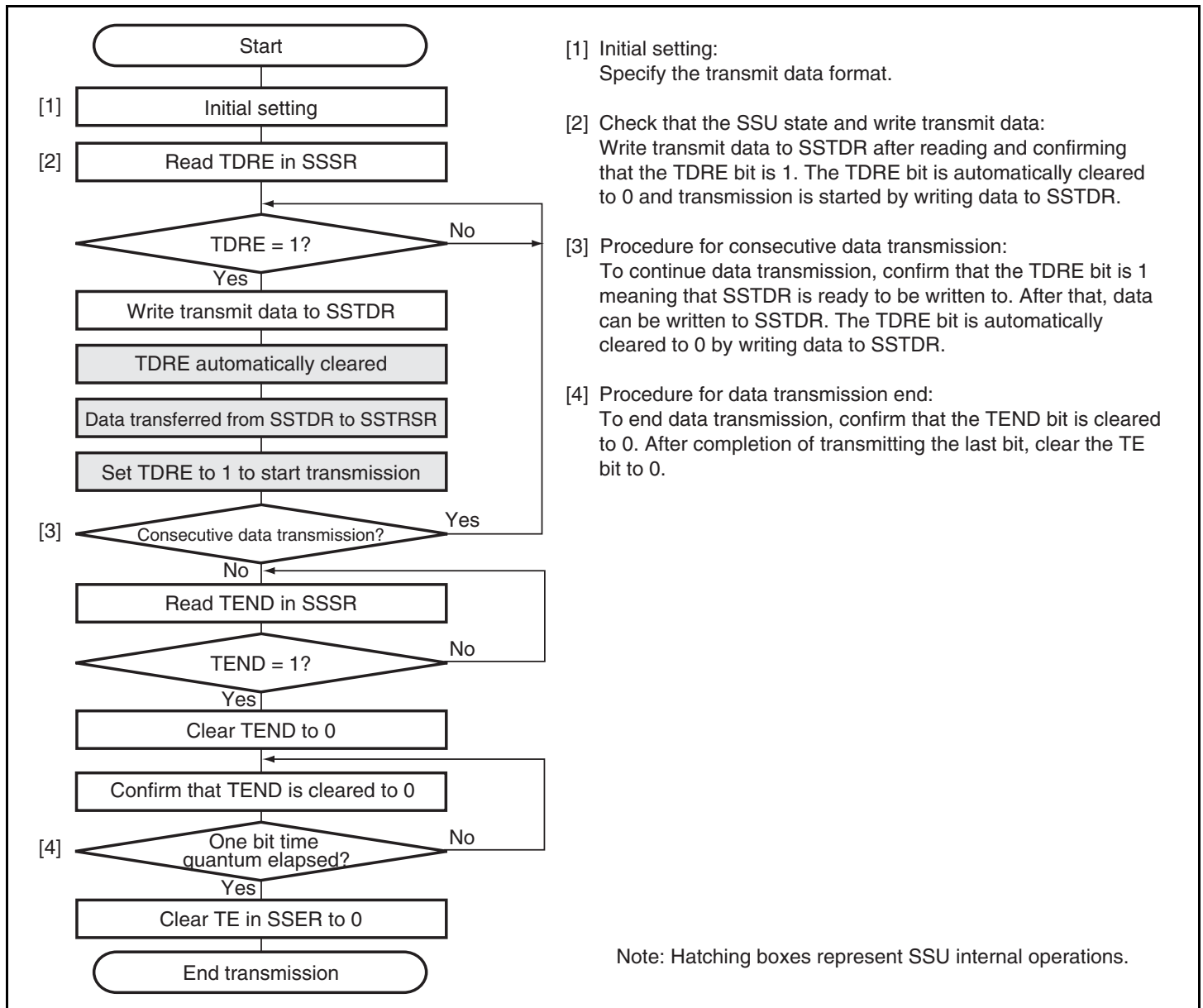
Figure 15.6 Flowchart Example of Data Transmission (SSU Mode)
