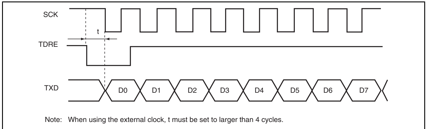
Figure 14.22 Example of Clock Synchronous Transfer Using DTC
