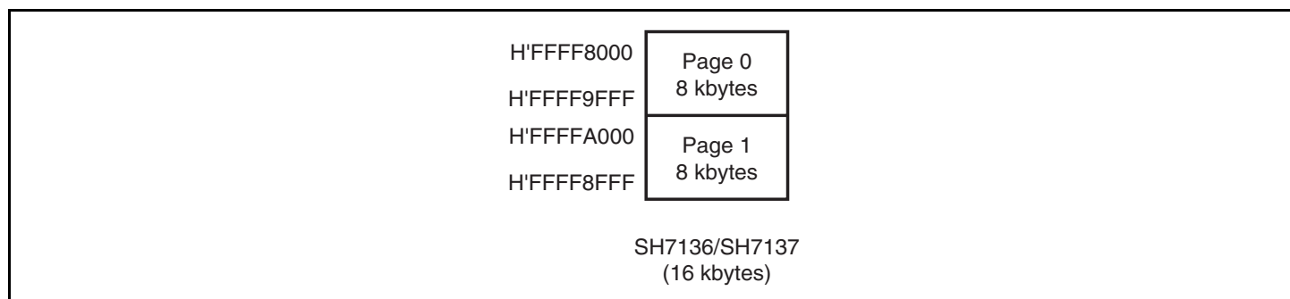
Figure 23.1 On-chip RAM Addresses
