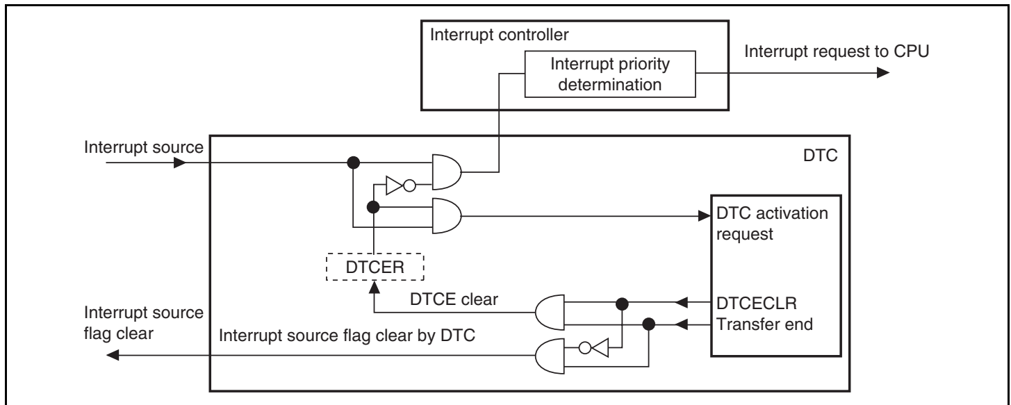
Figure 6.6 On-Chip Module Interrupt Control Block Diagram
