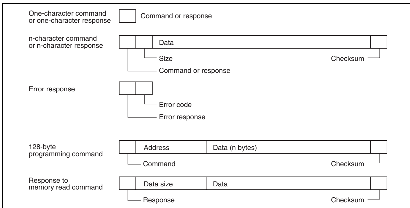
Figure 22.24 Formats in the Communications Protocol
