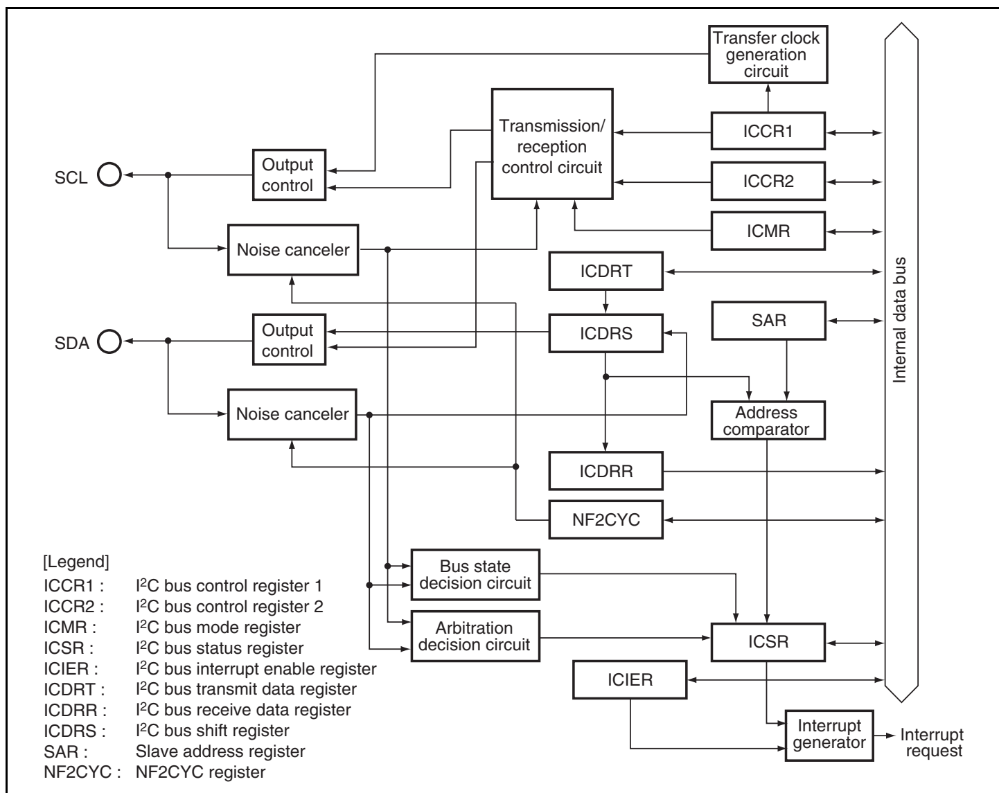
Figure 16.1 Block Diagram of I 2 C Bus Interface 2
