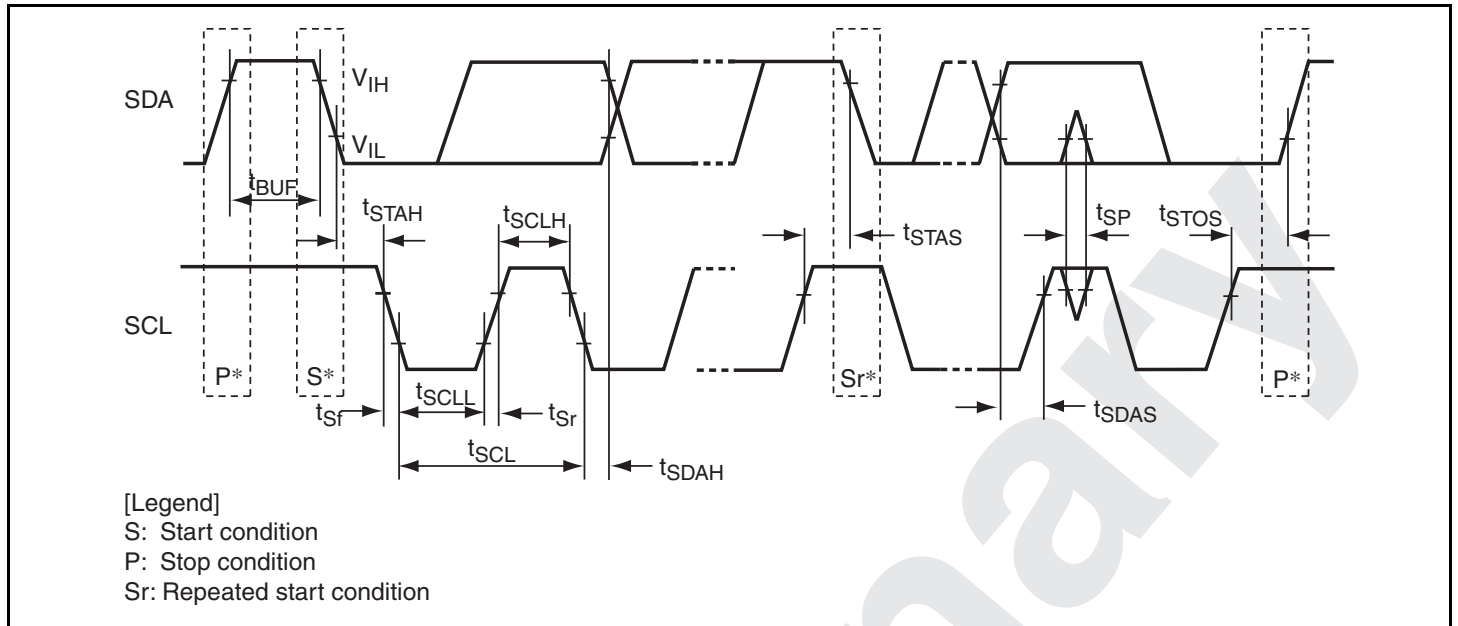
Figure 26.29 I²C2 Input/Output Timing
