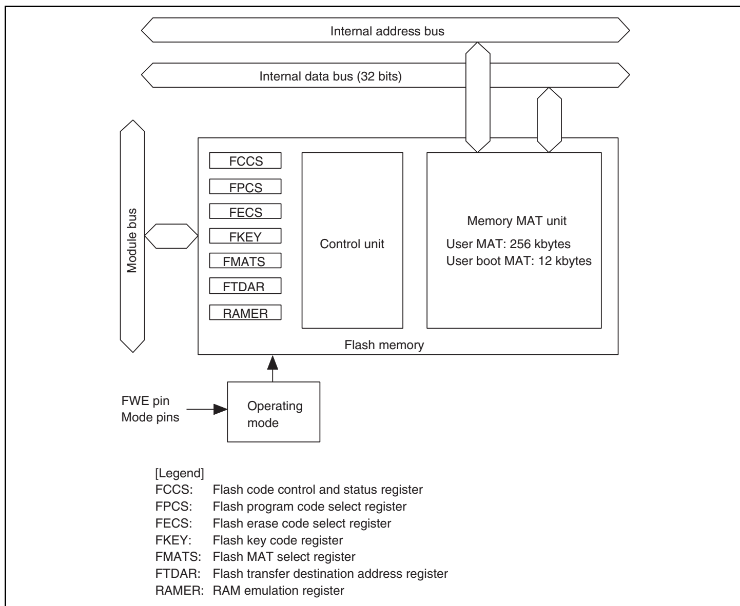
Figure 22.1 Block Diagram of Flash Memory
