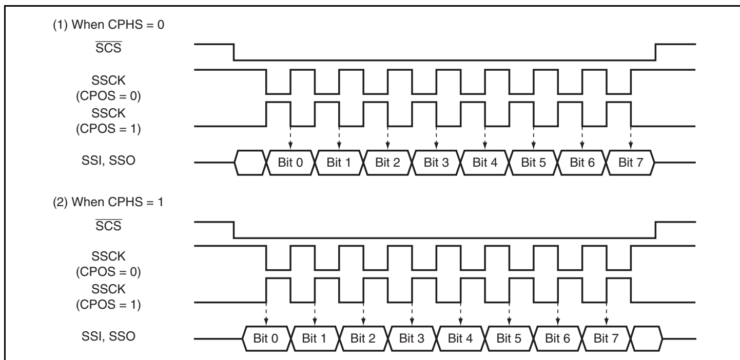
Figure 15.2 Relationship of Clock Phase, Polarity, and Data
