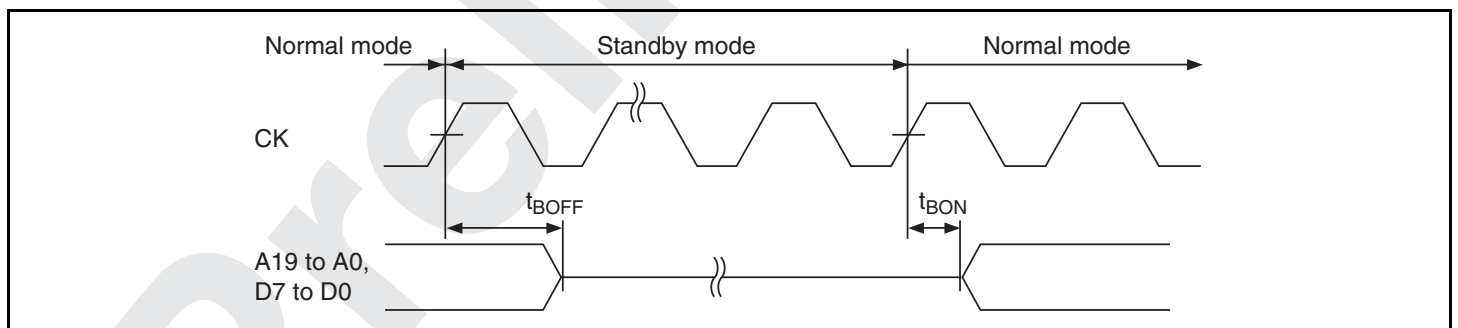
Figure 26.10 Pin Driving Timing in Standby Mode
