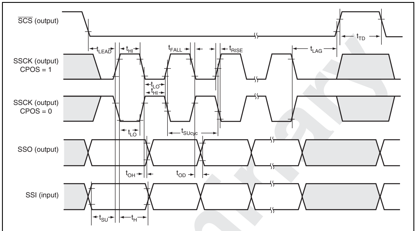
Figure 26.23 SSU Timing (Master, CPHS = 1)
