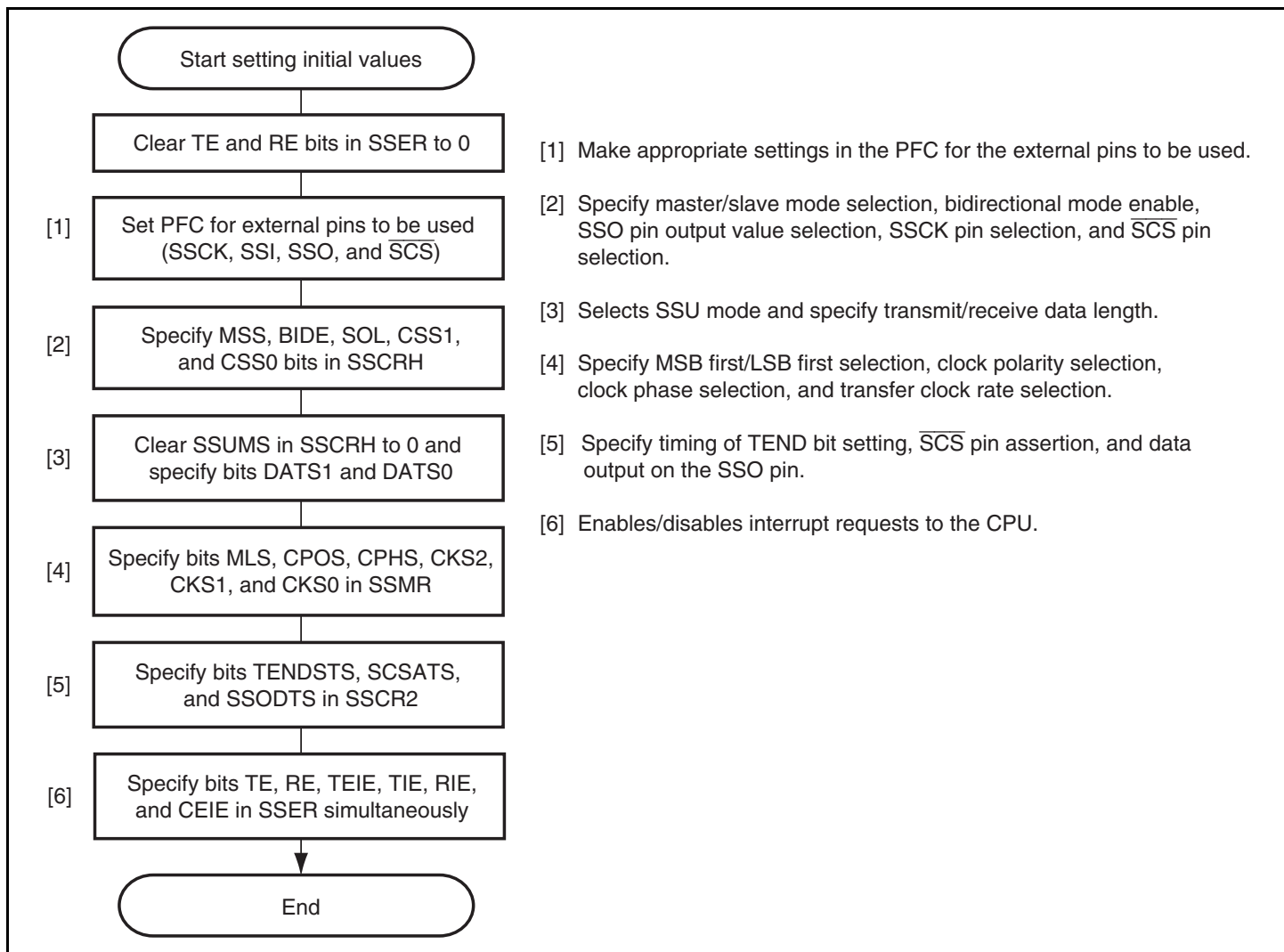
Figure 15.4 Example of Initial Settings in SSU Mode
