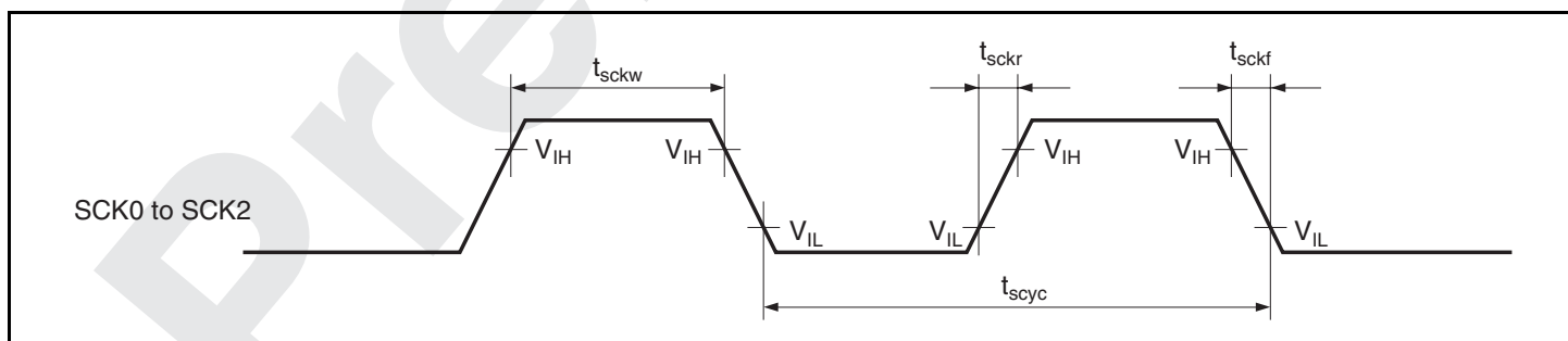
Figure 26.21 Input Clock Timing
