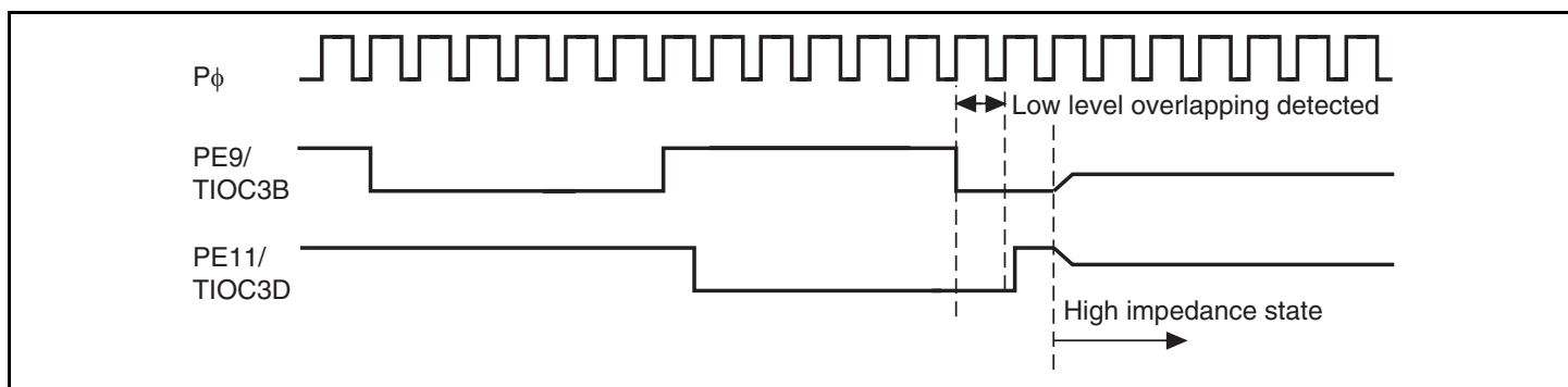
Figure 12.4 Output-Level Compare Operation
