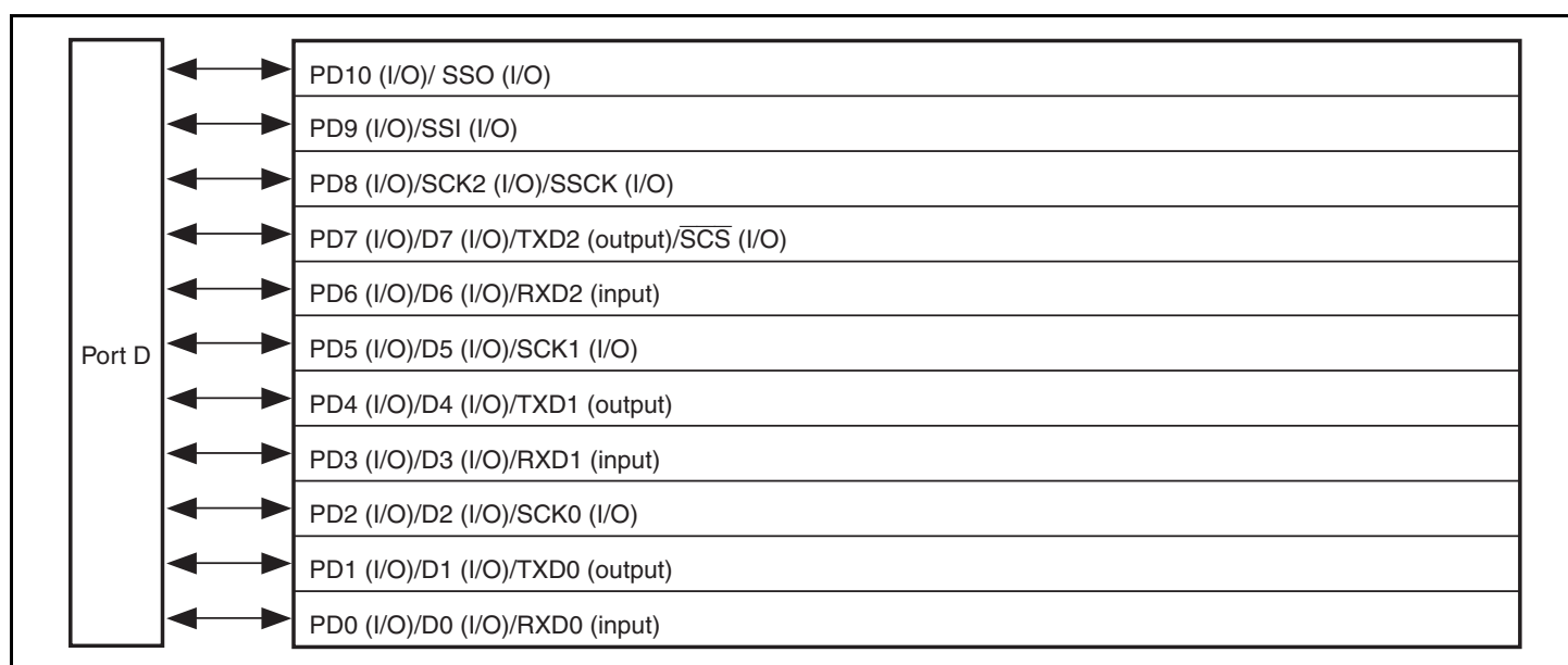
Figure 21.5 Port D
