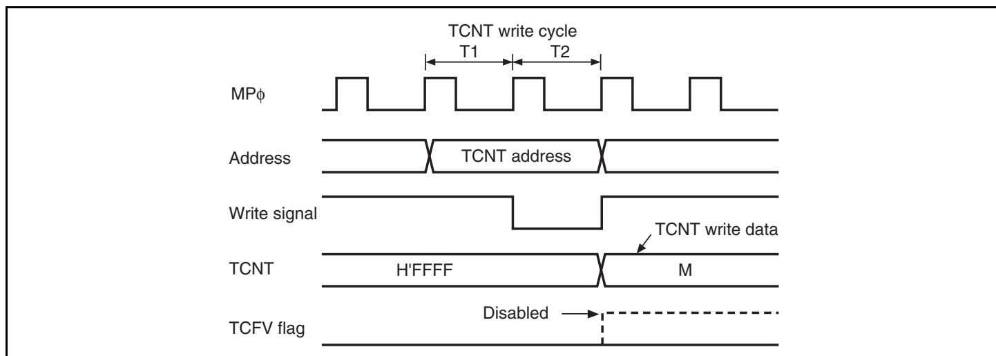
Figure 10.135 Contention between TCNT Write and Overflow
