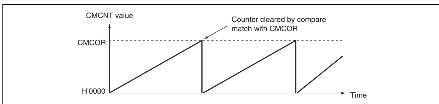
Figure 18.2 Counter Operation
