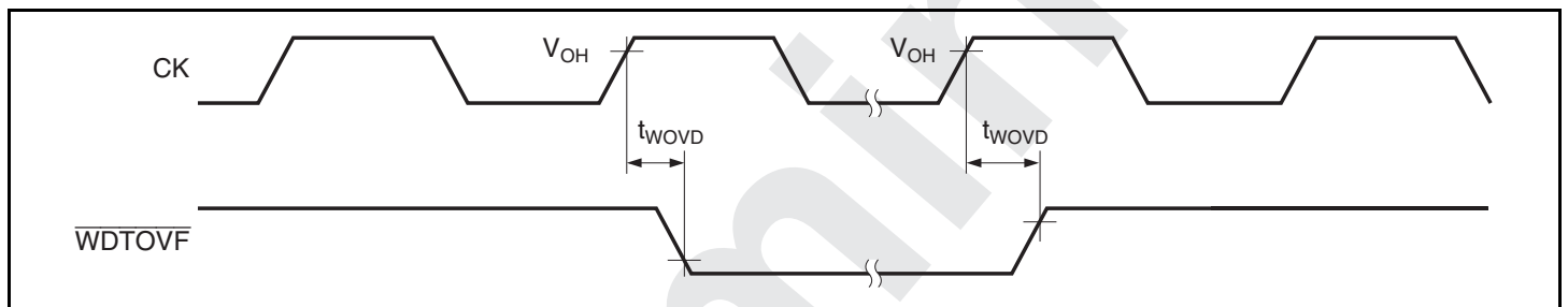
Figure 26.20 WDT Timing
