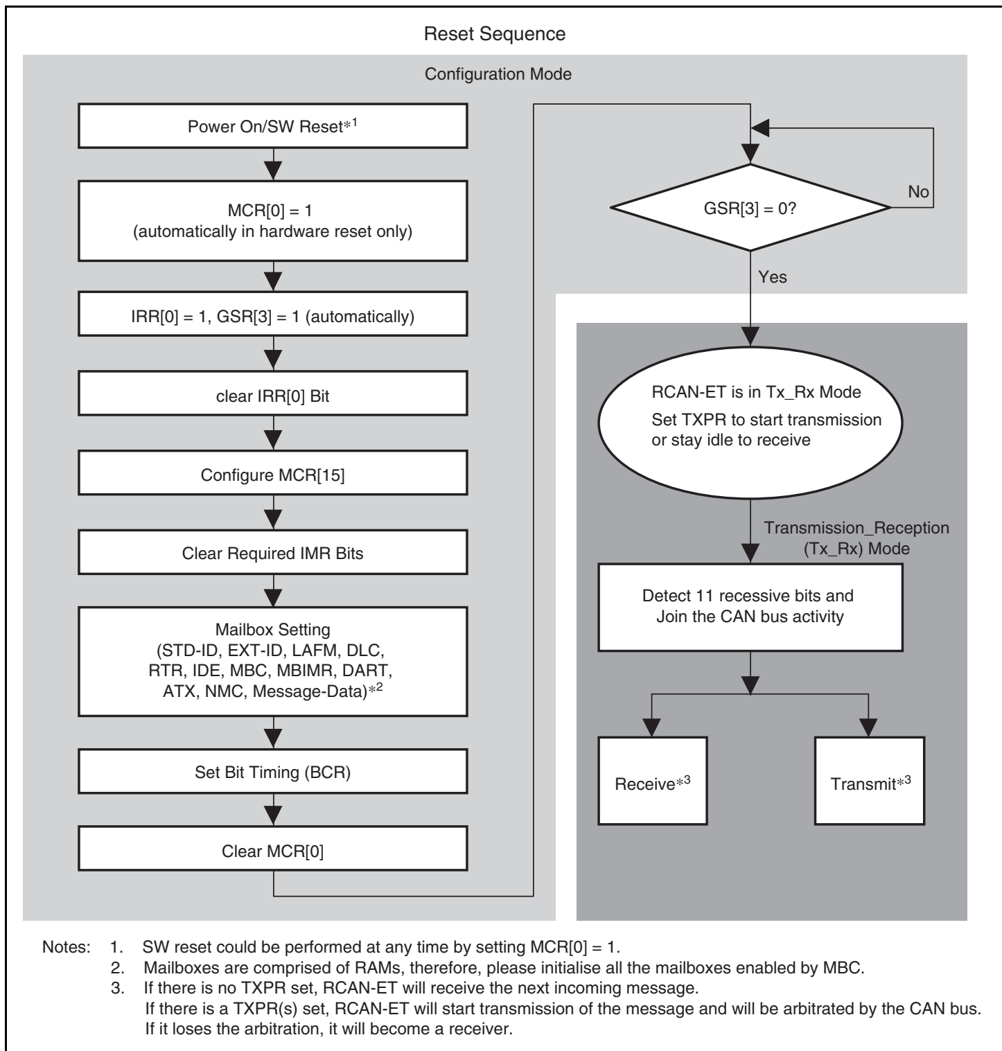
Figure 19.8 Reset Sequence
