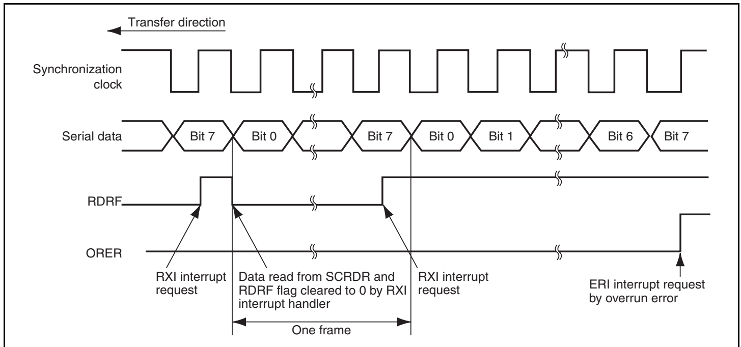
Figure 14.13 Example of SCI Receive Operation
