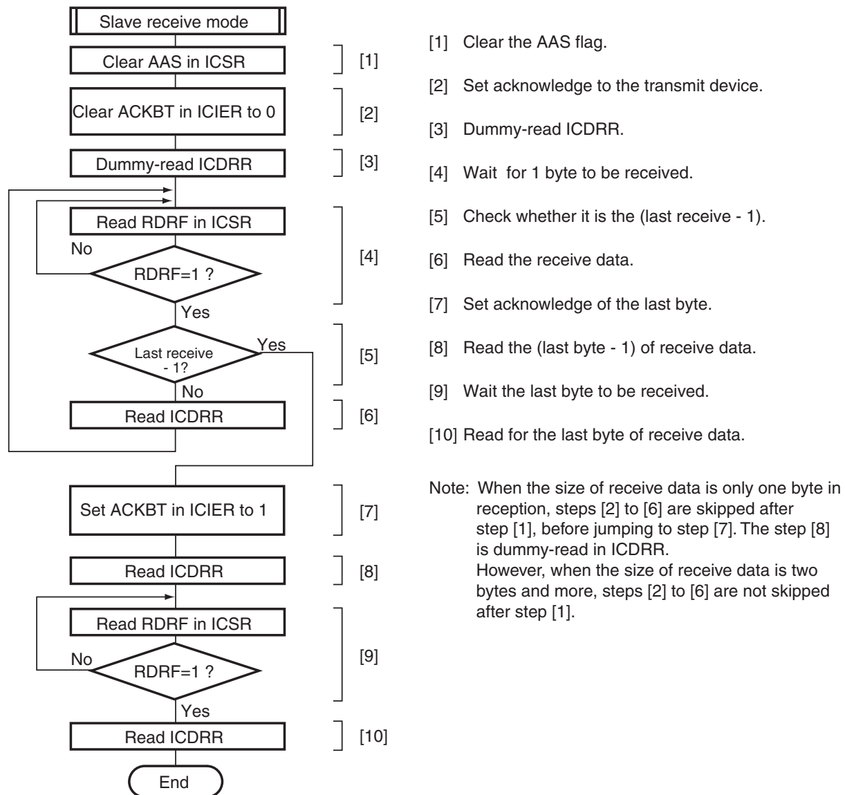
Figure 16.21 Sample Flowchart for Slave Receive Mode
