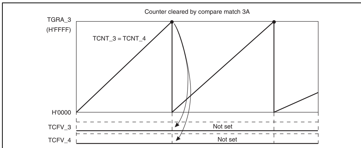
Figure 10.133 Reset Synchronous PWM Mode Overflow Flag
