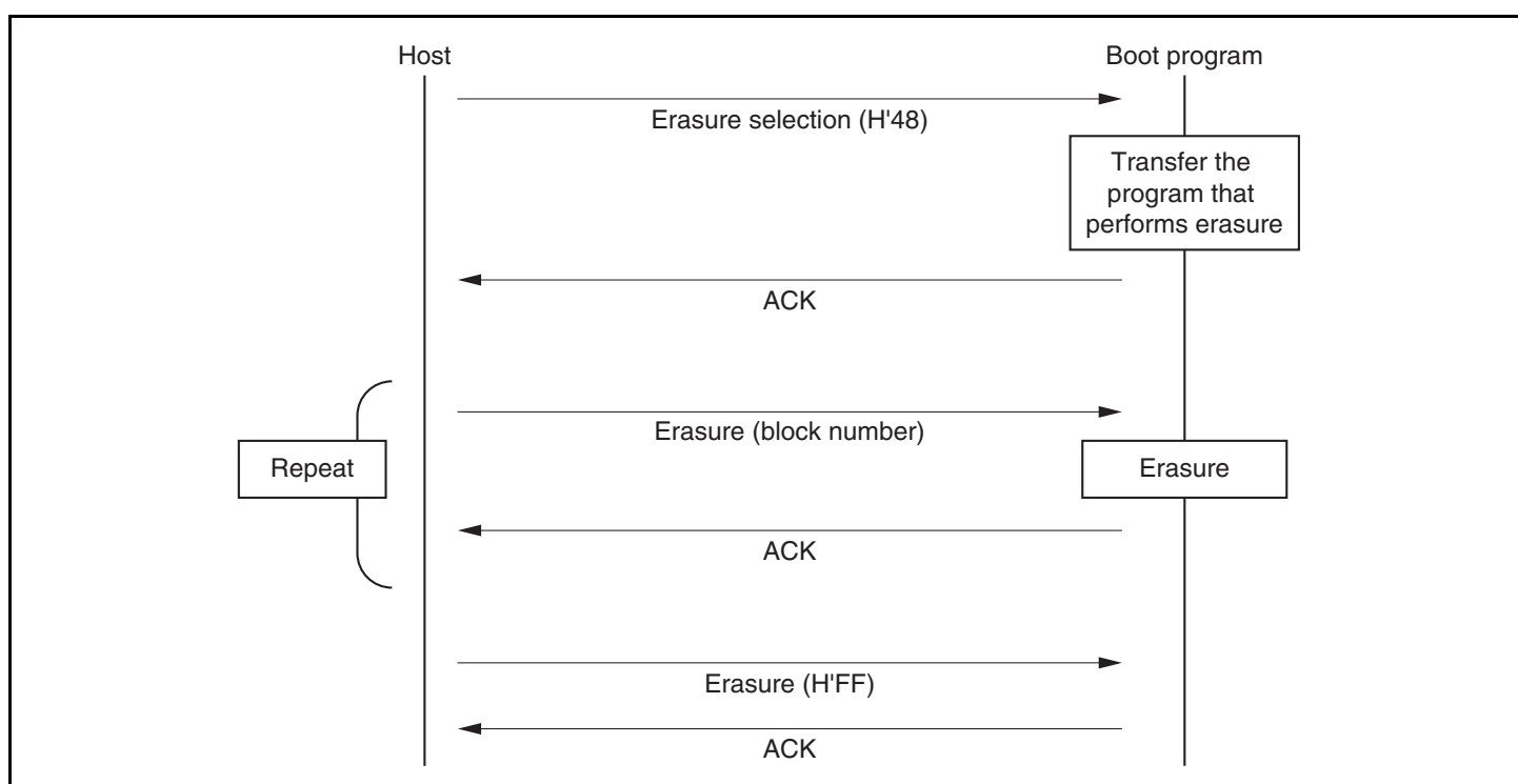
Figure 22.27 Sequence of Erasure
