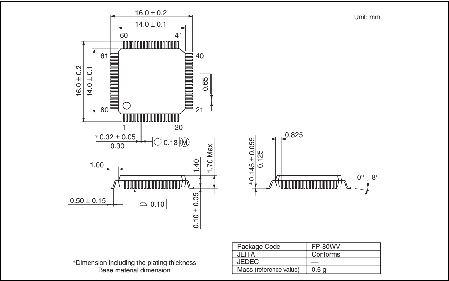
Figure D.1 FP-80WV
