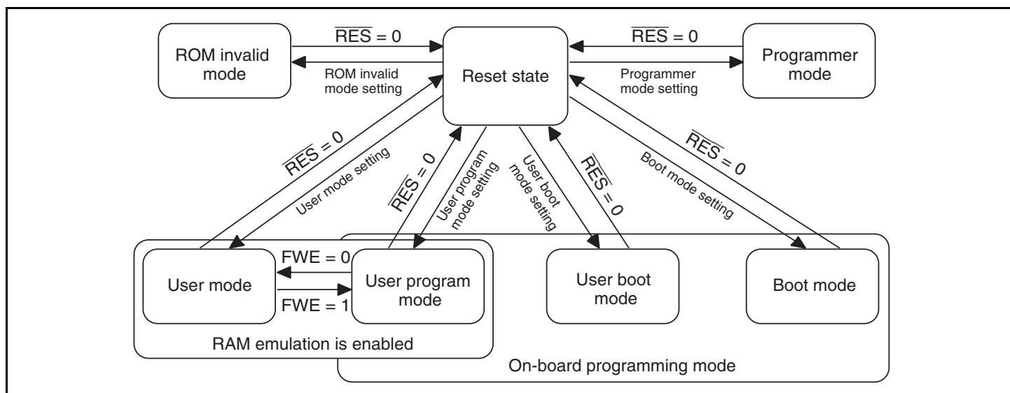
Figure 22.2 Mode Transition of Flash Memory
