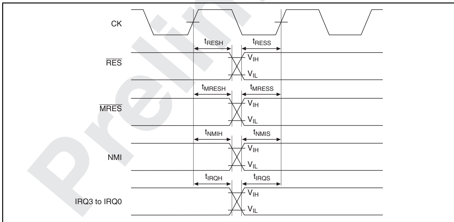
Figure 26.7 Interrupt Signal Input Timing
