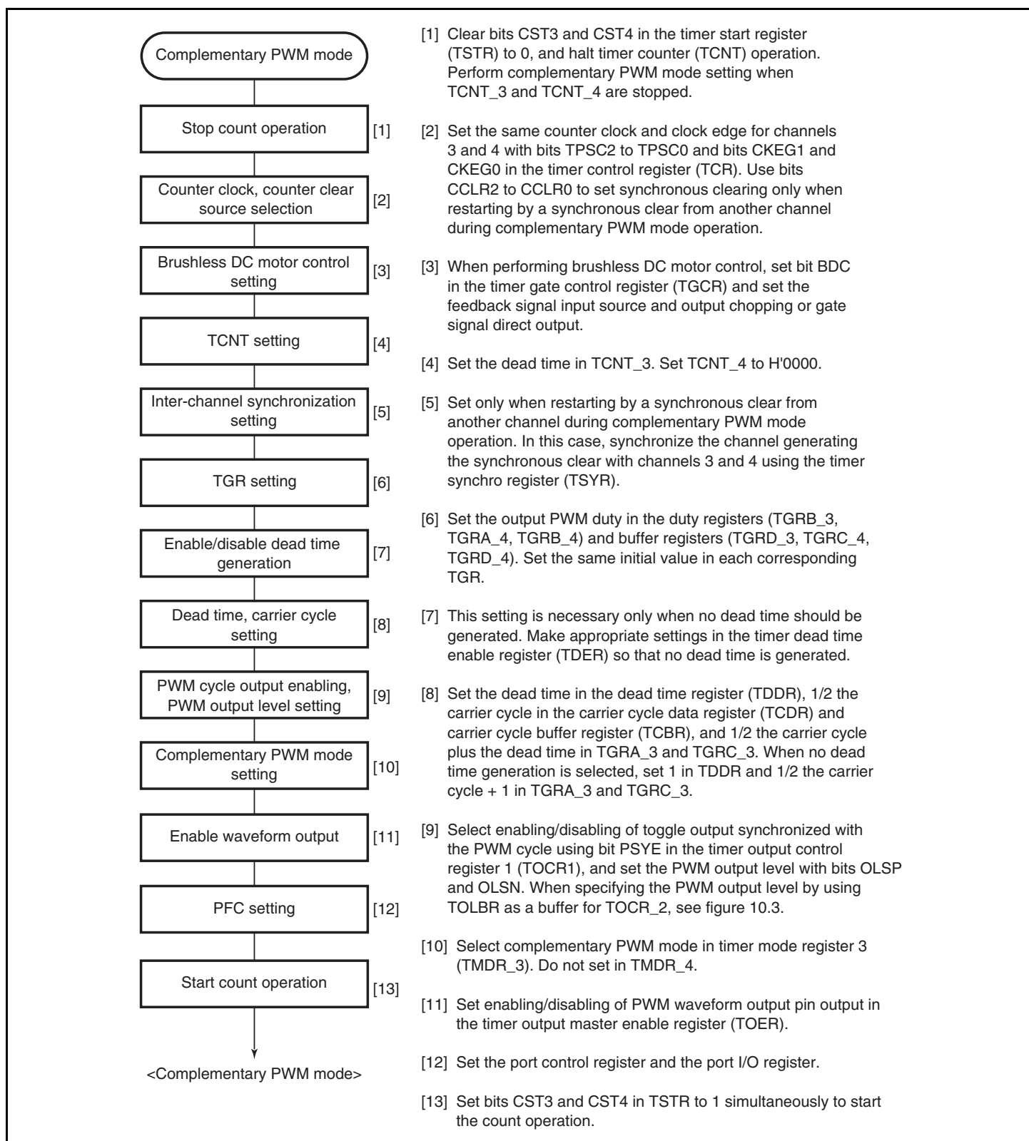
Figure 10.38 Example of Complementary PWM Mode Setting Procedure
