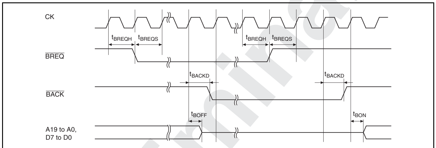
Figure 26.9 Bus Release Timing
