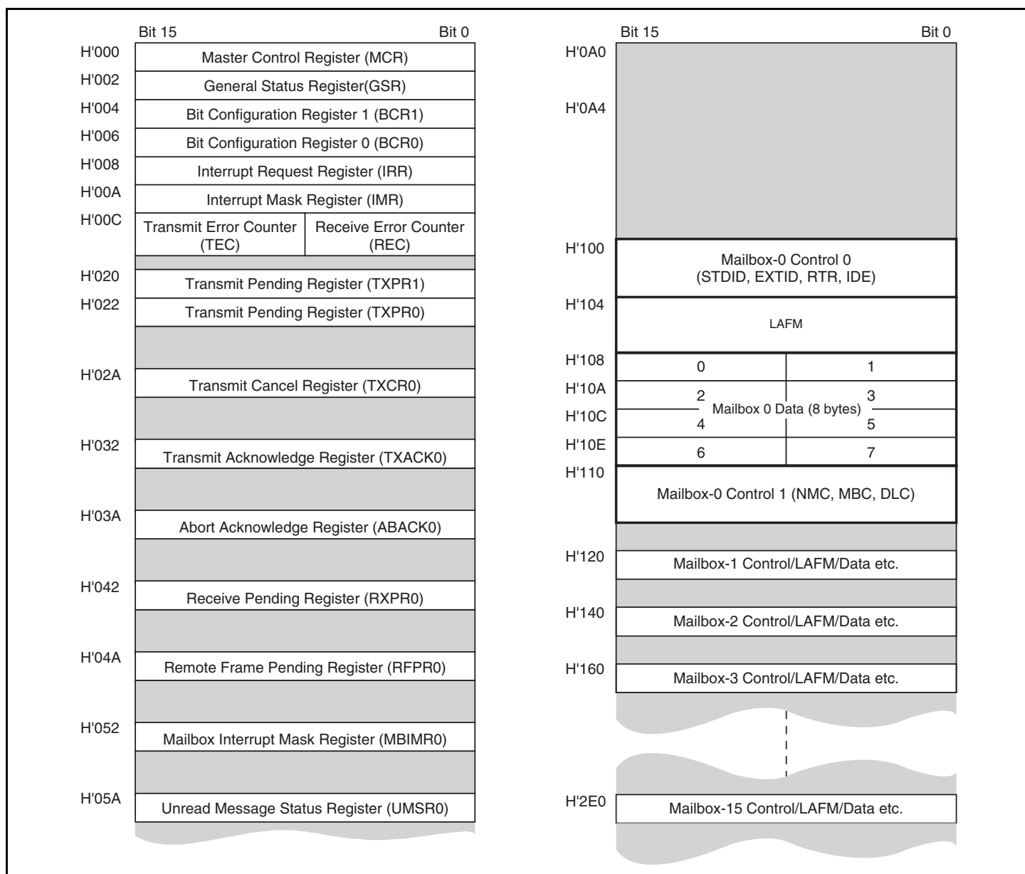
Figure 19.2 RCAN-ET Memory Map
