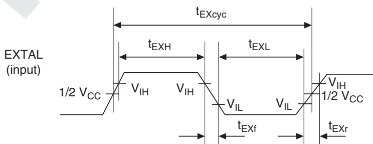
Figure 26.1 EXTAL Clock Input Timing
