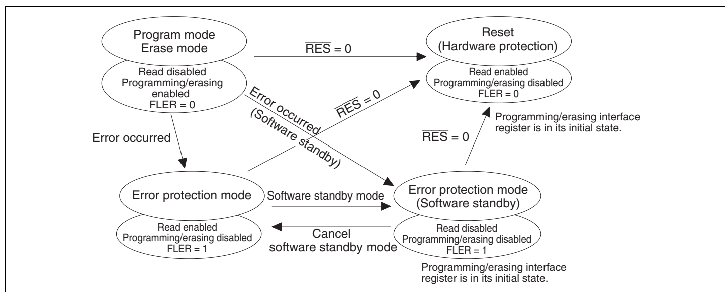
Figure 22.16 Transitions to and from Error Protection State
