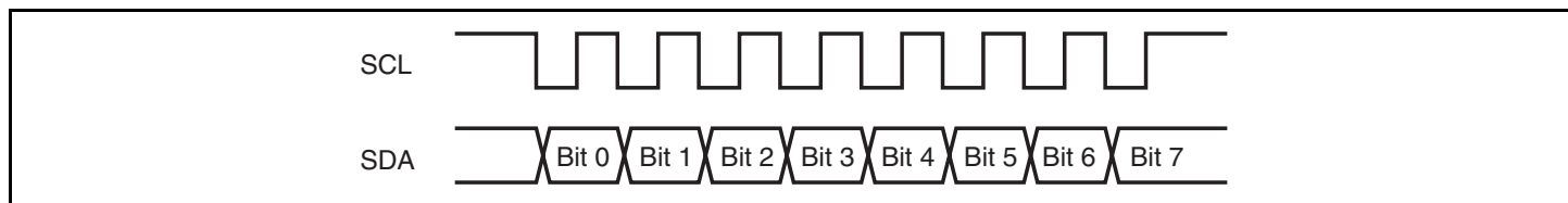
Figure 16.13 Clock Synchronous Serial Transfer Format
