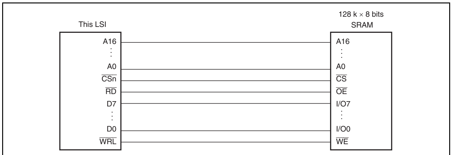
Figure 9.5 Example of 8-Bit Data-Width SRAM Connection
