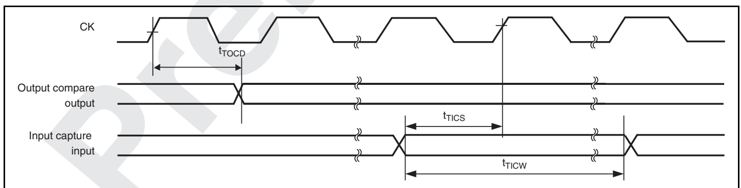
Figure 26.16 MTU2 Input/Output Timing
