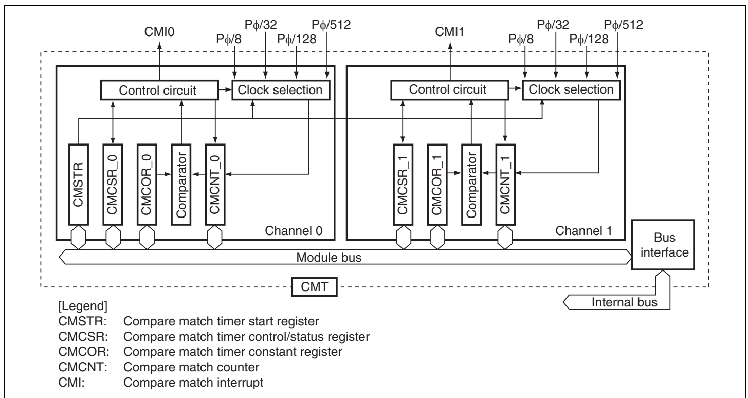
Figure 18.1 Block Diagram of CMT
