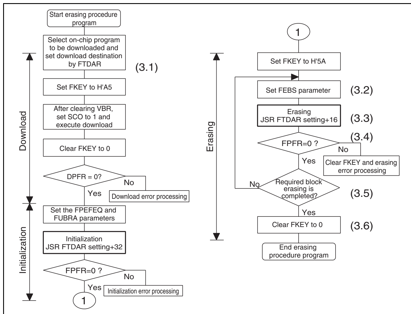
Figure 22.12 Erasing Procedure
