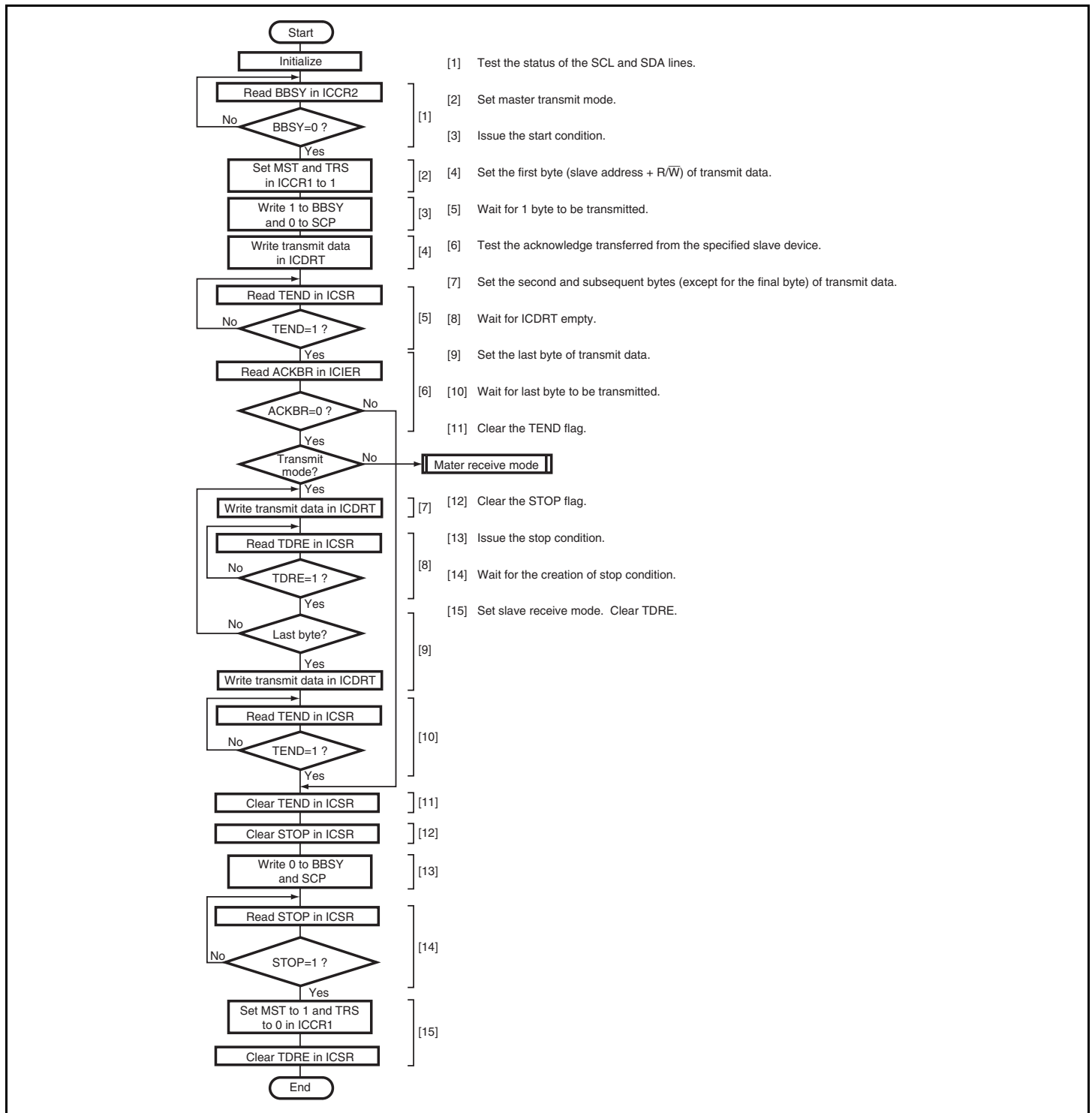
Figure 16.18 Sample Flowchart for Master Transmit Mode
