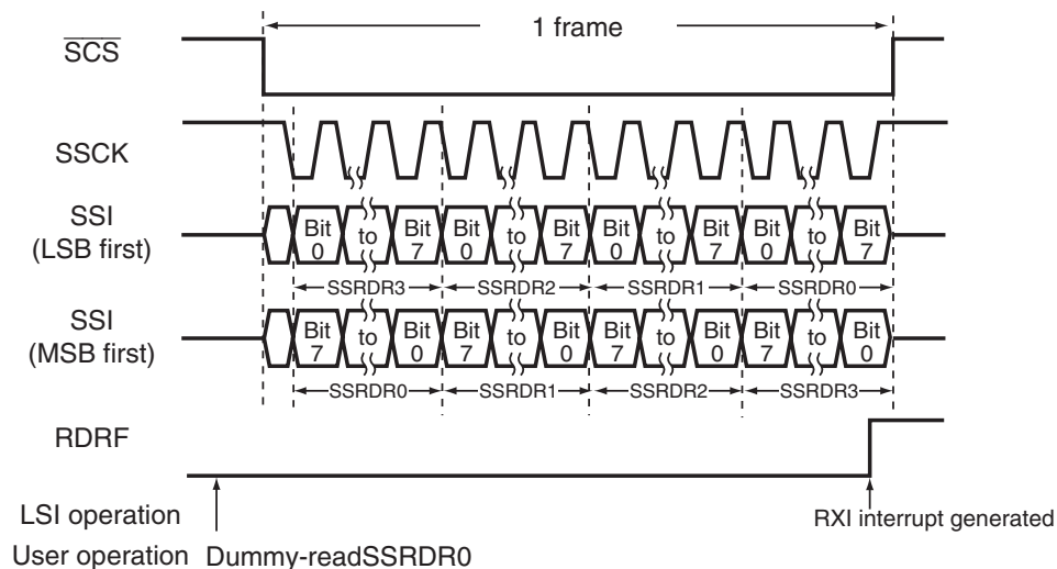
Figure 15.7 Example of Reception Operation (SSU Mode)
