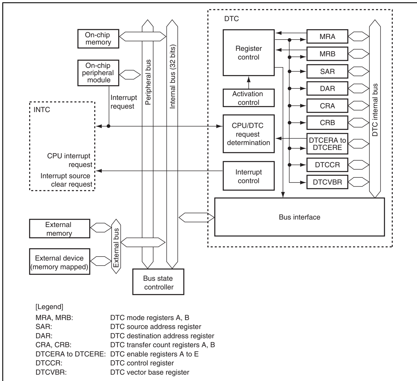
Figure 8.1 Block Diagram of DTC
