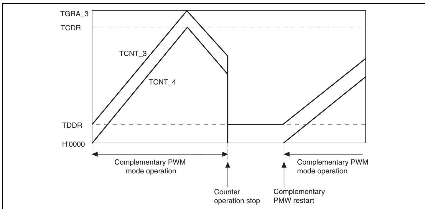
Figure 10.131 Counter Value during Complementary PWM Mode Stop
