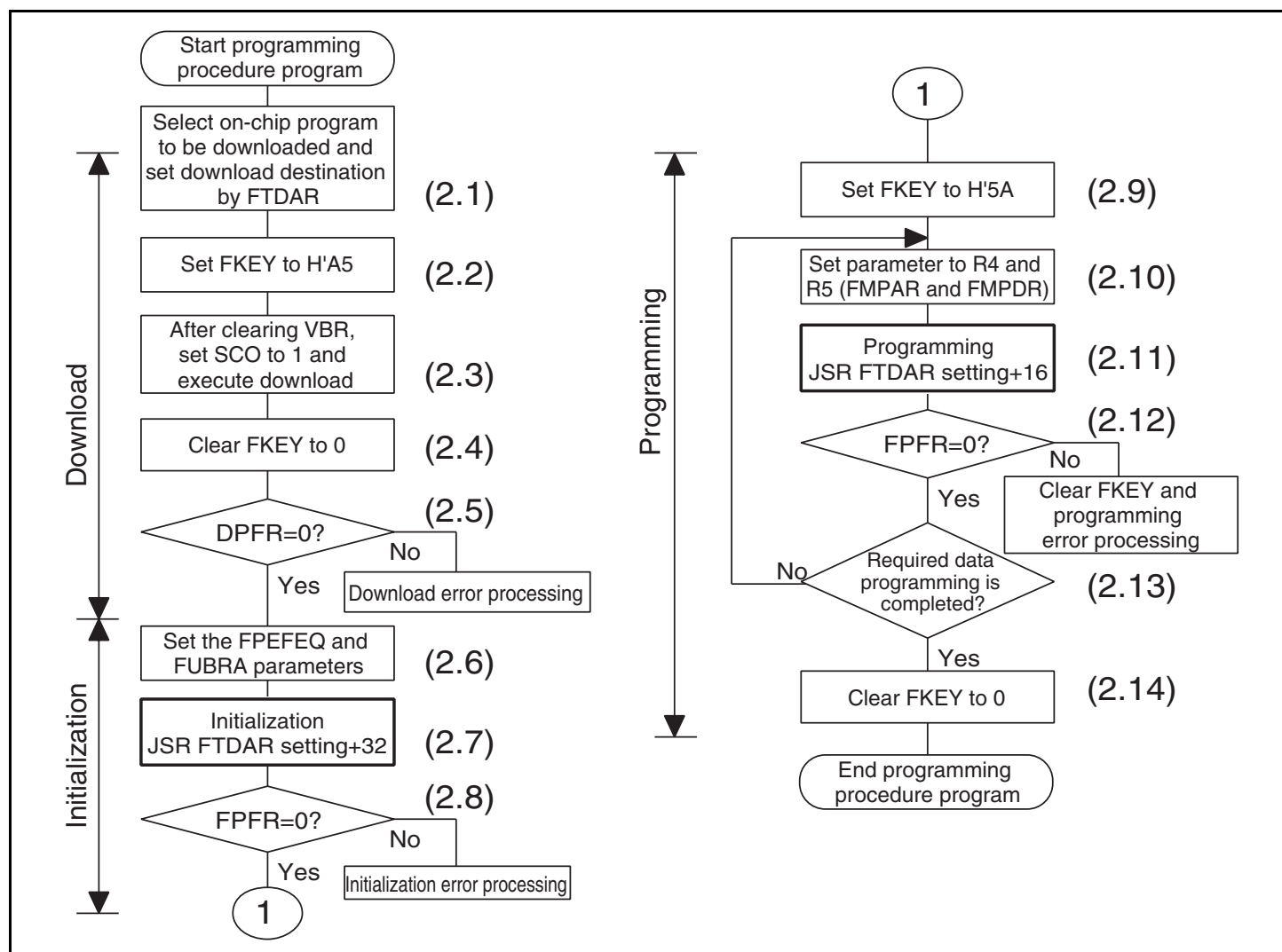
Figure 22.11 Programming Procedure
