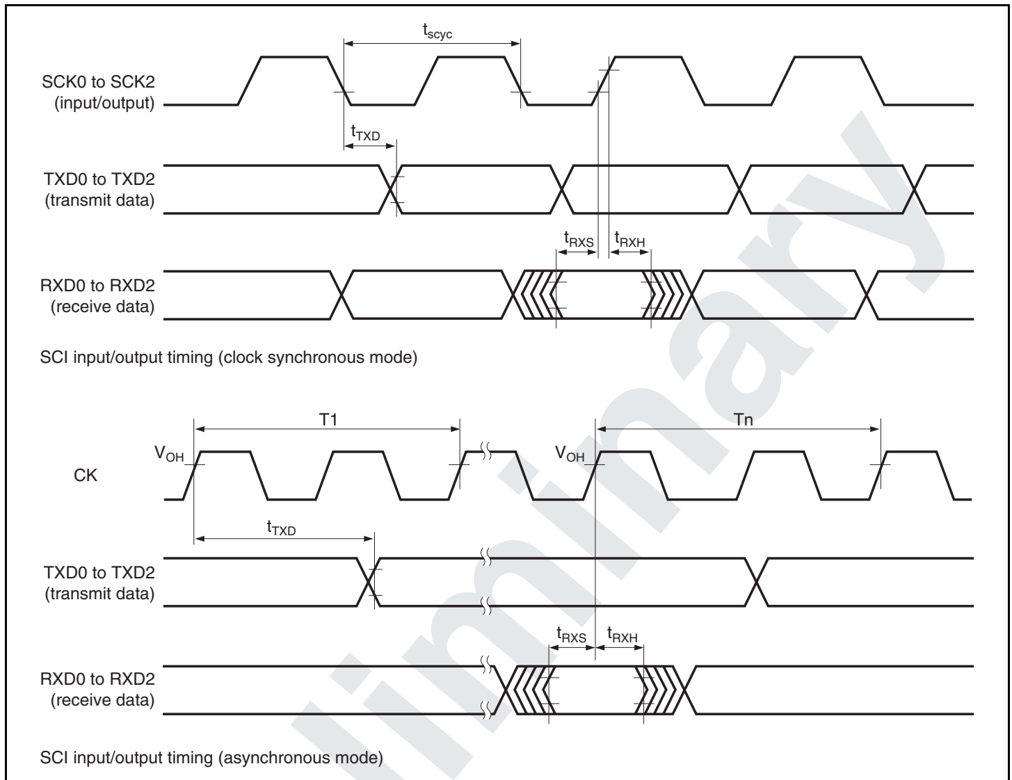
Figure 26.22 SCI Input/Output Timing
