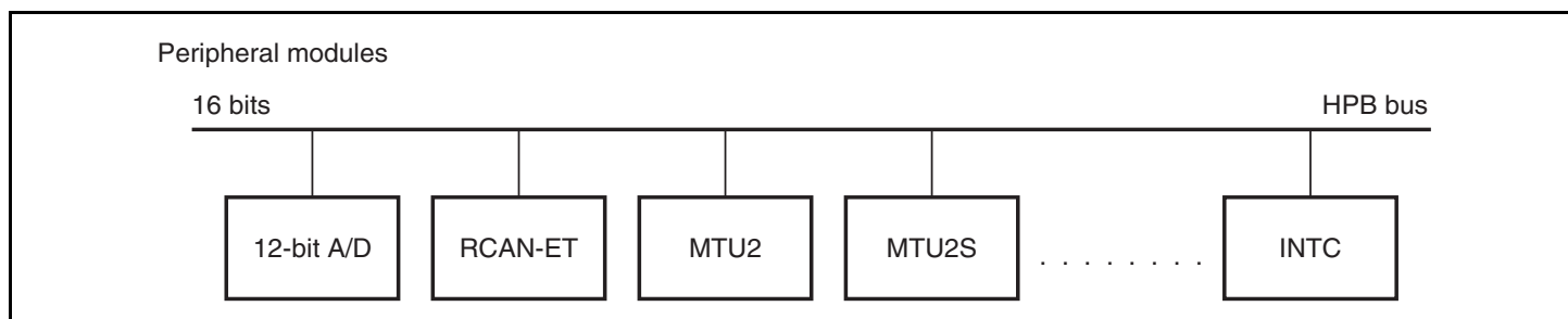
Figure 17.2 Interface Between CPU and 12-Bit A/D Converter
