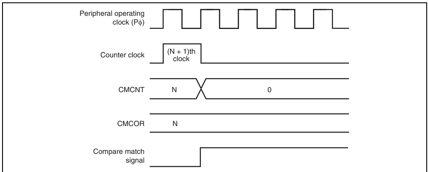
Figure 18.4 Timing of CMF Setting
