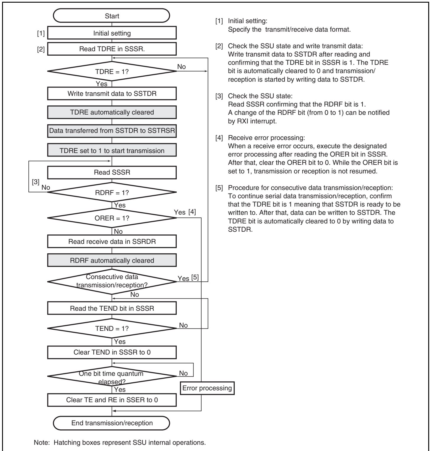
Figure 15.9 Flowchart Example of Simultaneous Transmission/Reception (SSU Mode)
