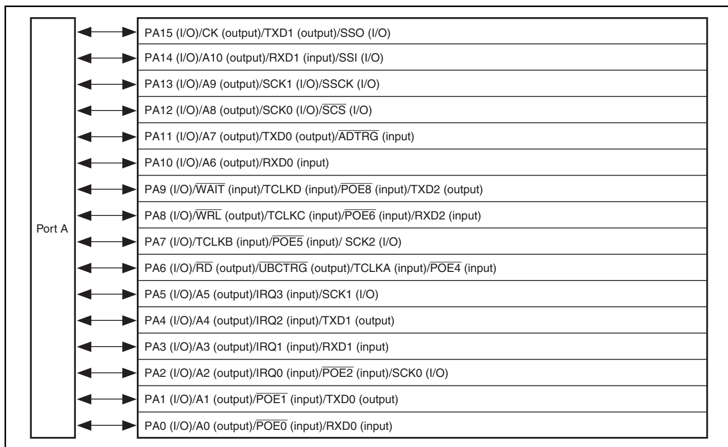
Figure 21.2 Port A (SH7137)
