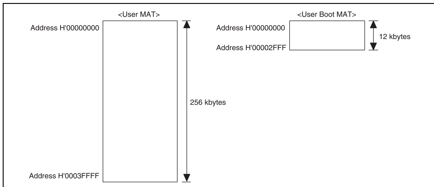
Figure 22.3 Flash Memory Configuration
