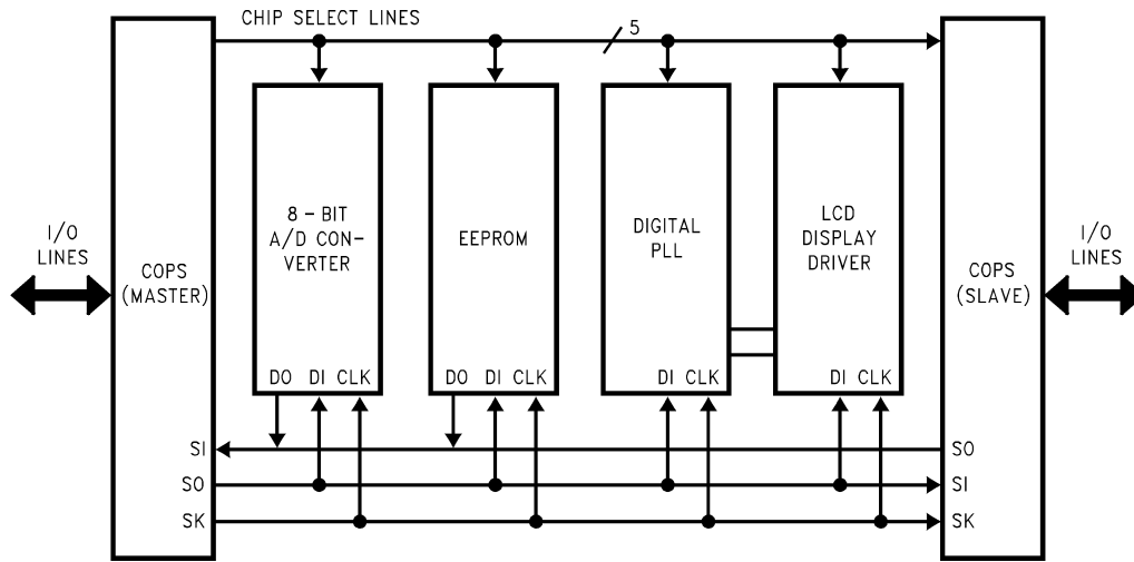
FIGURE 20. MICROWIRE/PLUS Application
