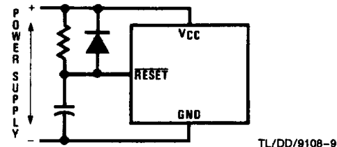
FIGURE 5. Recommended Reset Circuit
