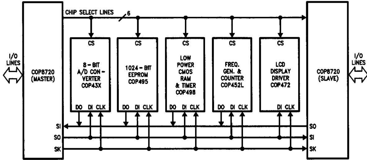
FIGURE 9. MICROWIRE/PLUS Application
