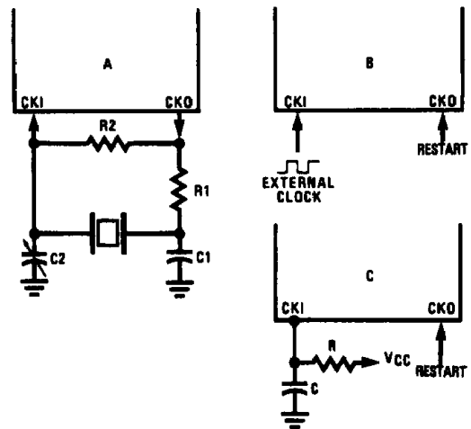
FIGURE 6. Crystal and R-C Connection Diagrams
