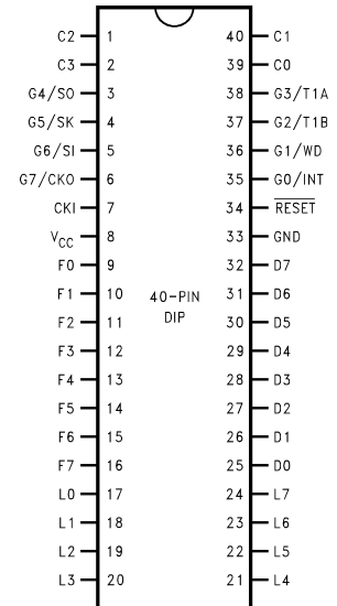
Top View
