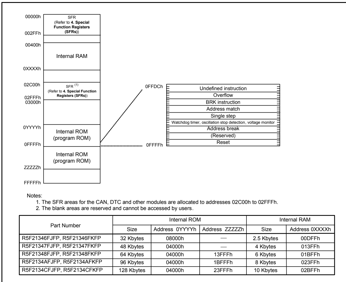
Figure 3.2 Memory Map of R8C/34F Group
