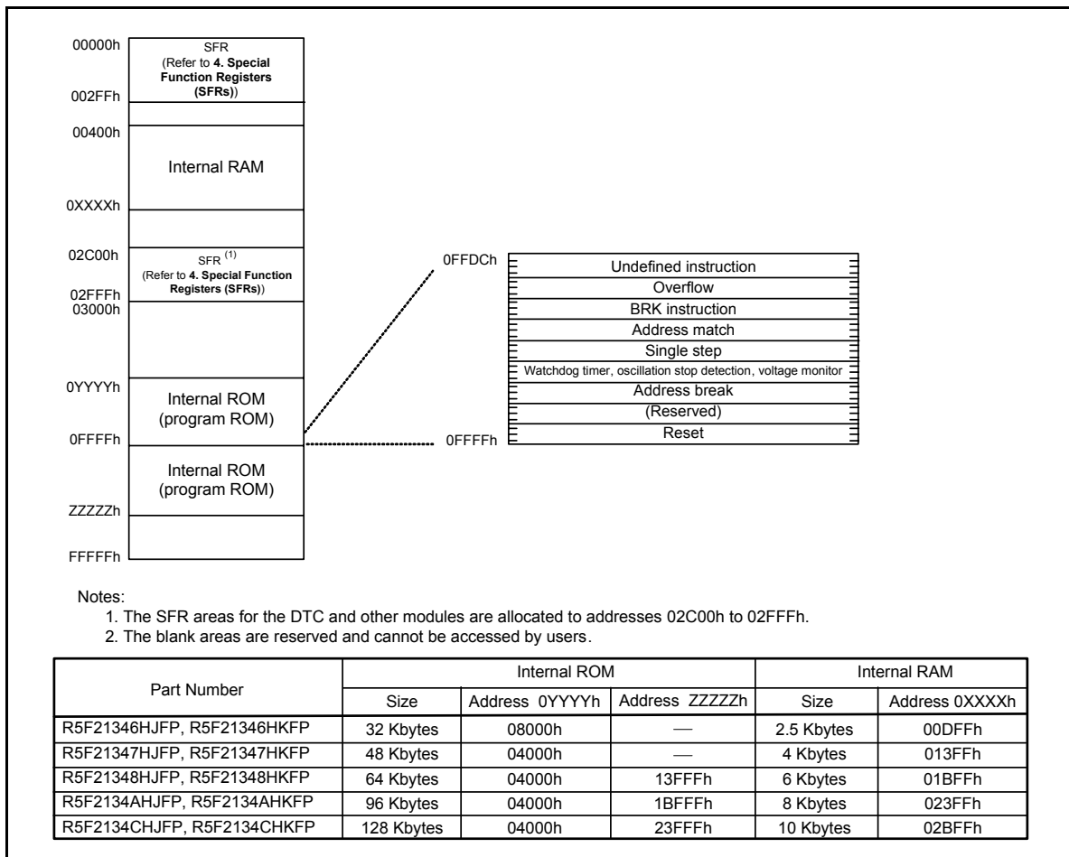
Figure 3.4 Memory Map of R8C/34H Group
