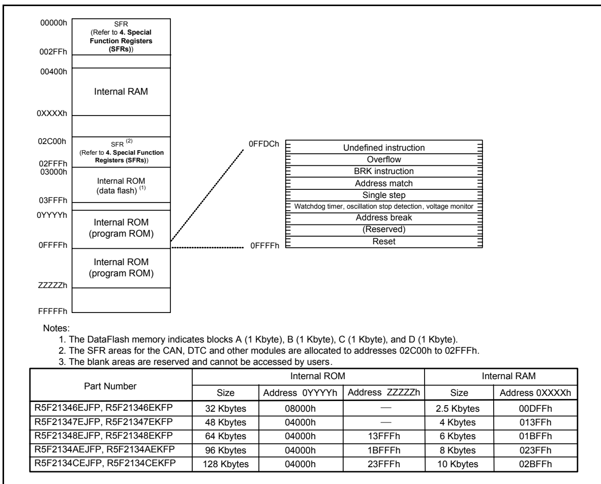
Figure 3.1 Memory Map of R8C/34E Group
