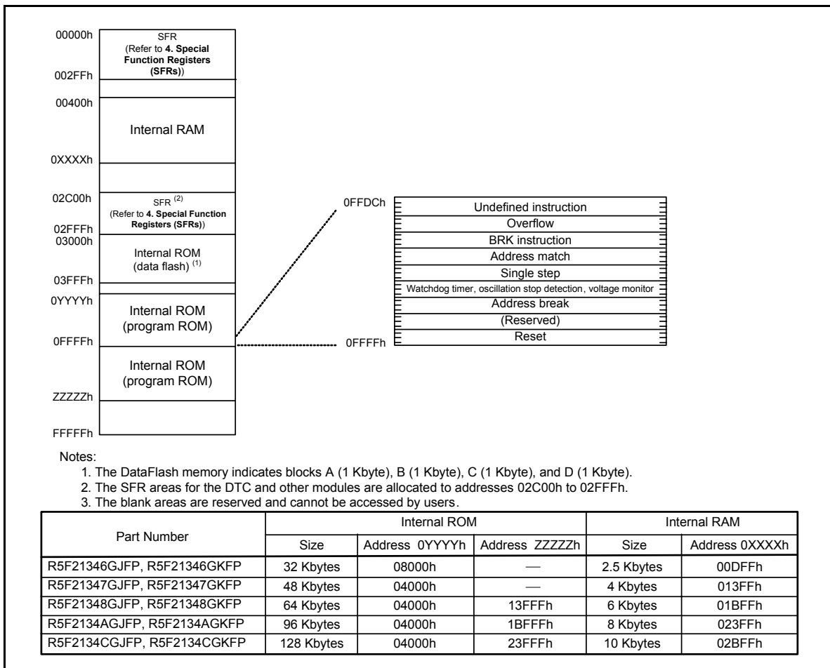
Figure 3.3 Memory Map of R8C/34G Group
