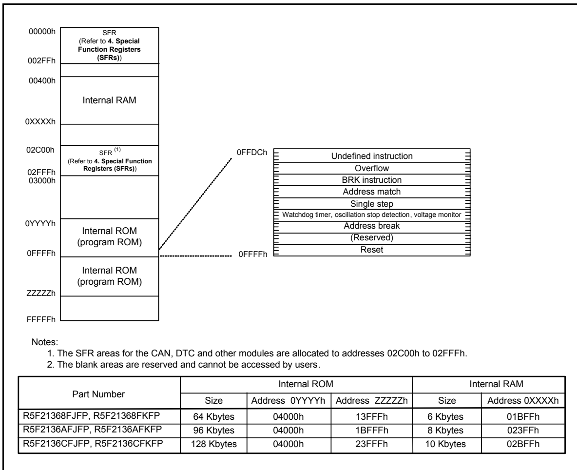
Figure 3.2 Memory Map of R8C/36F Group
