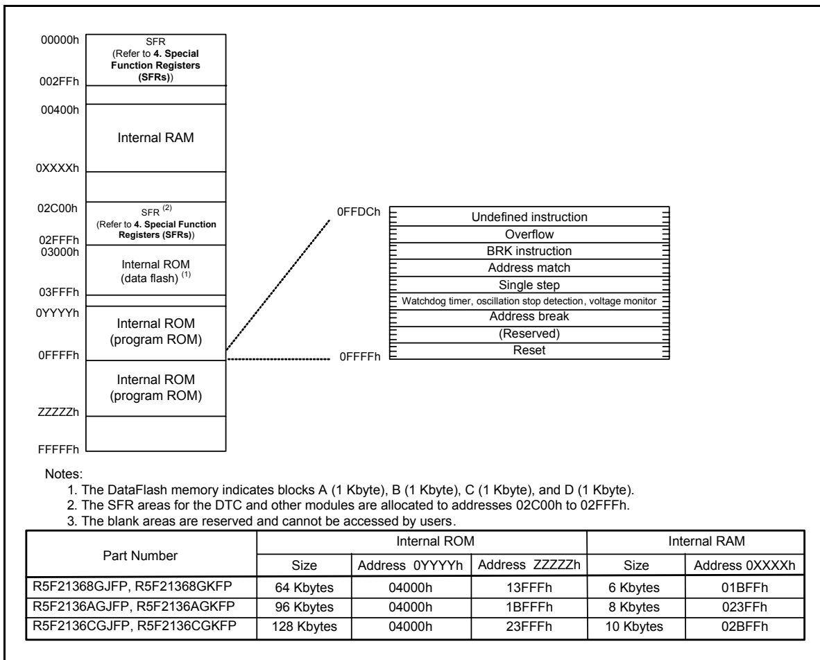
Figure 3.3 Memory Map of R8C/36G Group
