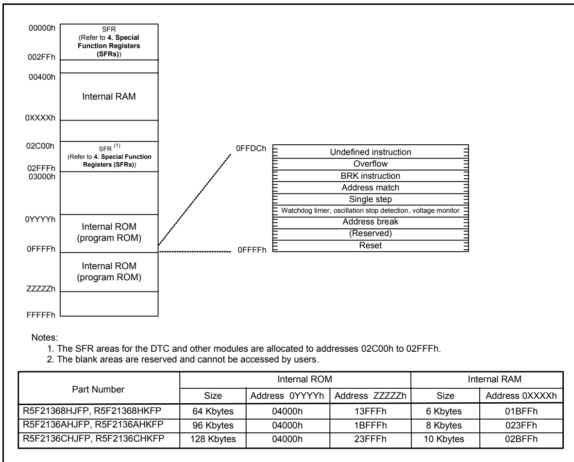
Figure 3.4 Memory Map of R8C/36H Group
