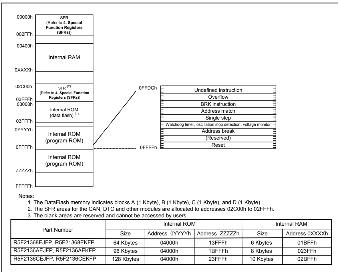
Figure 3.1 Memory Map of R8C/36E Group
