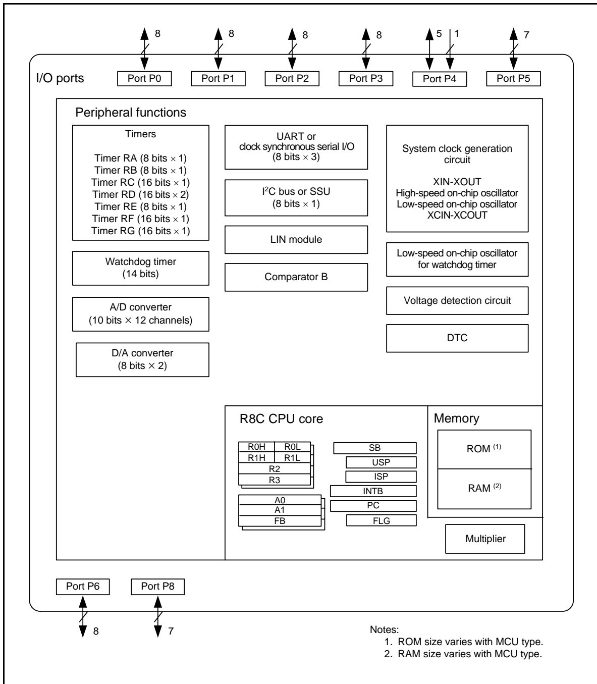
Figure 1.2 Block Diagram
