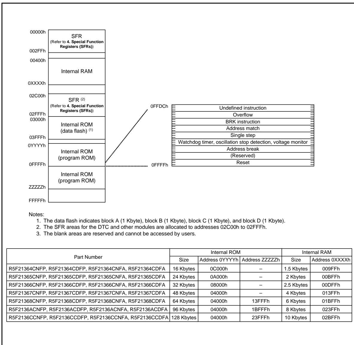
Figure 3.1 Memory Map of R8C/36C Group
