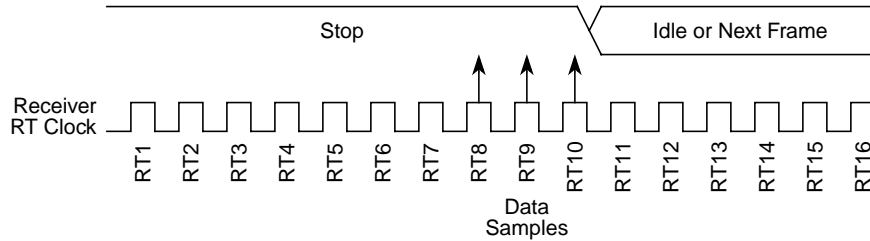
Figure 23-29. Fast Data
