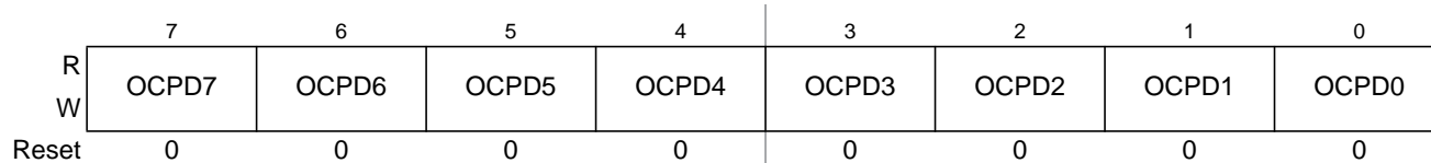
Figure 26-48. Output Compare Pin Disconnect Register (OCPD)
