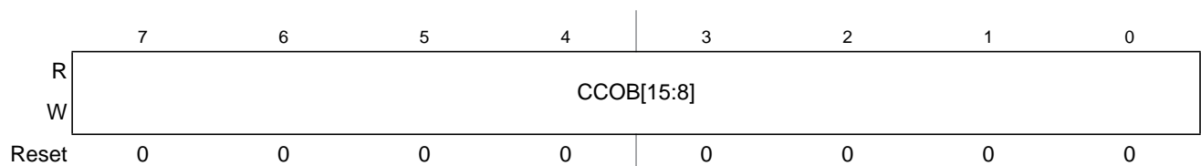
Figure 9-16. Flash Common Command Object High Register (FCCOBHI)
