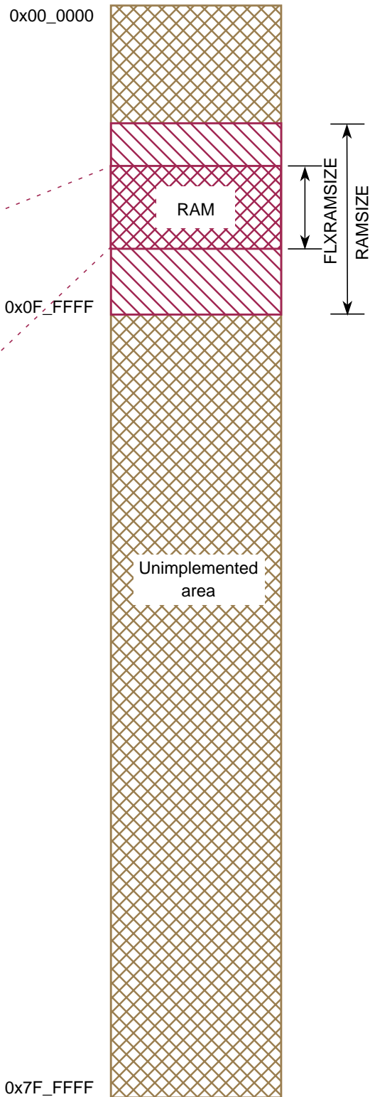
Figure 11-20. FLEXRAY Global Address Mapping
