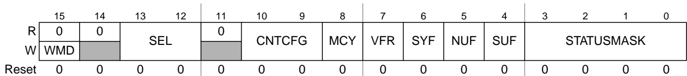
Figure 13-46. Slot Status Counter Condition Register (SSCCR)
