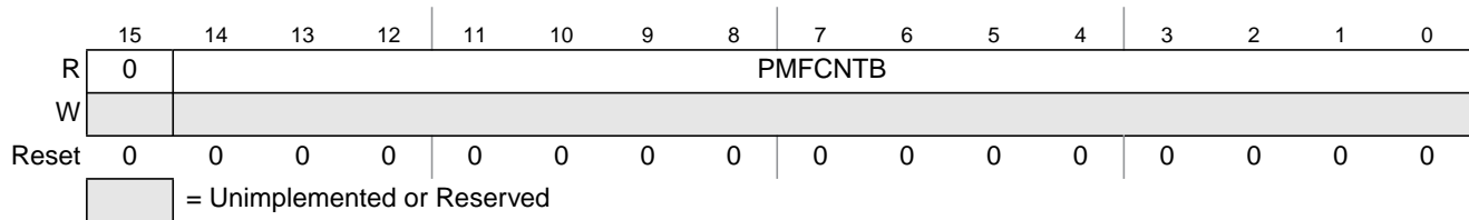
Figure 20-33. PMF Counter B Register (PMFCNTB)
