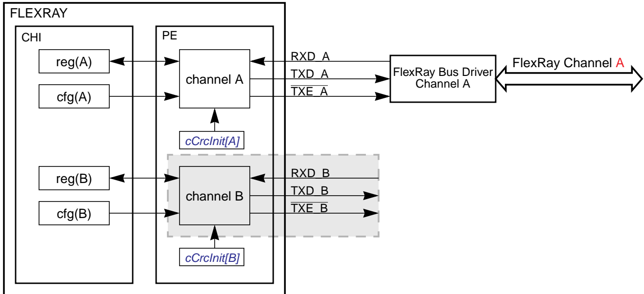
Figure 13-134. Single Channel Device Mode (Channel A)
