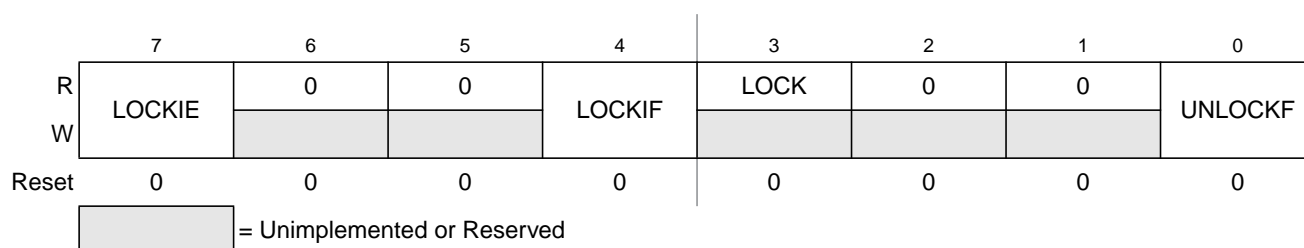
Figure 12-5. CGMIPLL Flags Register (CGMFLG)
