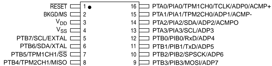
Figure 2-2. 16-Pin TSSOP
