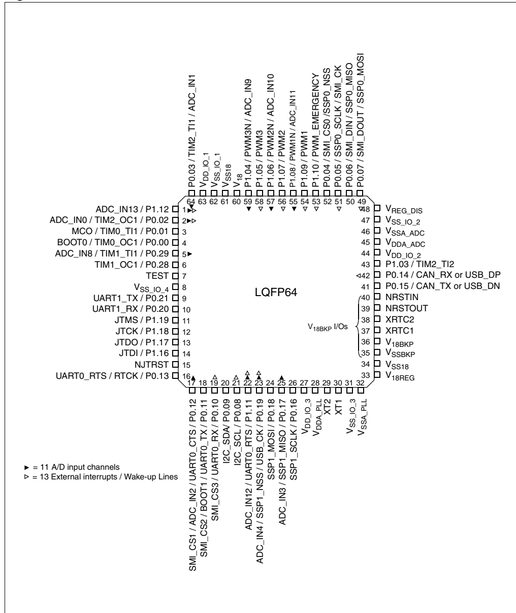
Figure 3. LQFP64 Pinout
