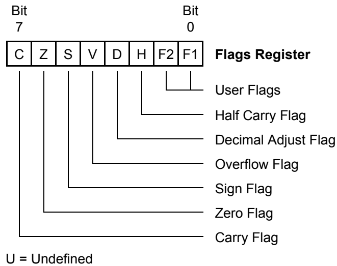
Figure 53. Flags Register
