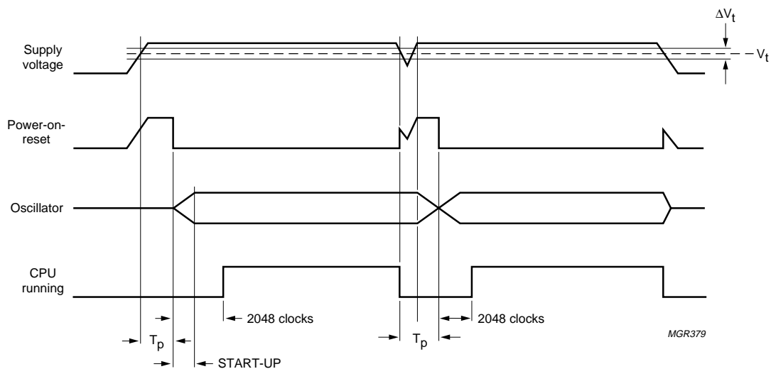
Fig.10 Power-on reset switching level.
