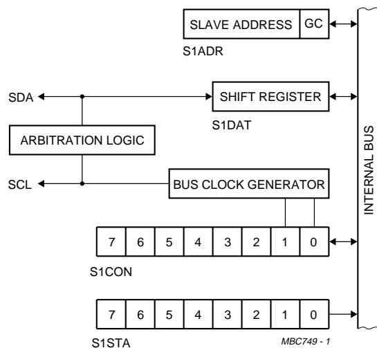
Fig.6 Block diagram of the I 2 C-bus serial I/O.
