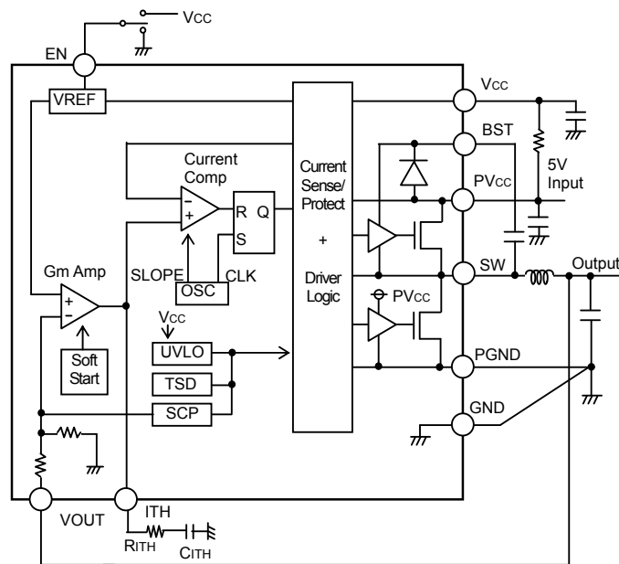
Fig.2 BD9134MUV Block Diagram
