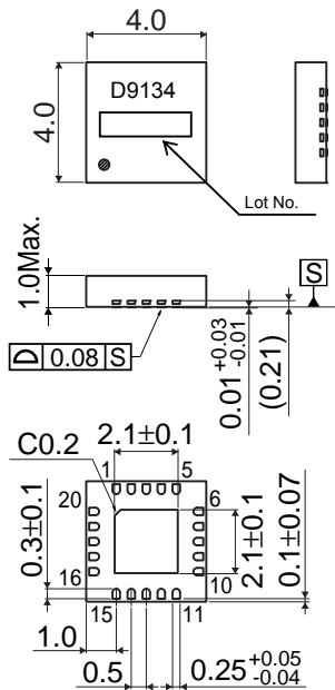
Fig.1 BD9134MUV TOP View
