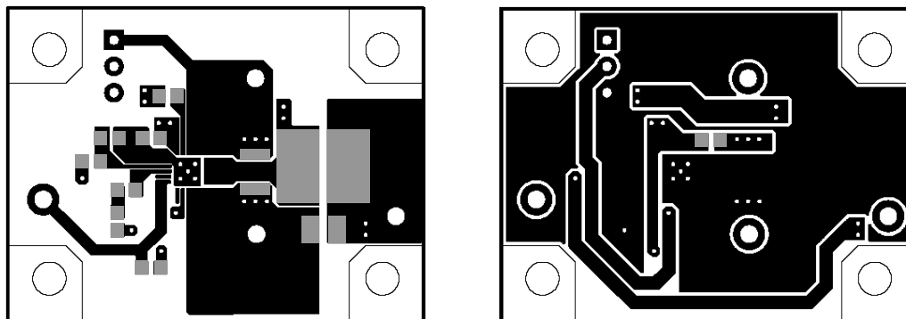
Fig.33 Layout diagram
