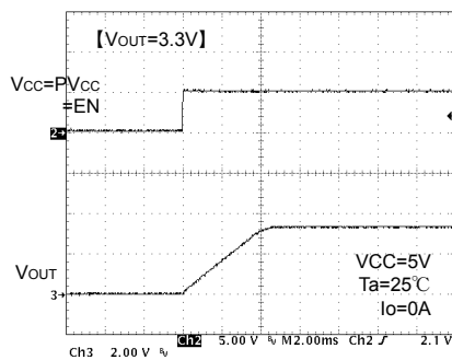
Fig.13 Soft start waveform
