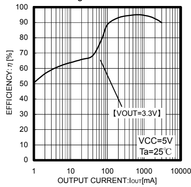
Fig.7 Efficiency
