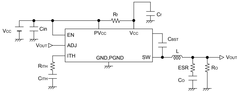
Fig.32 Typical application
