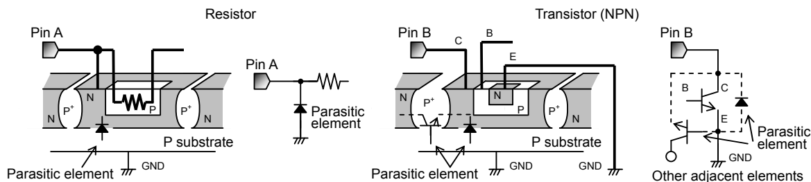
Fig.35 Simplified structure of monolithic IC
