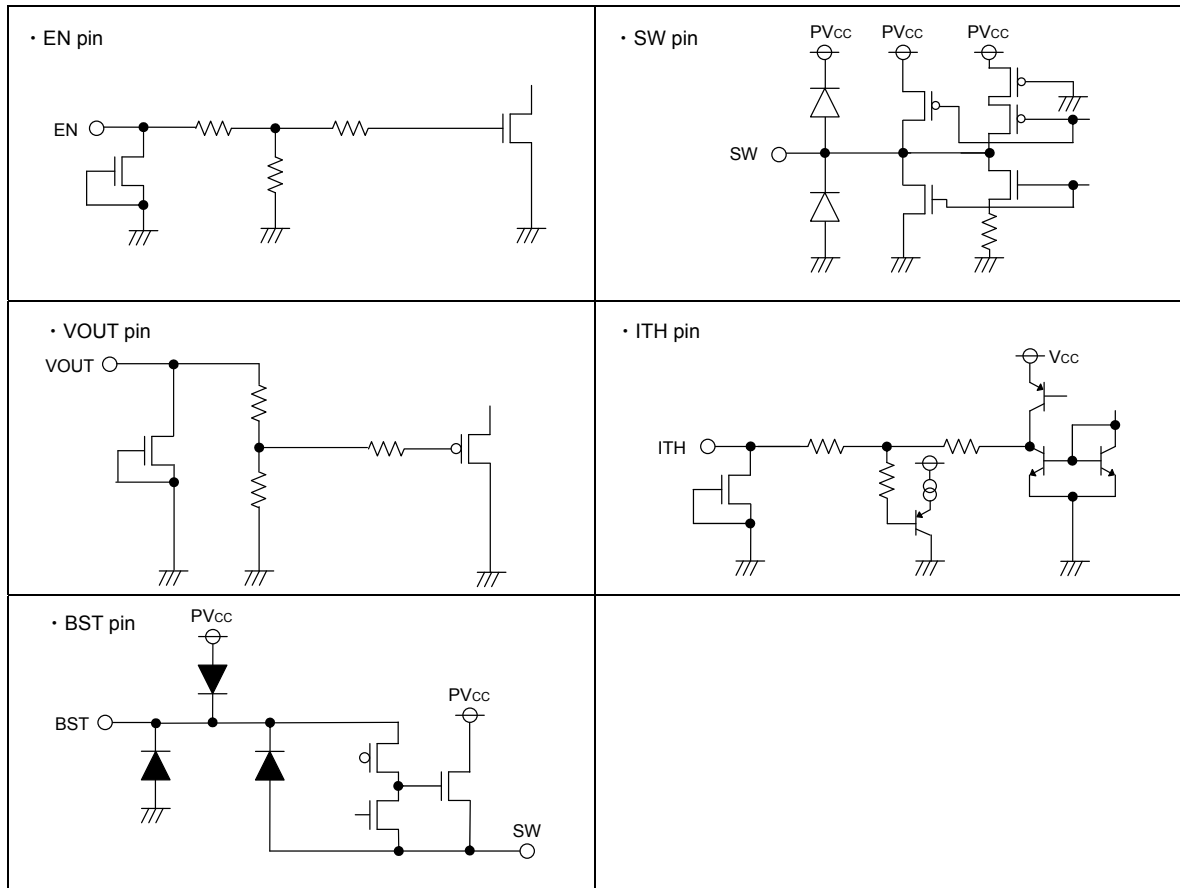
Fig.34 I/O equivalence circuit
