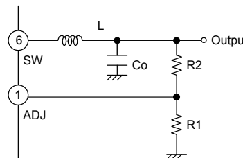
Fig.36 Determination of output voltage
