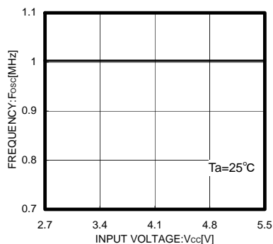
Fig.12 Power supply voltage-Operating frequency
