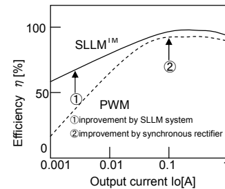
Fig.21 Efficiency
