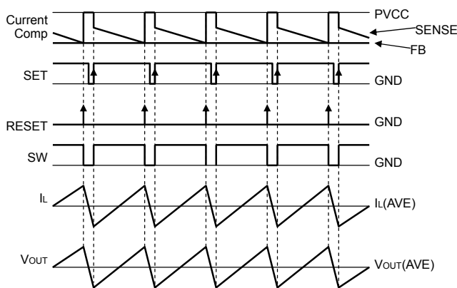
Fig.24 PWM switching timing chart
