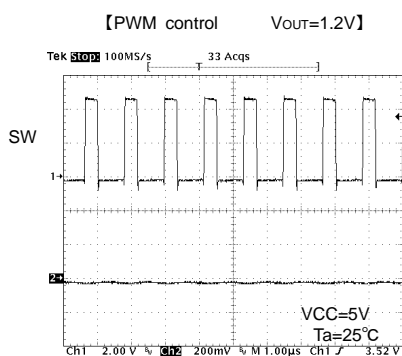
Fig.15 SW waveform Io=4A
