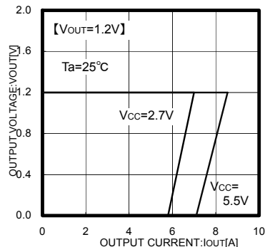
Fig.5 I OUT -V OUT
