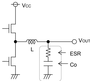
Fig.31 Output capacitor
