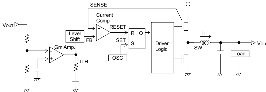
Fig.23 Diagram of current mode PWM control
