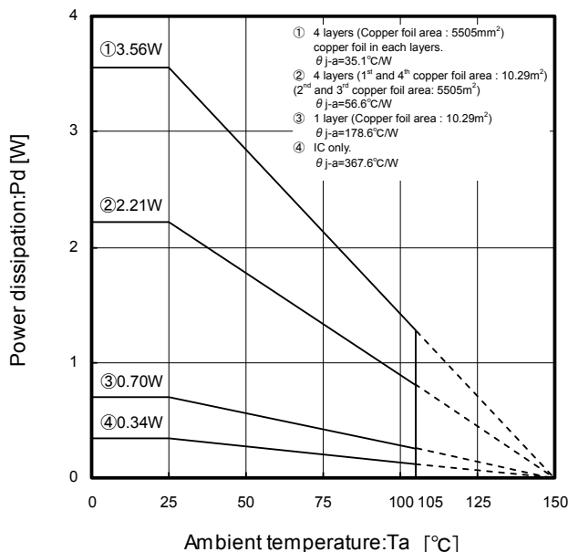
Fig.29 Thermal derating curve (VQFN020V4040)
