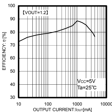
Fig.7 Efficiency
