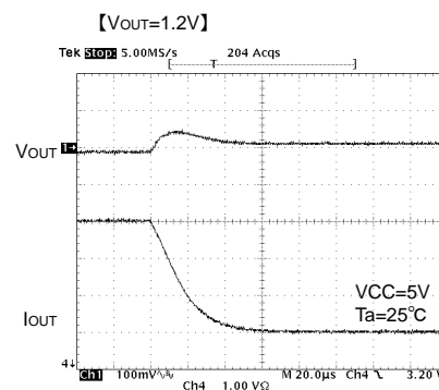
Fig.17 Transient Response Io=4A→1A(20μs)
