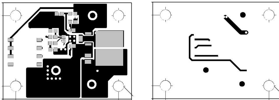
Fig.38 Layout diagram
