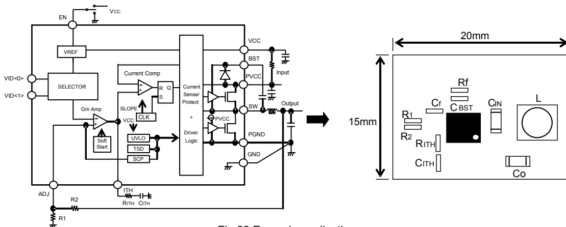
Fig.22 Example application
