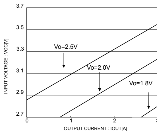
Fig.37 minimum input voltage in each output voltage
