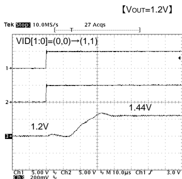
Fig.18 Change Response
