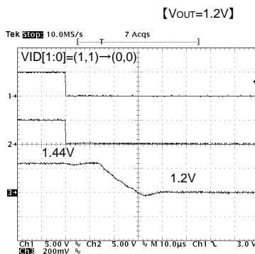
Fig.19 Change Response
