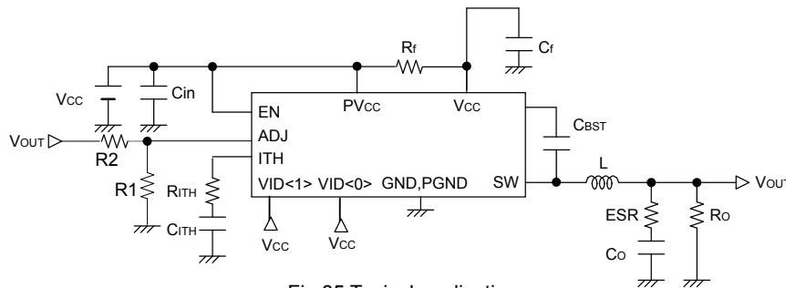
Fig.35 Typical application
