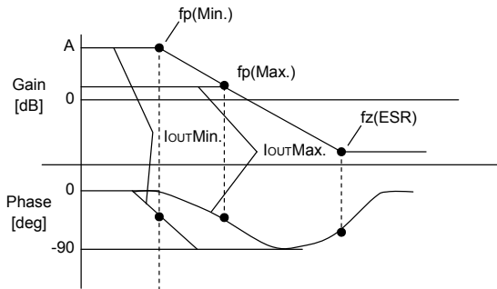
Fig.33 Open loop gain characteristics
