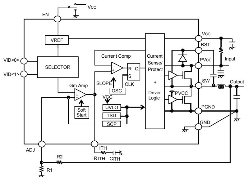
Fig.2 Block Diagram
