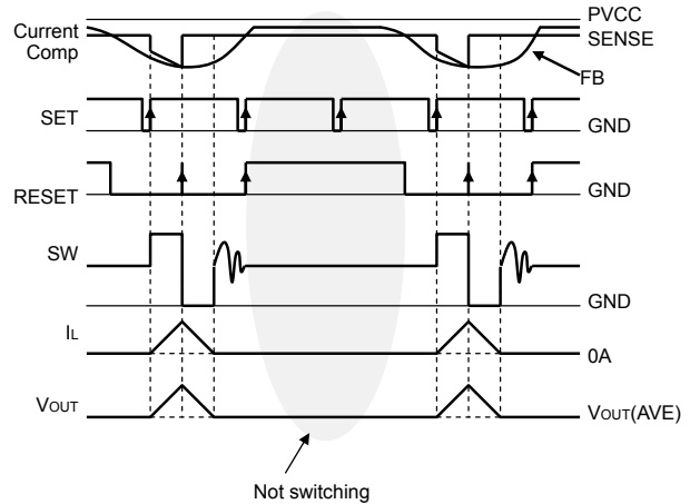
Fig.25 SLLM™ switching timing chart
