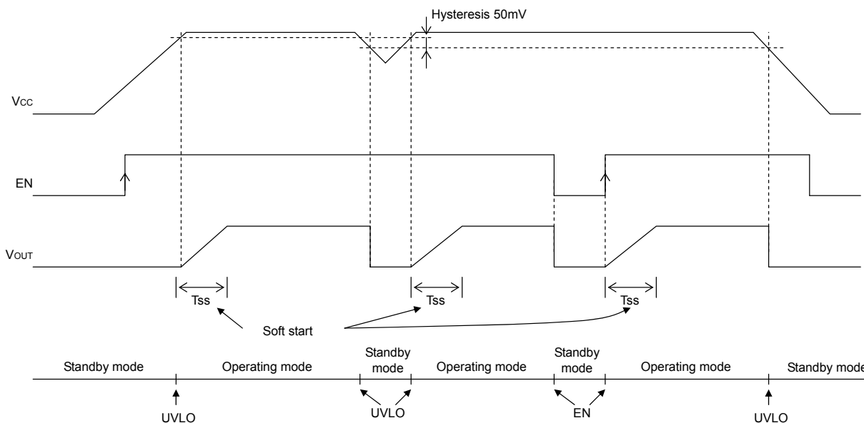
Fig.26 Soft start, Shutdown, UVLO timing chart
