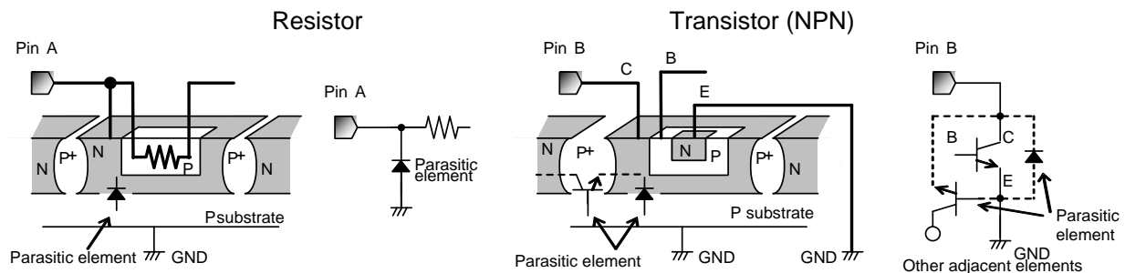
Fig.40 Simplified structure of monolithic IC
