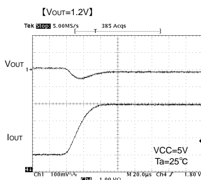
Fig. 16 Transient Response Io=1A→4A(20μs)
