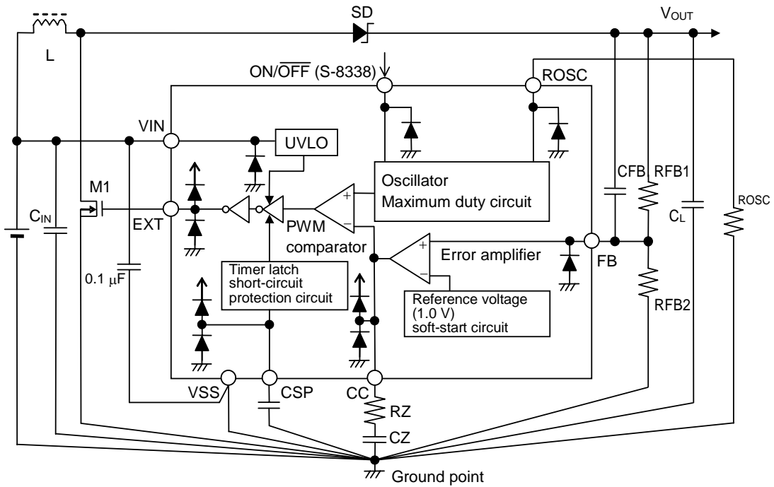
Figure 16 Standard Circuit (S-8338 Series)
