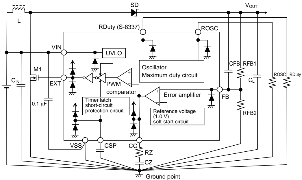
Figure 15 Standard Circuit (S-8337 Series)
