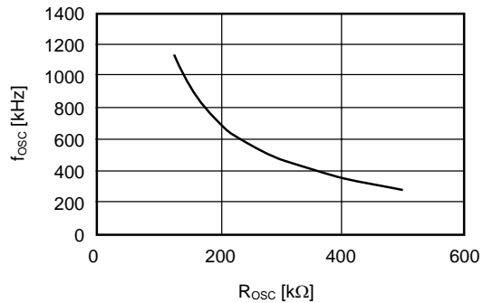
Figure 12 R osc vs. f osc
