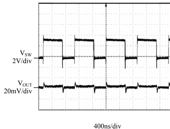
Figure 9. Heavy Load Operation ( V_{IN}=3.6V , V_{OUT}=1.8V , I_{OUT}=600mA )
