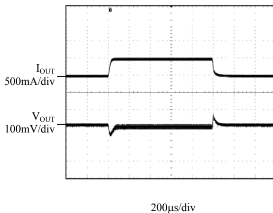
Figure 10. Load Transient ( V_{IN}=3.6V , V_{OUT}=1.8V , I_{OUT}=0mA to 500mA )
