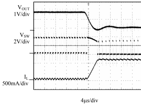
Figure 12. Short Circuit Protection ( V_{IN}=3.6V , V_{OUT}=1.8V , no load)
