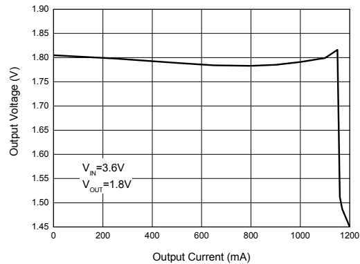
Figure 7. Output Voltage vs. Output Current
