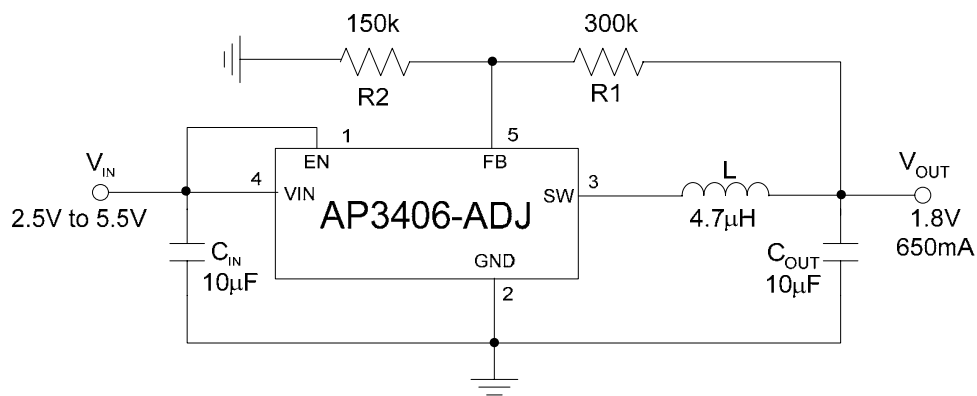
Figure 17. Typical Application of AP3406
