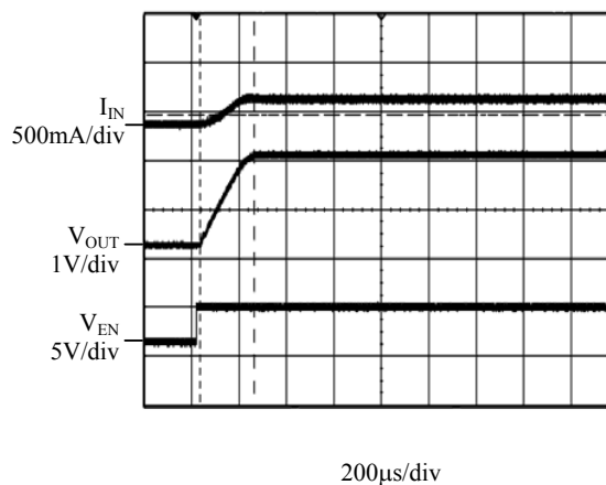
Figure 11. Start up from Shutdown ( V_{IN}=3.6V , V_{OUT}=1.8V , R_{LOAD}=4\Omega )
