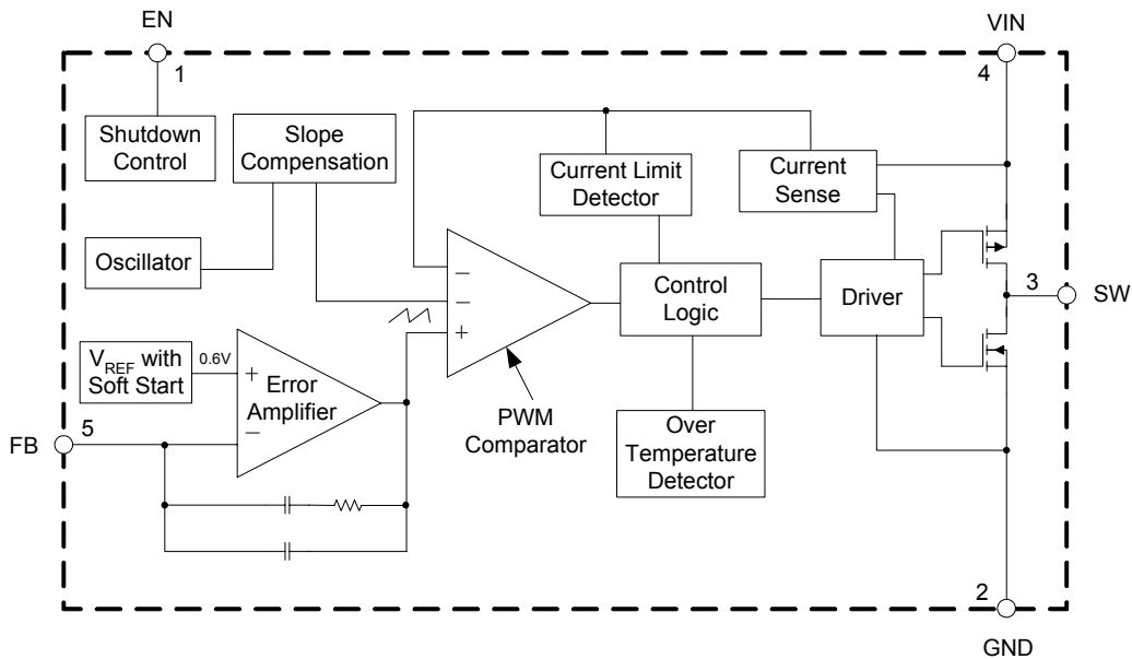
Figure 3. Functional Block Diagram of AP3406
