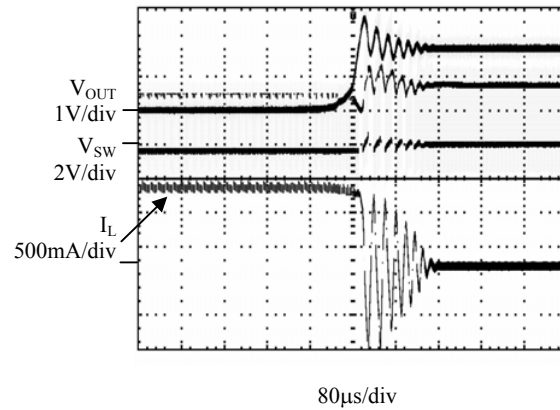
Figure 13. Short Circuit Recovery ( V_{IN}=3.6V , V_{OUT}=1.8V , no load)
