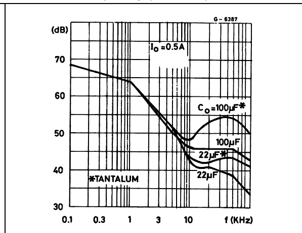
Figure 21. Supply voltage rejection vs frequency (L4940V5)
