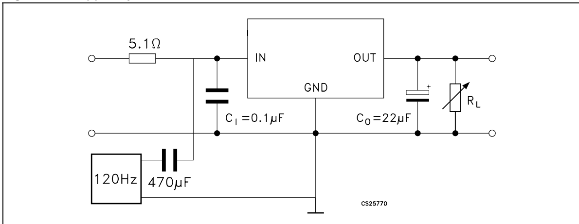
Figure 5. Ripple rejection
