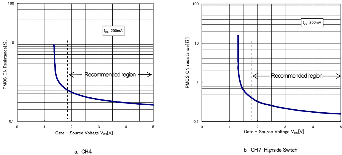
Fig - 11 Built-in PMOS ON resistance - V_{GS}
