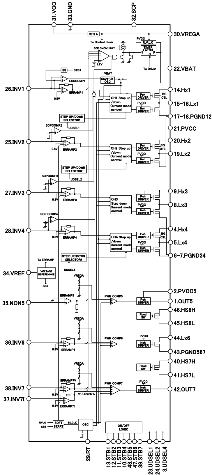
Fig. 3 Block diagram
