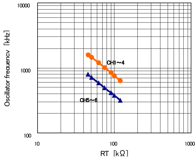
Fig-12 Oscillator frequency – RT resistor (EX)
