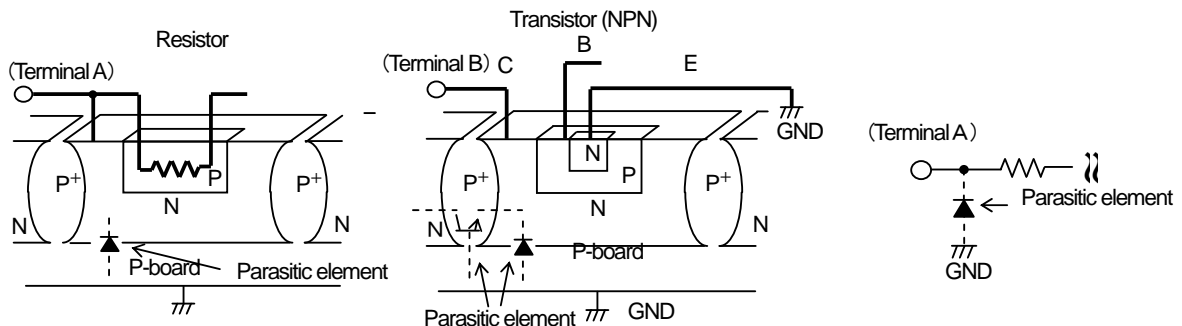
Fig - 15 Simplified structure of a Bipolar IC
