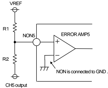
Fig-13 setting for CH5 feed back resistor
