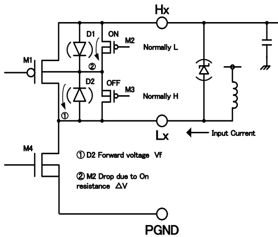
Fig - 9 Back gate control
