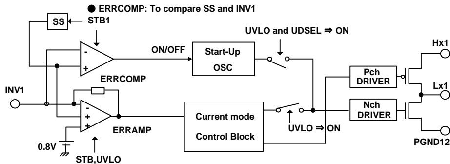
Fig - 6 CH1 Block diagram: Start up circuit
