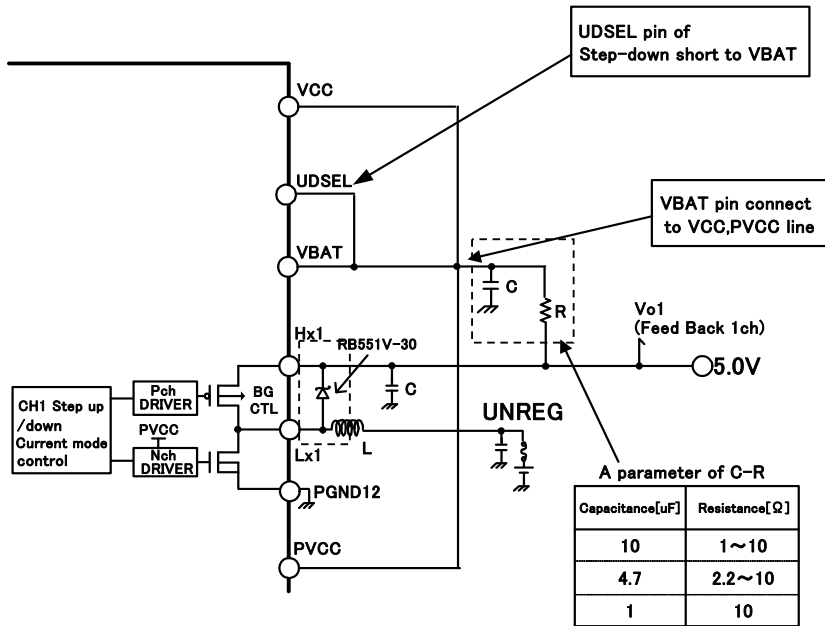
Fig - 6 CH1 Block diagram: Start up circuit
