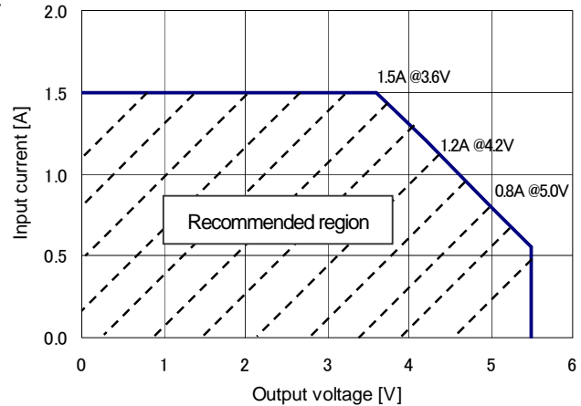
Fig - 10 Recommended operating area of using back-gate
