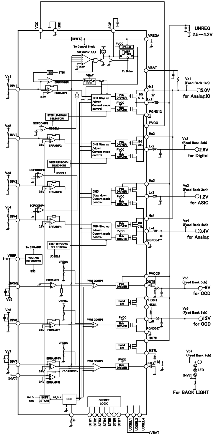
Fig. 4 (2) Application Circuit for Li battery 1cell
