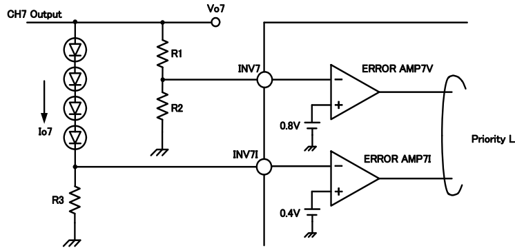
Fig-14 Setting for Voltage and current of CH7.
