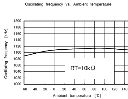
Fig.4 Oscillating frequency – Ambient temperature (RT=10kΩ)
