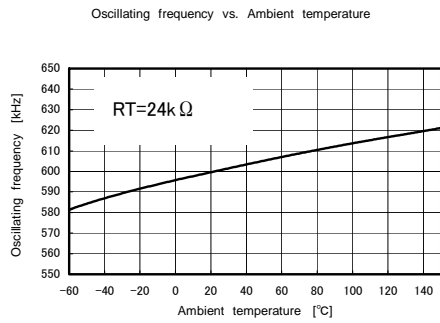
Fig.3 Oscillating frequency – Ambient temperature (RT=24kΩ)
