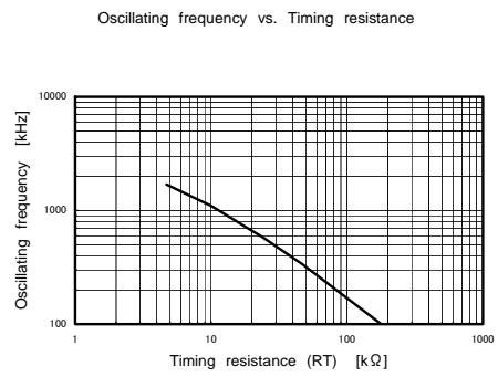
Fig.2 Oscillating frequency – Timing resistance (RRT)
