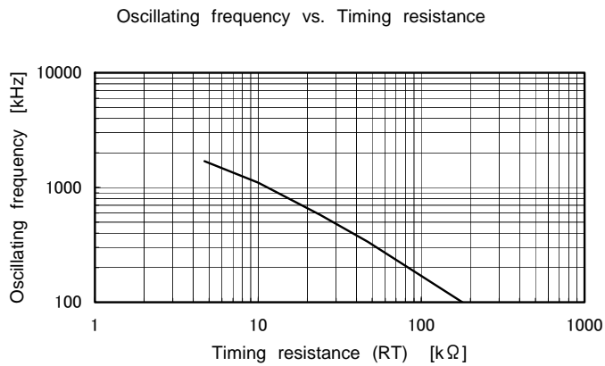
Fig.5 Oscillating frequency – Timing resistance (RRT)
