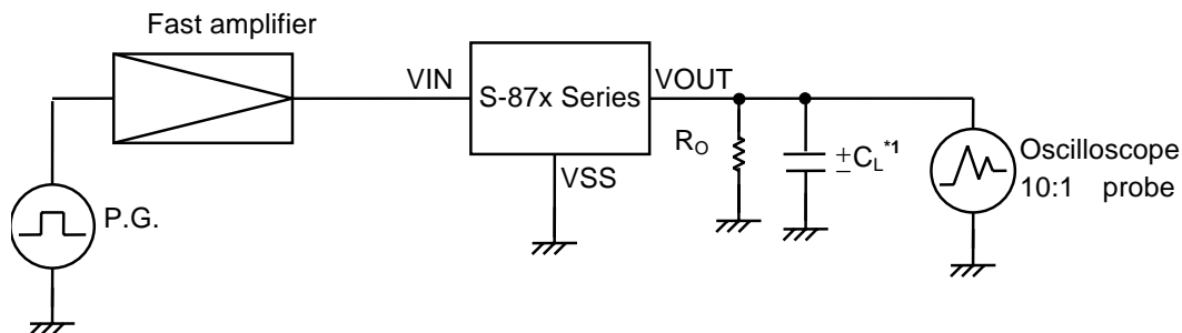
Figure 27 Rectangular wave from 0 V to 10 V (Type 2)
