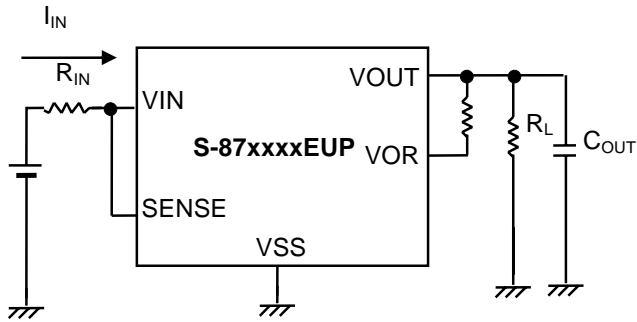
Figure 24 Attention connecting example 2
