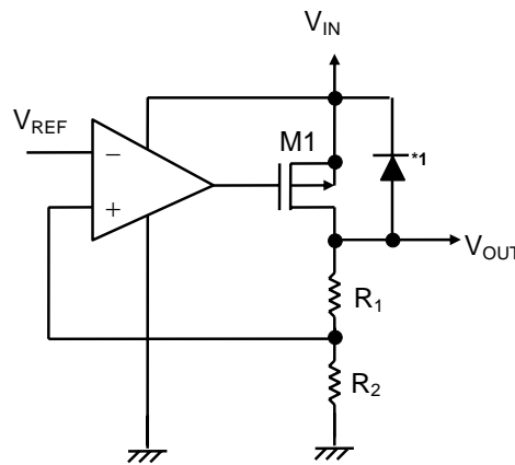
Figure 18 Voltage regulator circuit
