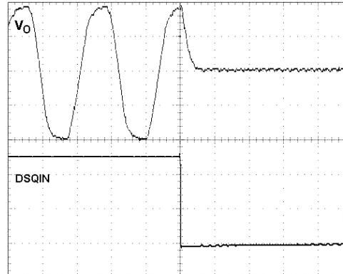
Figure 32. DSQIN Tone Disable Transient Response
