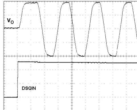
Figure 30. DSQIN Tone Enable Transient Response
