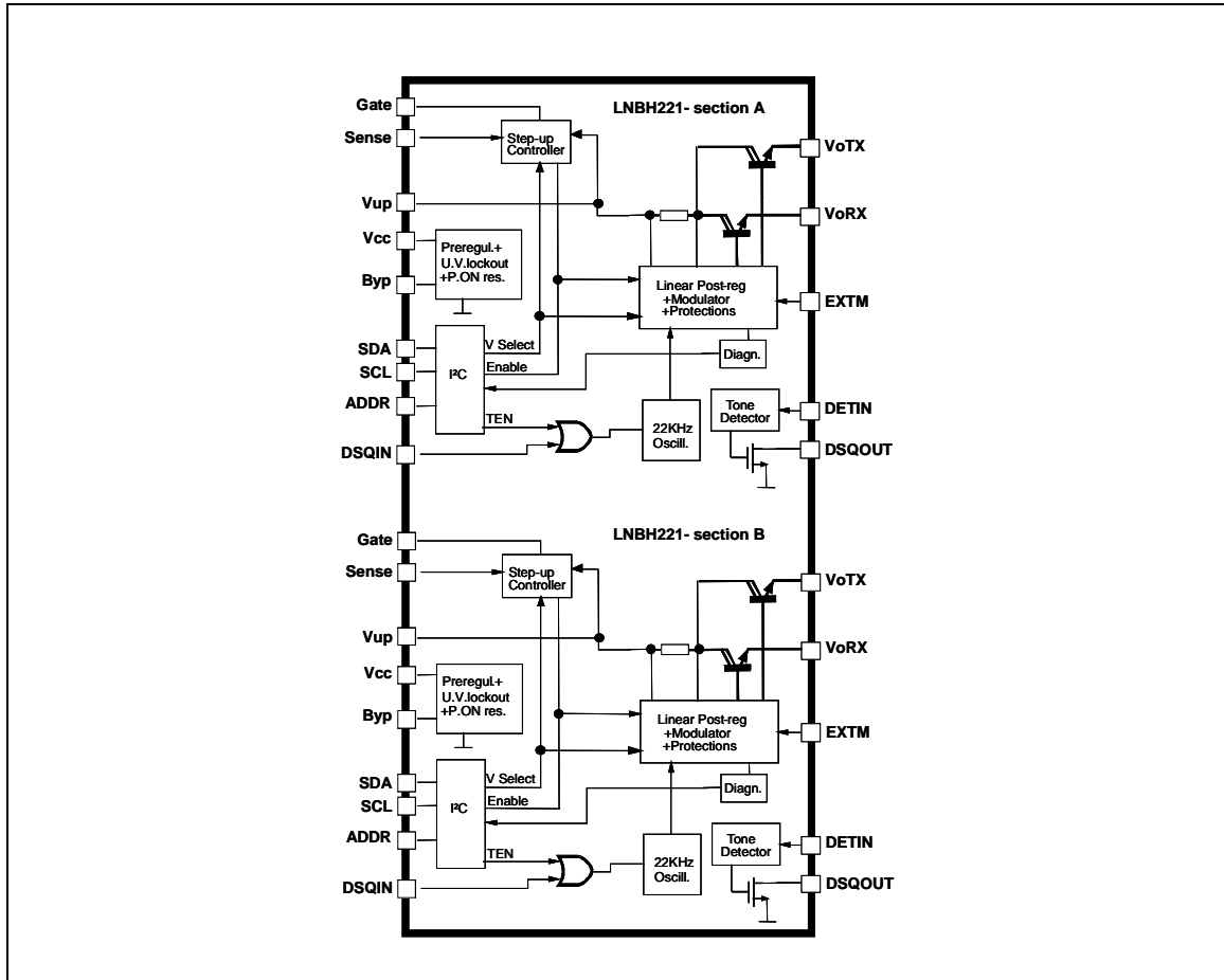
Figure 1. Block diagram
