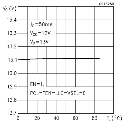
Figure 11. Output Voltage vs Temperature
