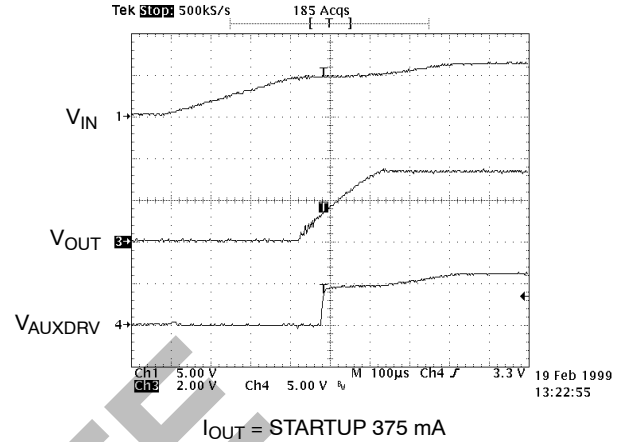
Figure 13. Initial Power-Up, V_{AUX} Not Present R_{OUT} = 8.8 \Omega
