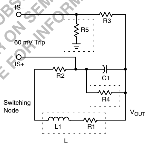
Figure 8. Current Limit
