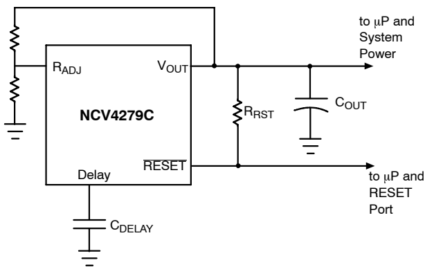
Figure 12. Adjustable \overline{\text{RESET}}
