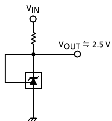
(1) 2.5 V REFERENCE
