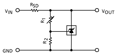
(2) SHUNT REGULATOR
