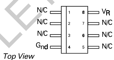
S08 Package Suffix - N8
