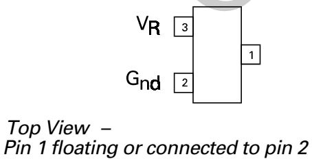
SOT23 Package Suffix - F
