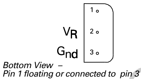
E-Line, 3 pin Package Suffix - A
