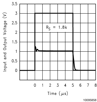
Pulse Response 2
