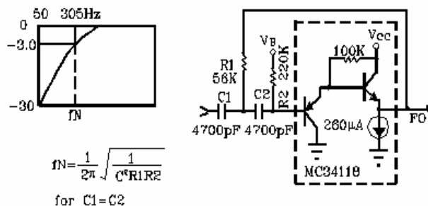
Figure 8. High Pass Filter
