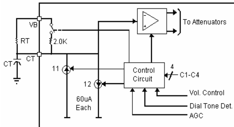
Figure 6. CT Attenuator Control Block Circuit
