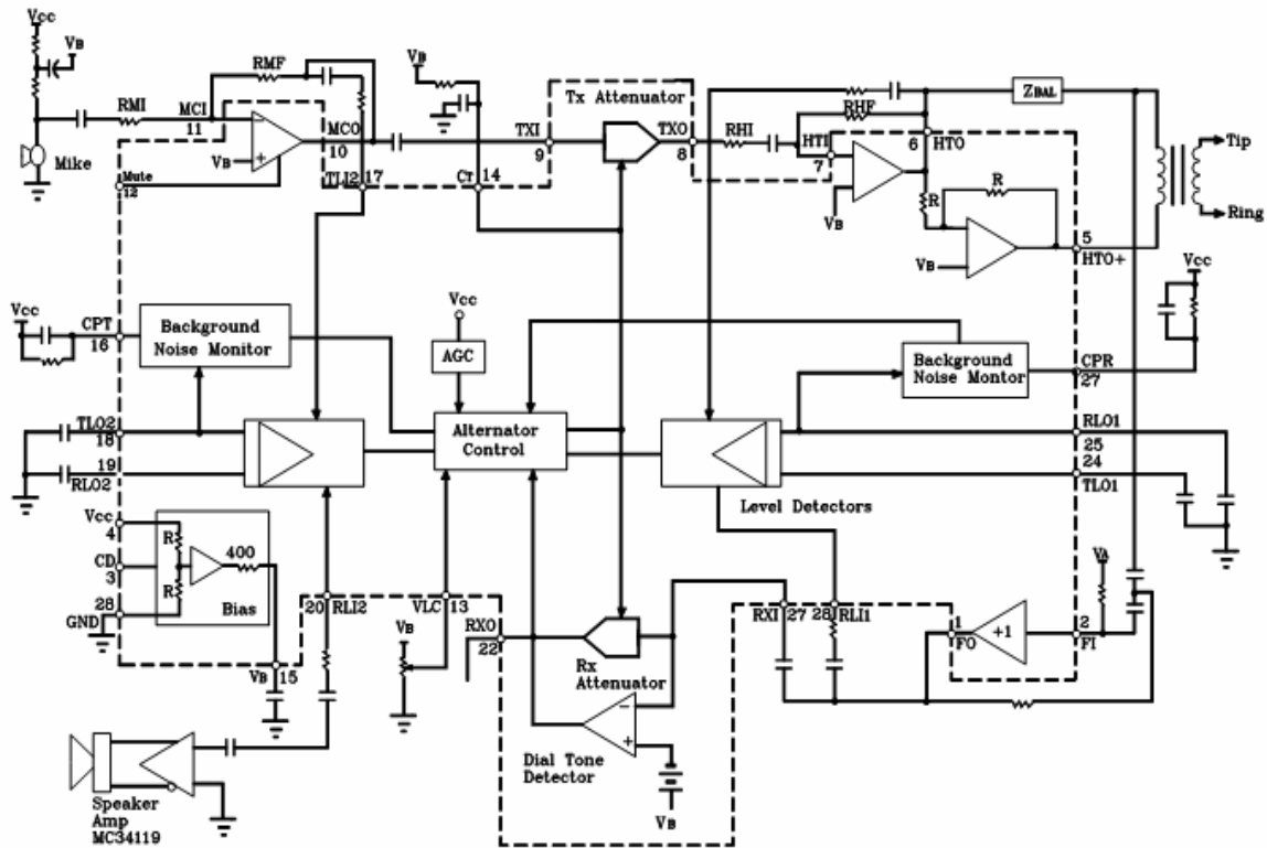
Figure 2. TS34118 Block Diagram
