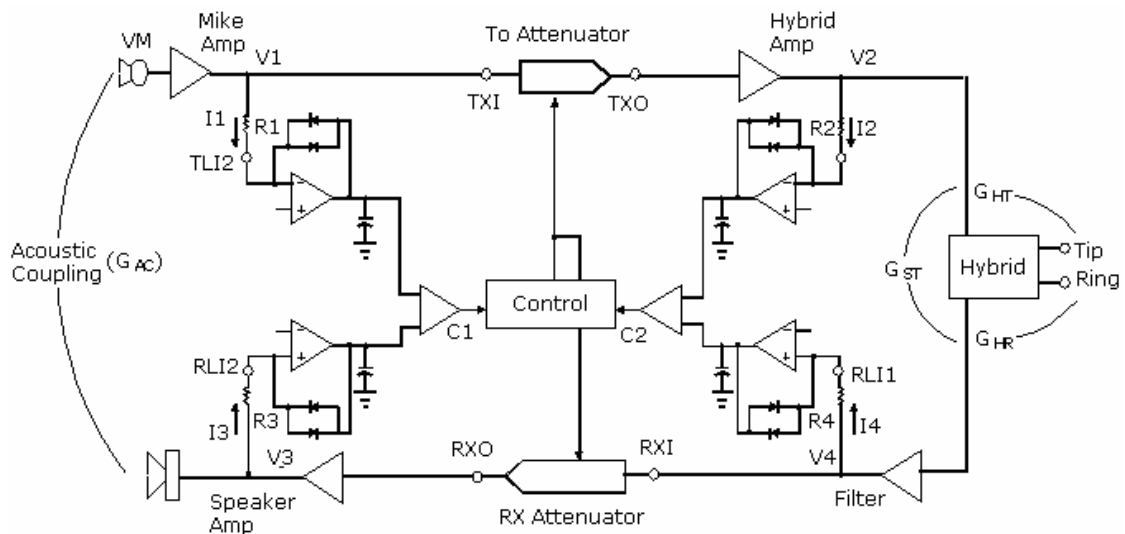
Figure 10. Basic Block Diagram For Design Purpos
