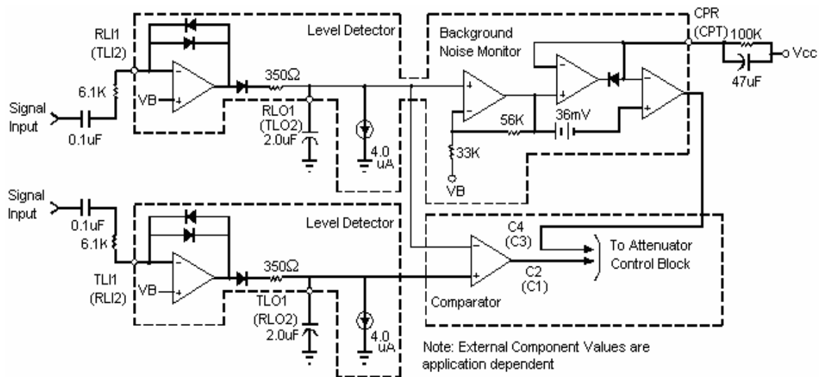
Figure 4. Level Detectors
