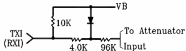
Figure 3. Attenuator Input Stage
