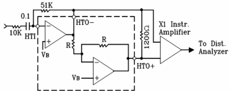
Figure 1. Hybrid Amplifier Distortion Test
